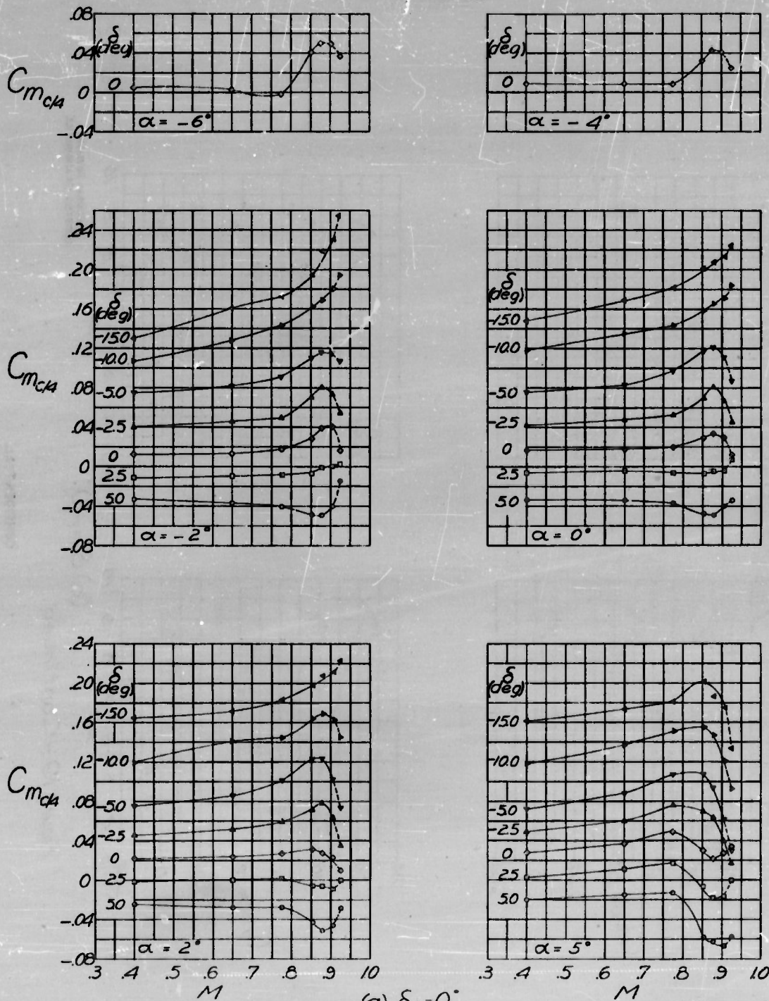
Figure 19.- Pitching-moment-coefficient data. (a) \delta_+ = 0^\circ .
