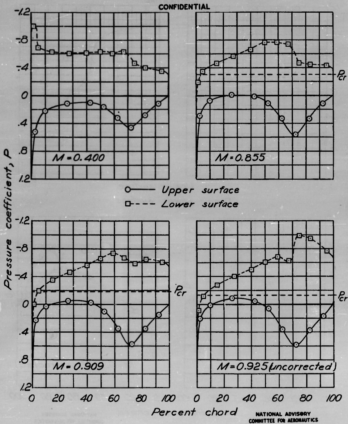
Figure 5.— Pressure distribution about the horizontal tail at the 40-percent-semispan station. \delta = -15^\circ ; \delta_t = 0^\circ .
