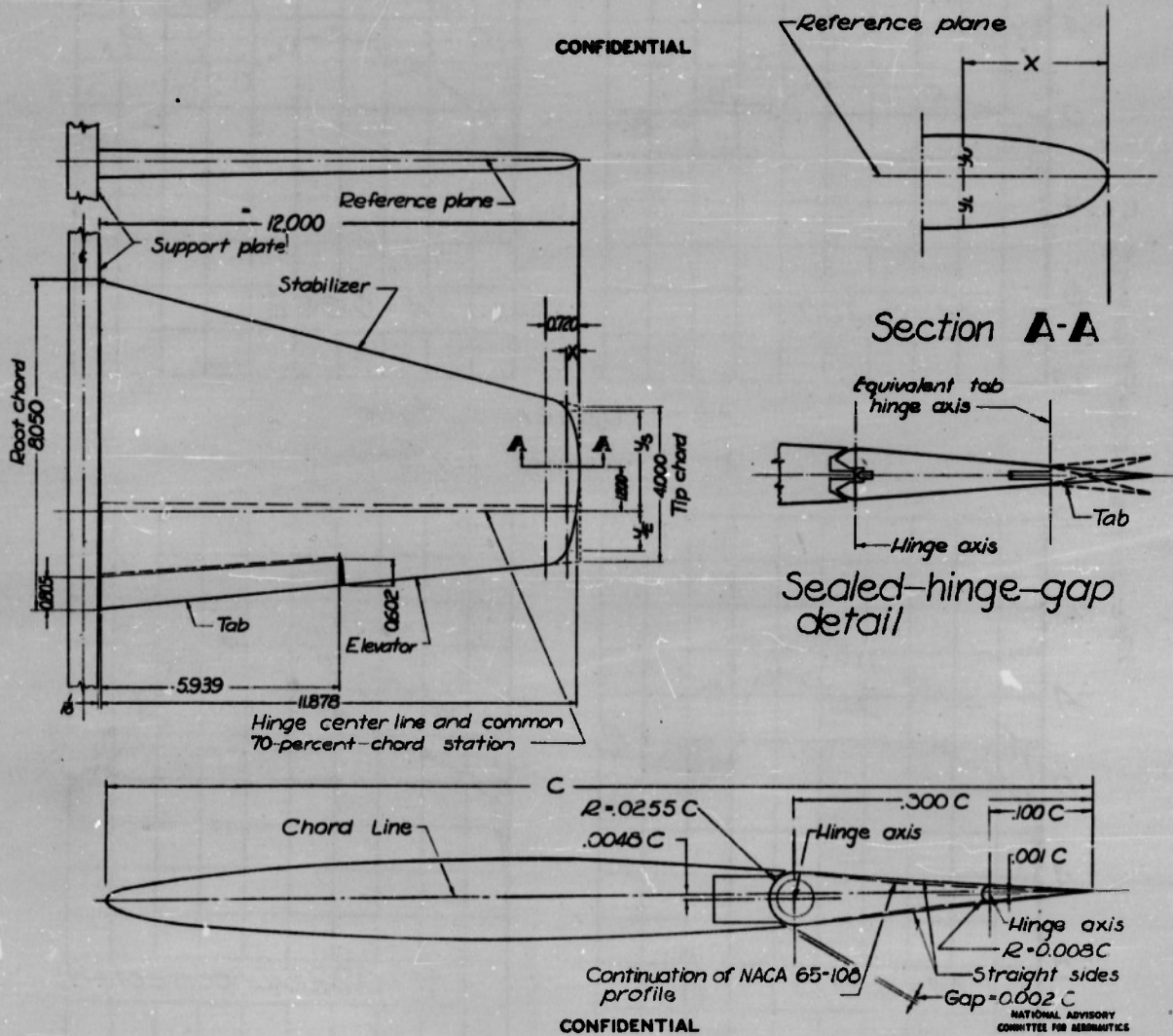
Figure 1.-Details of horizontal-tail model tested. (Dimensions in inches.)
