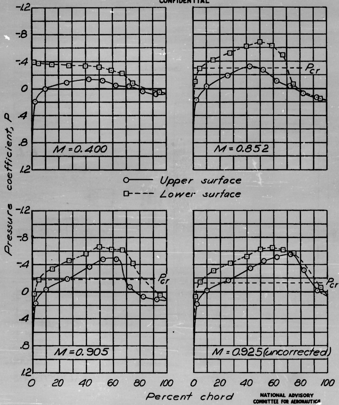
Figure 2. - Pressure distribution about the horizontal tail at the 40-percent-semispan station. \delta = 0^\circ ; \delta_T = 0^\circ .
