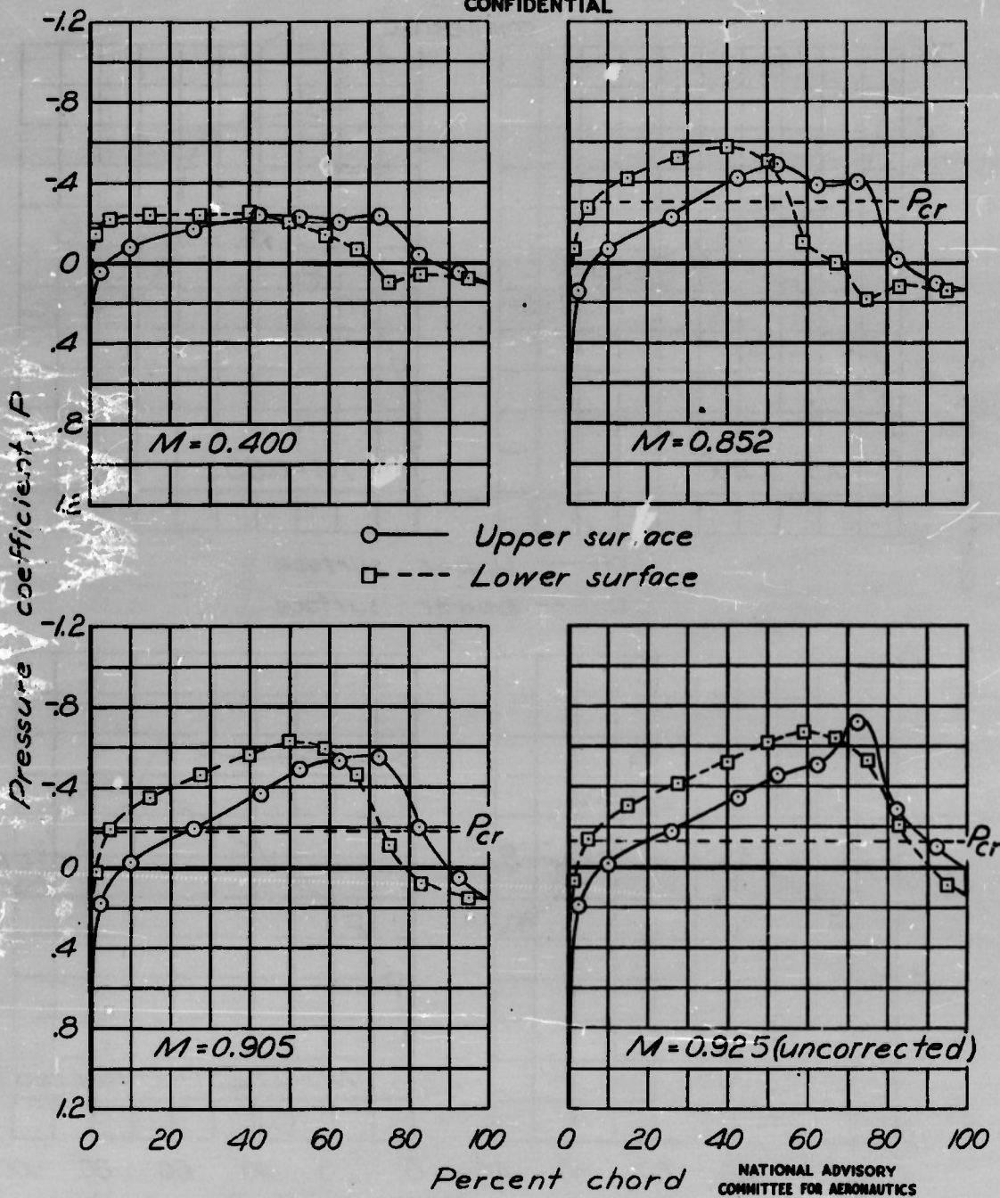
Figure 3. — Pressure distribution about the horizontal tail at the 40-percent-semispan station. \delta = 5^\circ ; \delta_T = 0^\circ .
