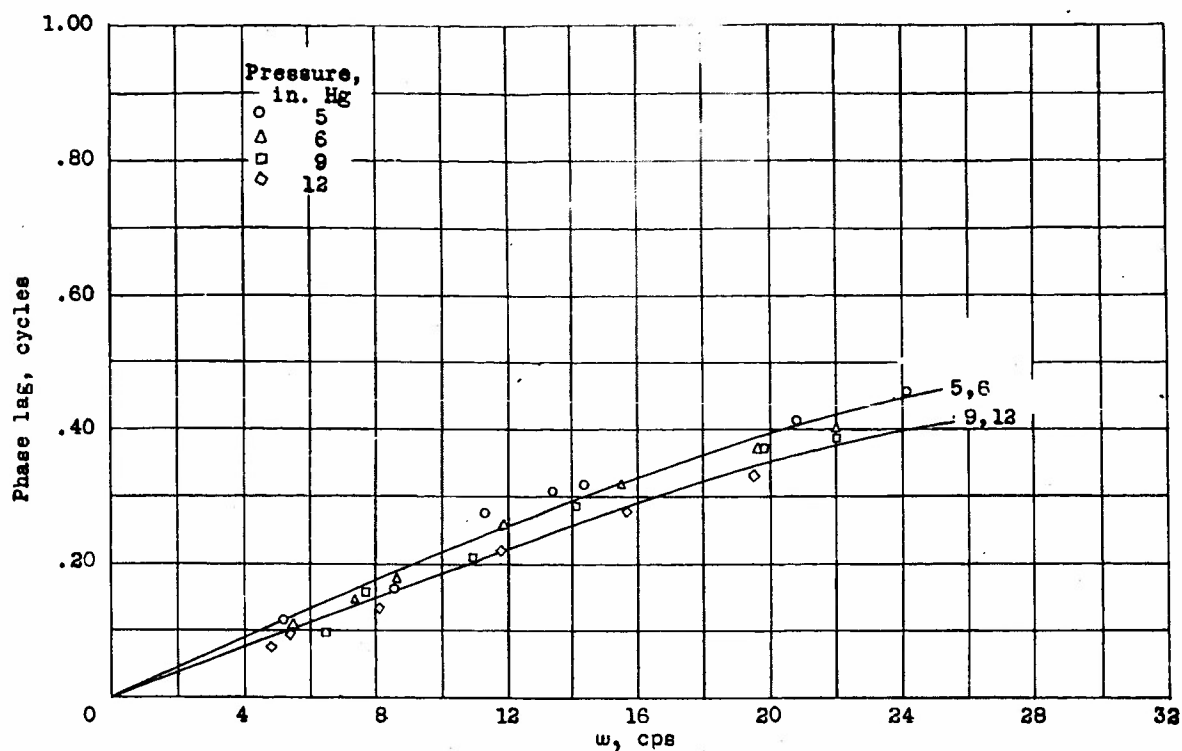
Figure 11.- Variation of phase lag with frequency at four pressures; stabilizer orifice line, airplane 1.
