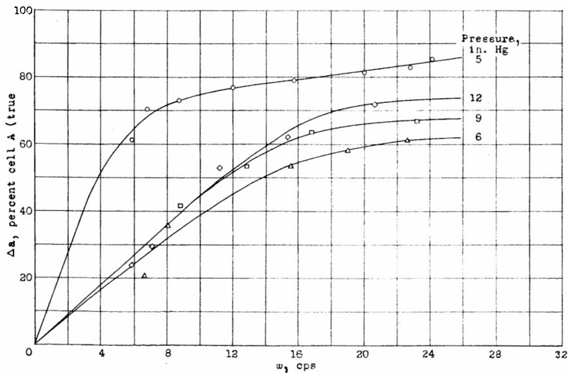
Figure 22.- Variation of amplitude error with frequency at four pressures; static-head line airspeed system, airplane 2.
