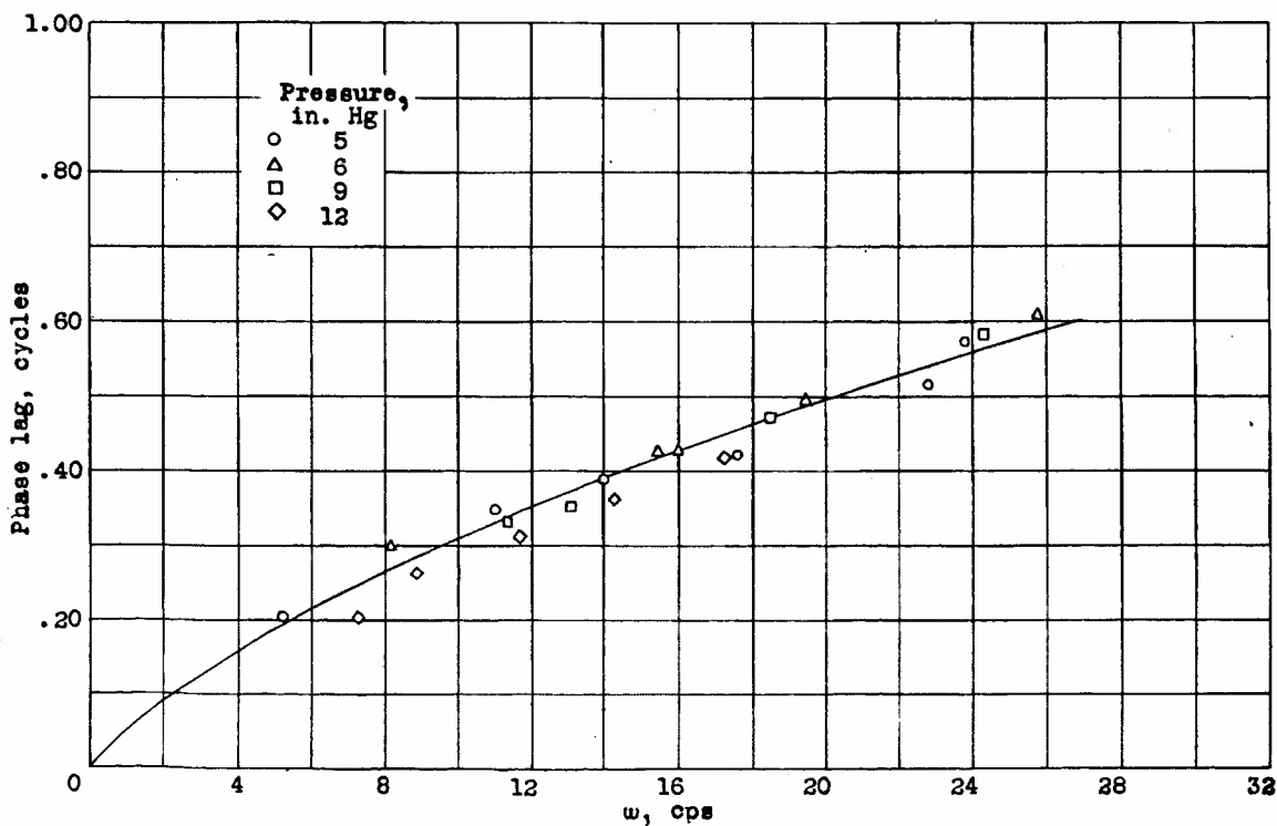
Figure 10.- Variation of phase lag with frequency at four pressures; aileron orifice line, airplane 1.
