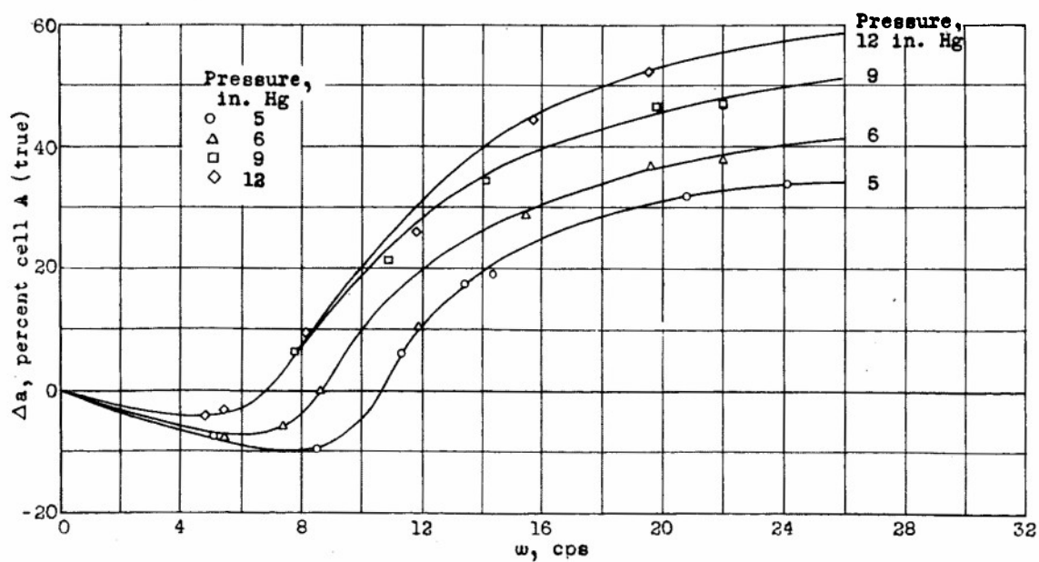
Figure 20.— Variation of amplitude error with frequency at four pressures; stabilizer orifice line, airplane 1.
