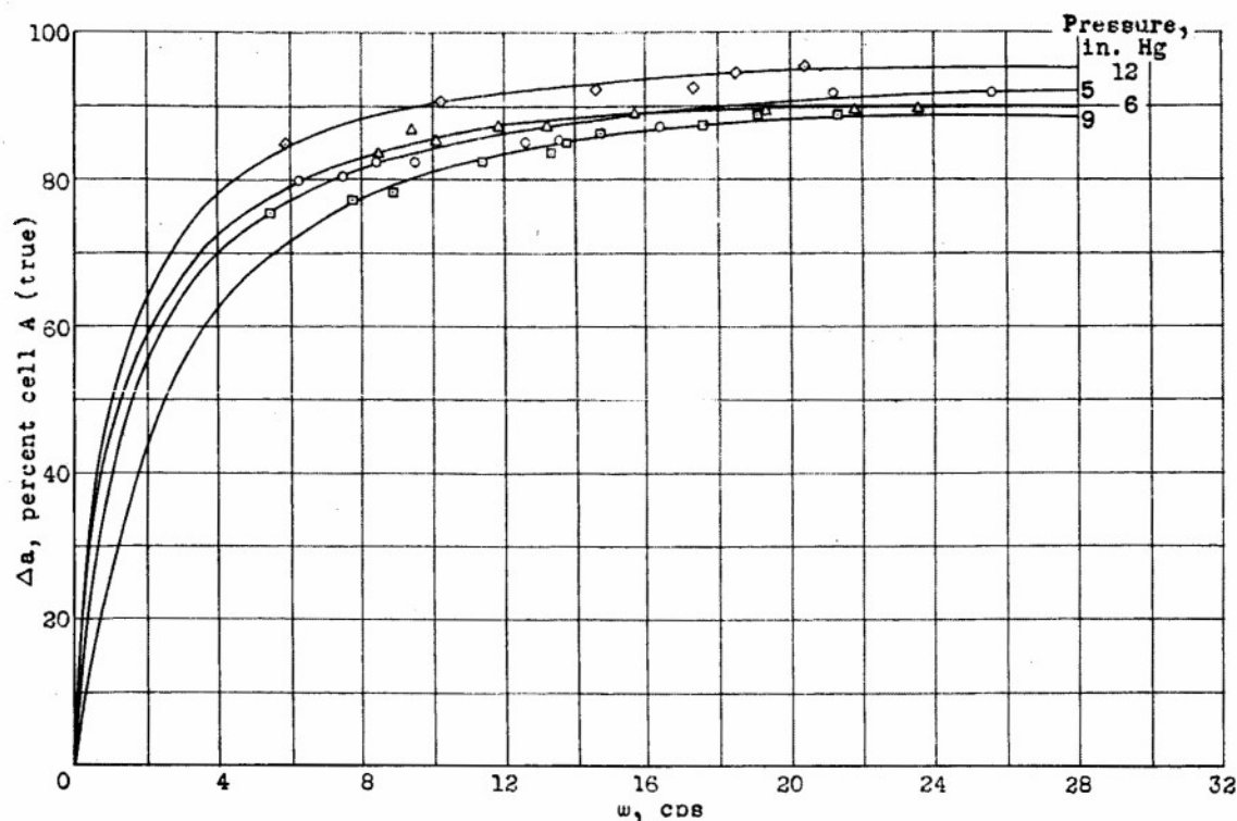
Figure 21.- Variation of amplitude error with frequency at four pressures; total-head line airspeed system, airplane 2.
