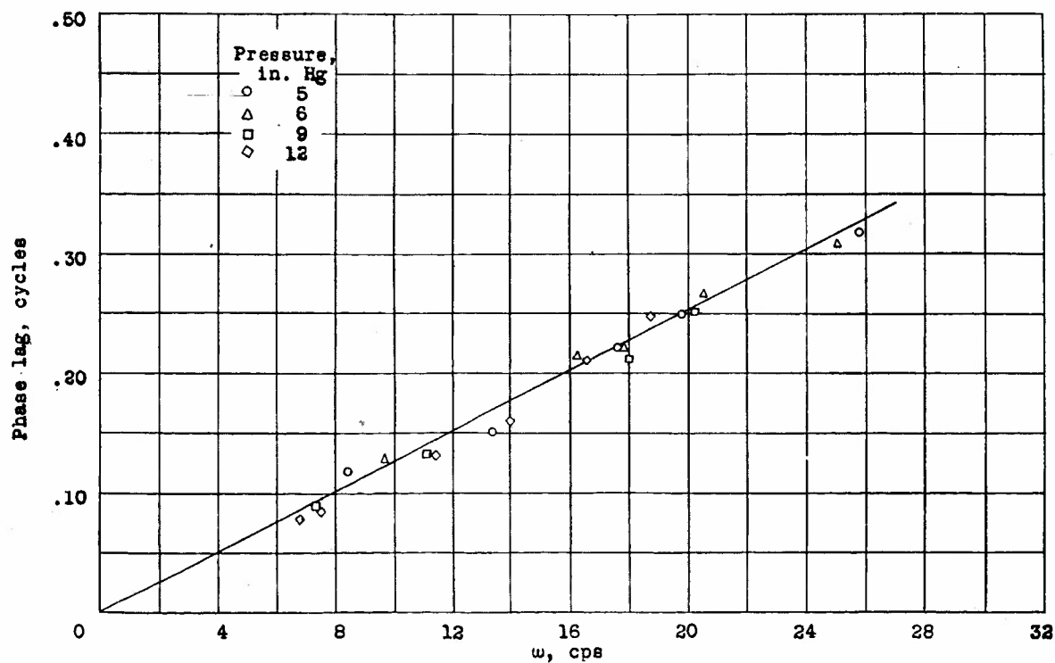
Figure 12.- Variation of phase lag with frequency at four pressures; wing orifice line, airplane 1.
