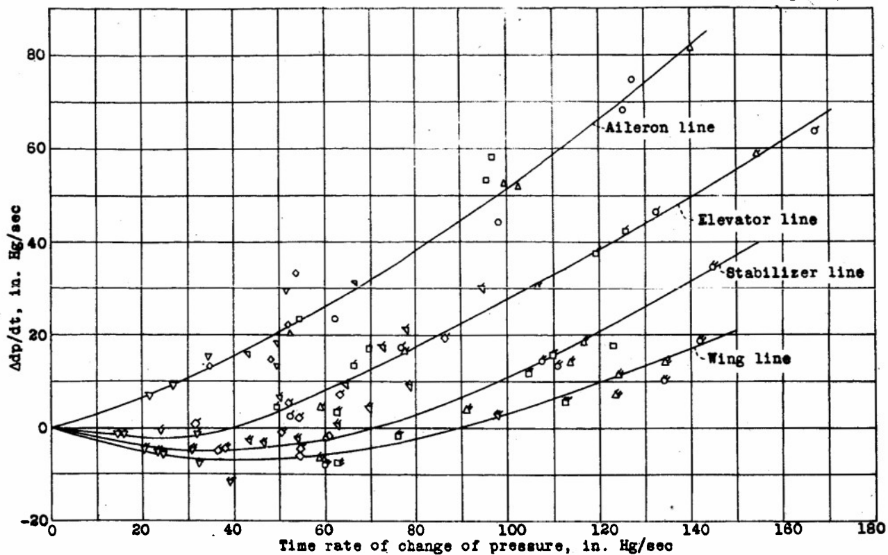
Figure 4.- The lag in pressure in typical pressure recorder lines, airplane 1.
