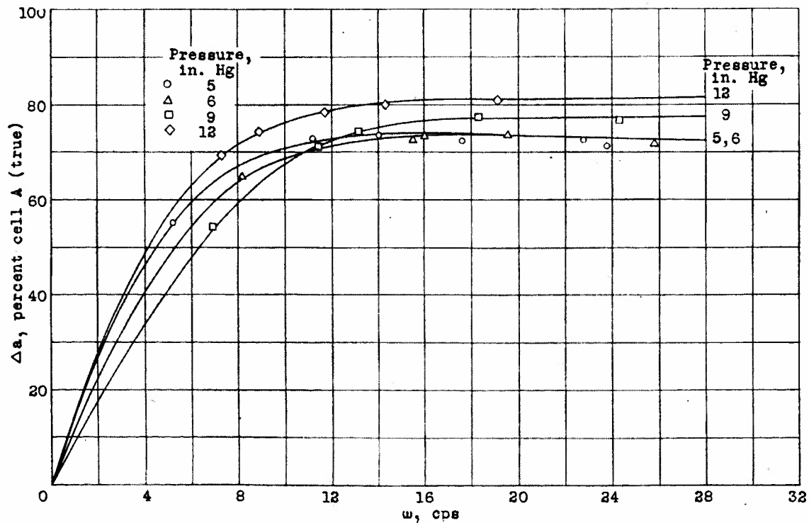
Figure 18.- Variation of amplitude error with frequency at four pressures; aileron orifice line, airplane 1.
