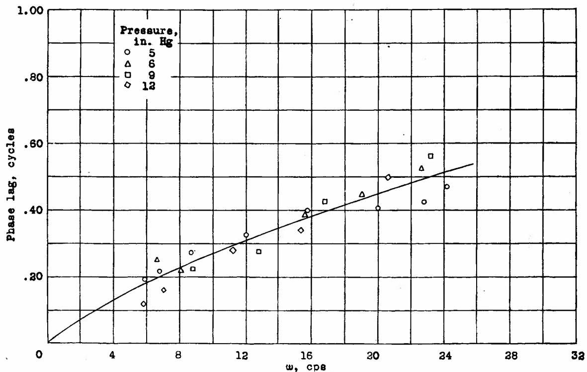
Figure 14.- Variation of phase lag with frequency at four pressures; static-head line airspeed system, airplane 2.
