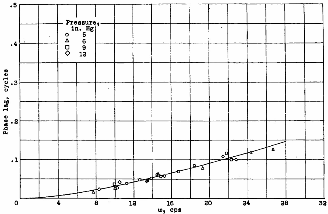
Figure 7.- Variation of phase lag with frequency at four pressures; total-head line airspeed system, airplane 1.
