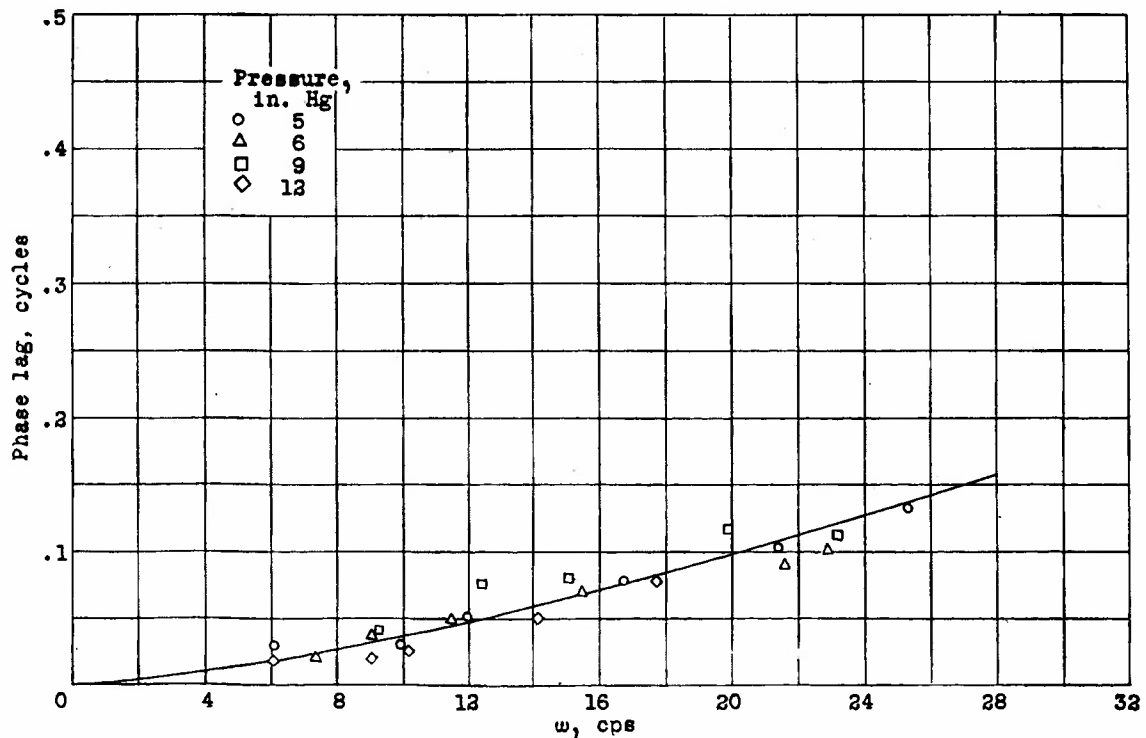
Figure 8.- Variation of phase lag with frequency at four pressures; static-head line airspeed system, airplane 1.
