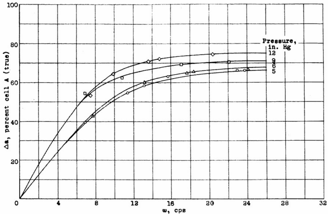
Figure 17.- Variation of amplitude error with frequency at four pressures; elevator orifice line, airplane 1.
