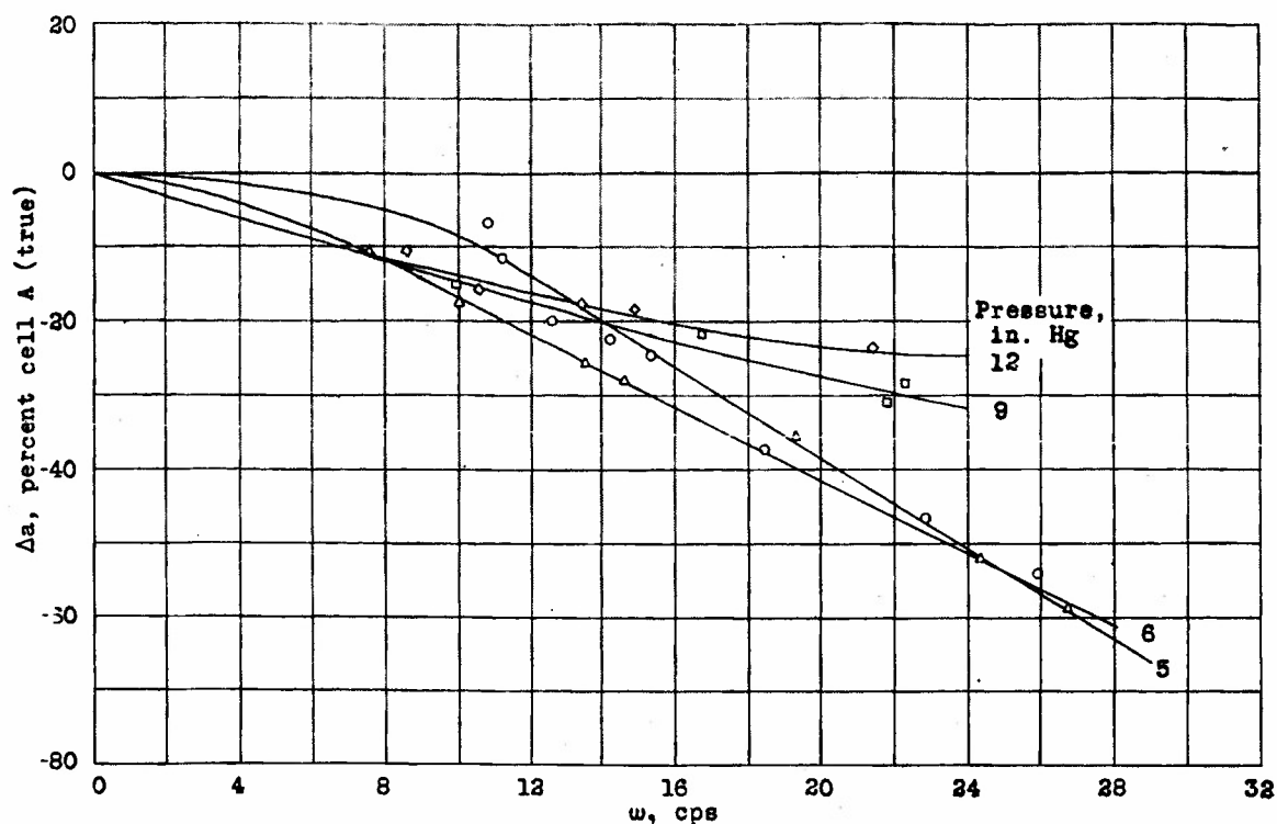
Figure 15.- Variation of amplitude error with frequency at four pressures; total-head line airspeed system, airplane 1.
