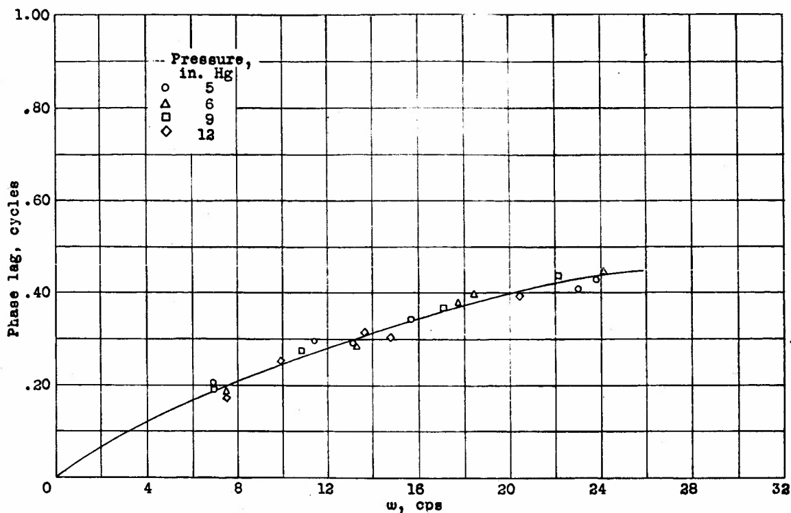
Figure 9.- Variation of phase lag with frequency at four pressures; elevator orifice line, airplane 1.
