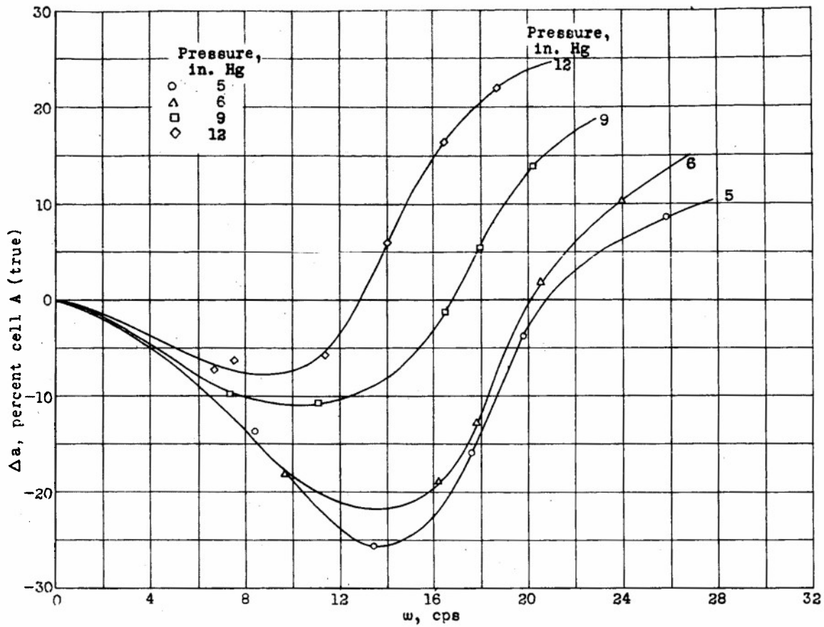
Figure 19.— Variation of amplitude error with frequency at four pressures; wing orifice line, airplane 1.
