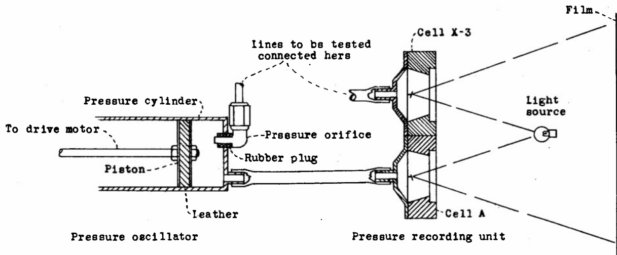
Figure 2.- Schematic diagram of equipment used to study effects of pressure oscillations on the indications of aircraft pressure-recording installations.
