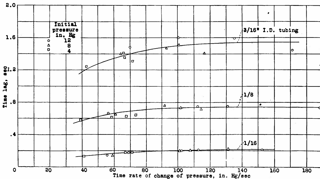
Figure 6.- Variation of pressure lag with tubing diameter for single-direction pressure changes through an .040 inch orifice.
