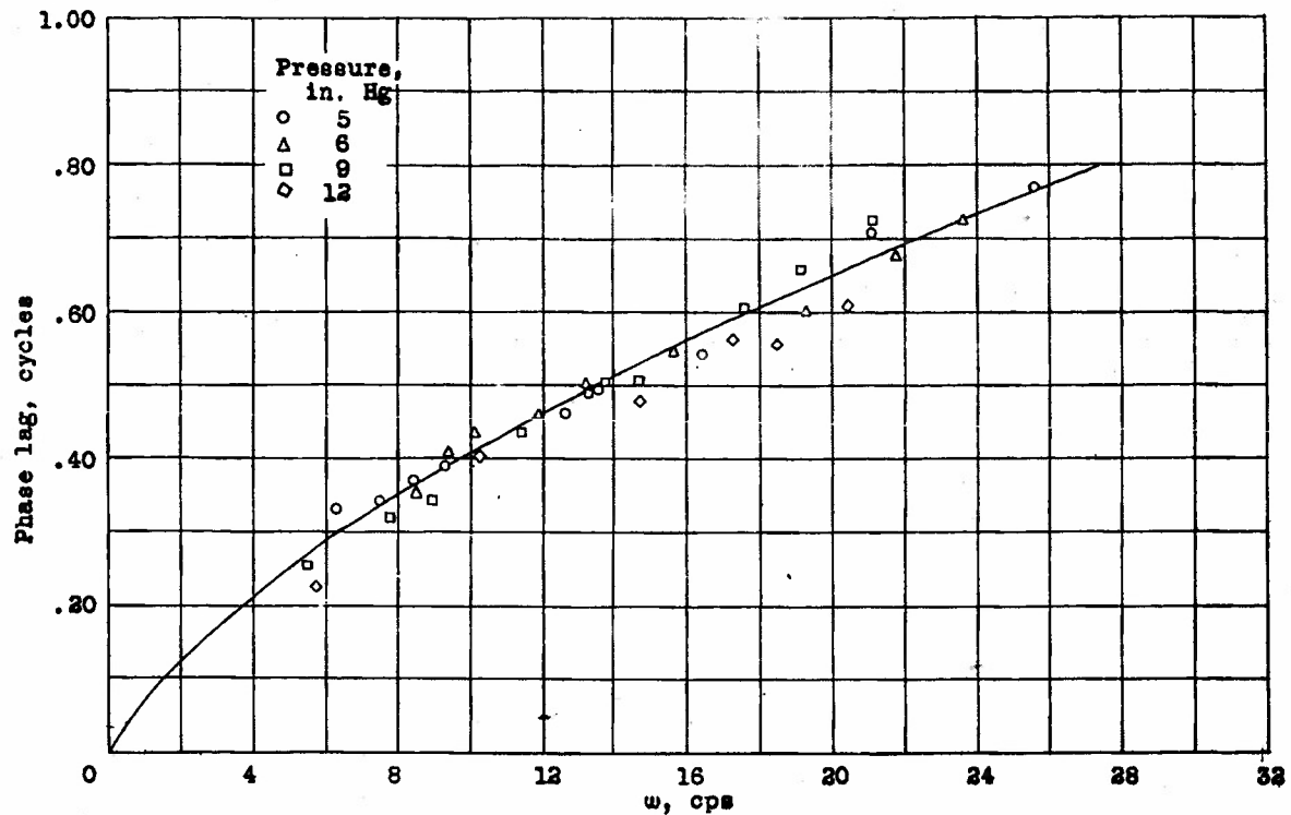
Figure 13.- Phase lag variation with frequency at four different pressures; total-head line airspeed system, airplane 2.
