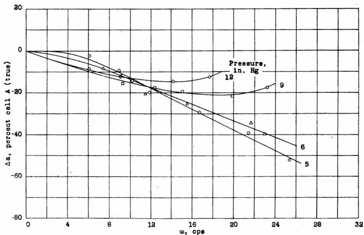
Figure 16.- Variation of amplitude error with frequency at four pressures; static-head line airspeed system, airplane 1.
