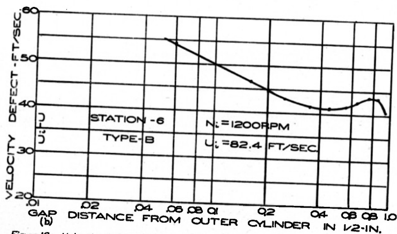
Figure 10.- Velocity defect between cylinders. N_1 , 1200 rpm; U_1 , 82.4 fps.
