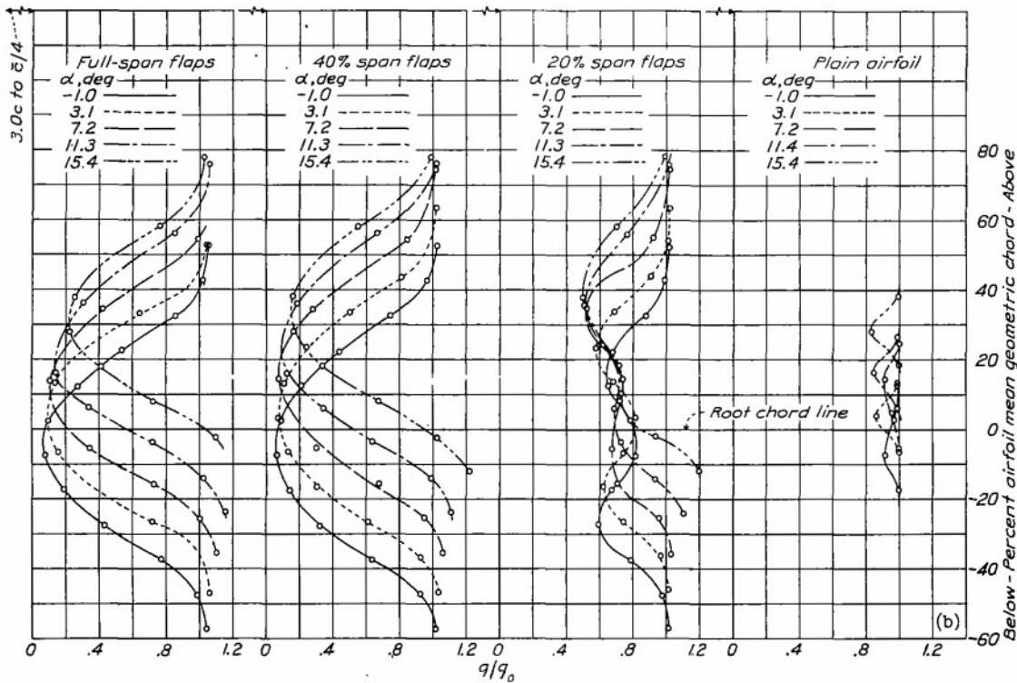
(b) Wake characteristics. Figure 3 (b).- Effect of 0.20c partial-span center-section perforated double split flaps located 0.20c from the airfoil trailing edge of a 60-inch span 3:1 tapered NACA 23012 airfoil. \delta f_U, 60^\circ ; \delta f_L, 60^\circ .
