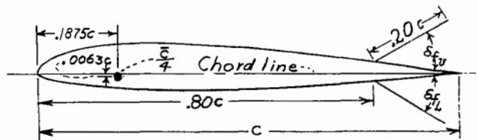
Section on mean geometric chord
