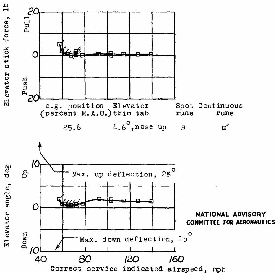
(b) Airplane with original tab on elevator locked. Figure 12.- Concluded.
