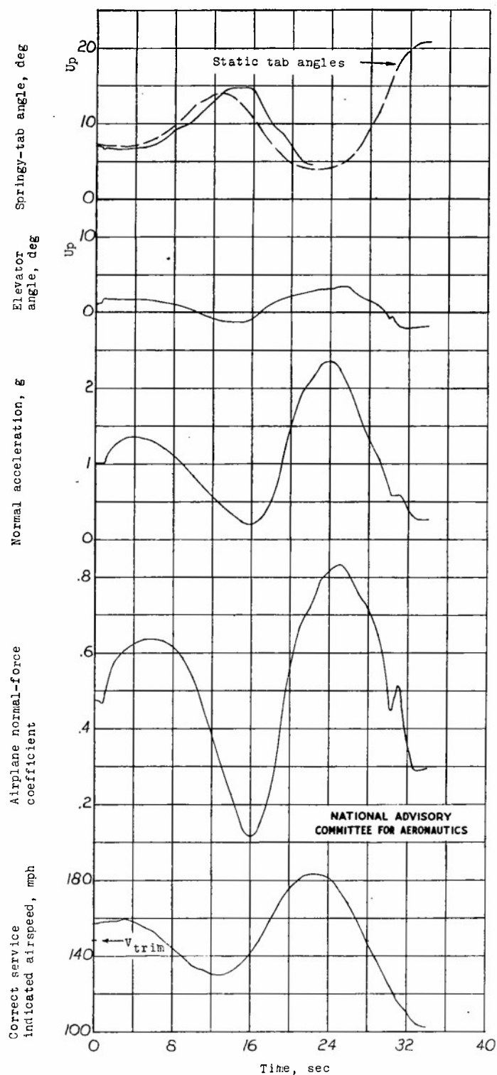
(b) Gliding condition; center of gravity at 30.2 percent mean aerodynamic chord; springy tab installed on elevator. Figure 14.- Concluded.
