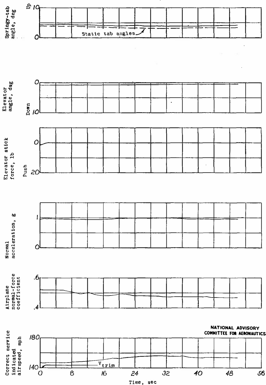
(a) Climbing condition; center of gravity at 30.3 percent mean aerodynamic chord; springy tab installed on elevator. Figure 14.- Time history of motion following stick release at speed slightly above trim.
