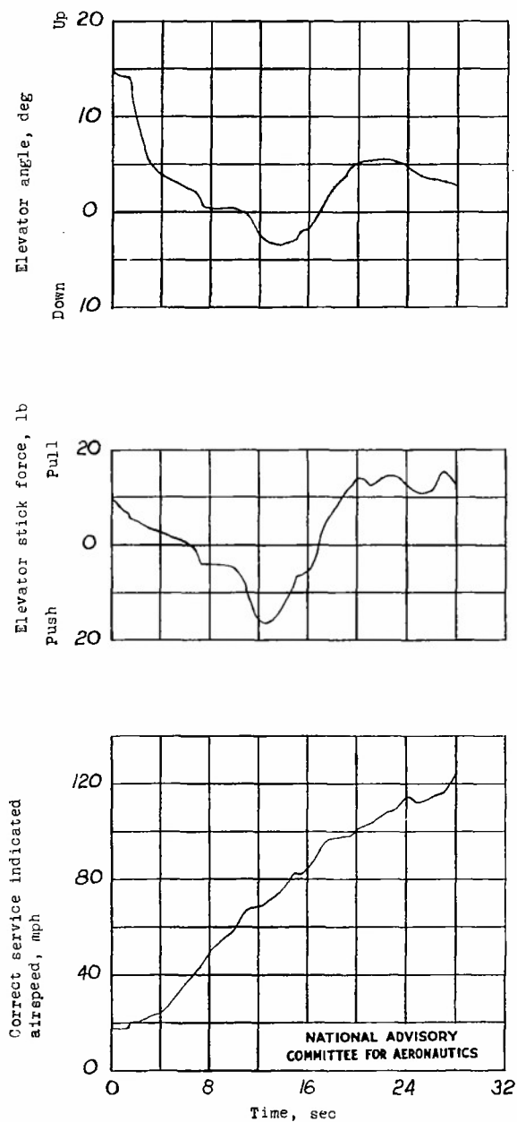
(b) Center of gravity at 27.2 percent mean aerodynamic chord; elevator-trim-tab setting, 0^\circ ; airplane with original tab on elevator locked. Figure 17.- Continued.
