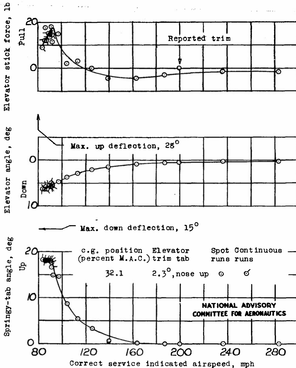
Figure 19.- Static longitudinal stability characteristics in the climbing condition with the initial springy-tab configuration.
