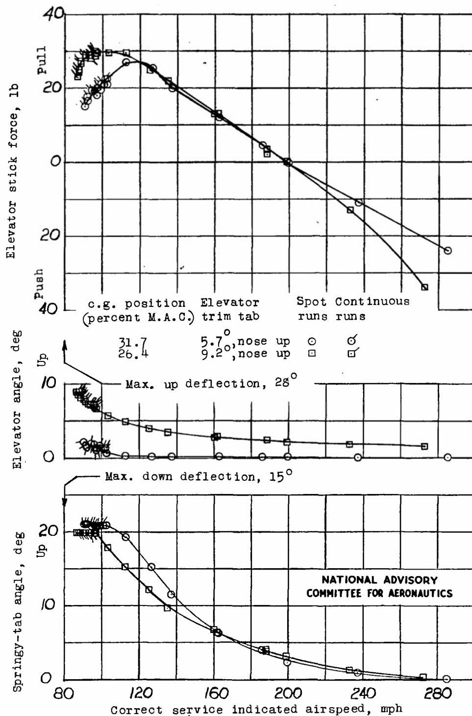
(a) Airplane with springy tab installed on elevator. Figure 10.- Static longitudinal stability characteristics in the gliding condition.
