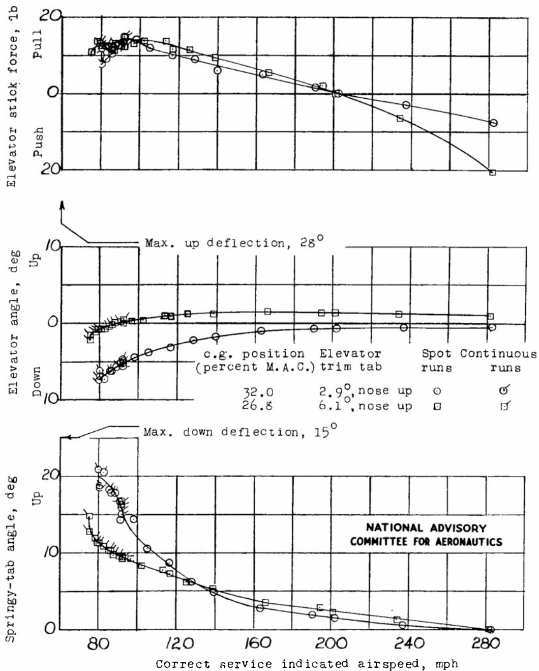
(a) Airplane with springy tab installed on elevator. Figure 9.- Static longitudinal stability characteristics in the climbing condition.
