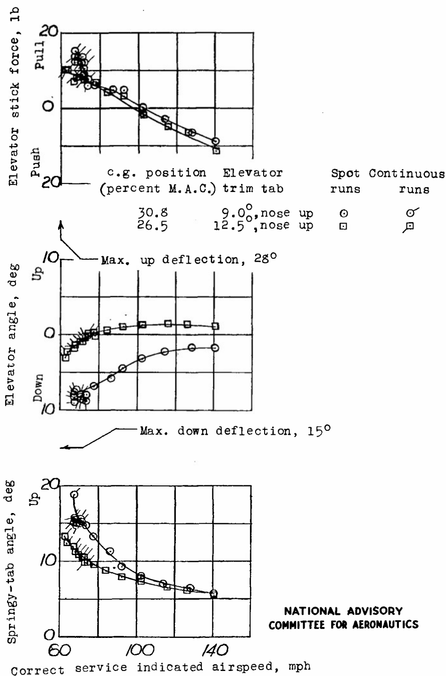
(a) Airplane with springy tab installed on elevator. Figure 12.- Static longitudinal stability characteristics in the wave-off condition.
