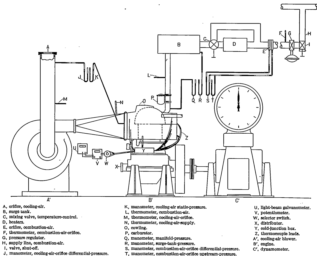
FIGURE 5.—Diagrammatic layout of equipment.
