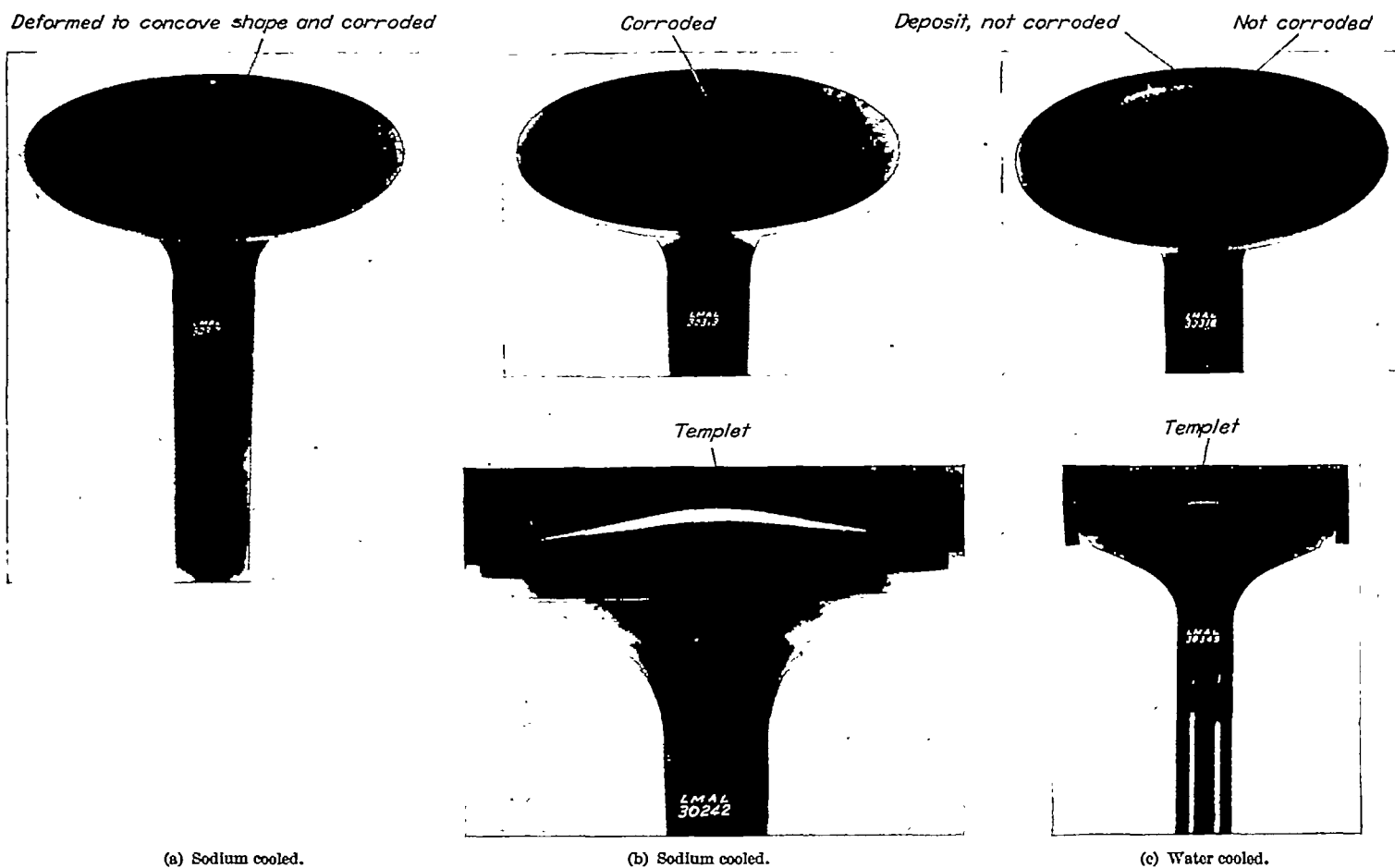
FIGURE 1.—Deformation and corrosion of exhaust valves cooled by sodium and by circulating water.
