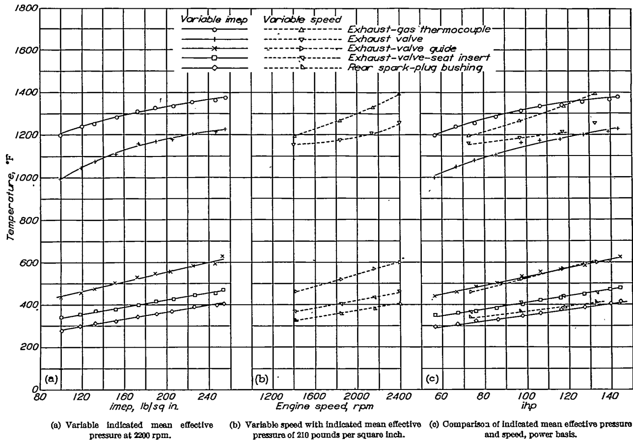
FIGURE 7.—Influence of engine power on the temperature of the exhaust valve and associated parts in an air-cooled cylinder. Fuel-air ratio, 0.08; spark advance, 19° B. T. O.; cooling-air pressure drop, 16 inches of water; cooling-air temperature, 88° F.
