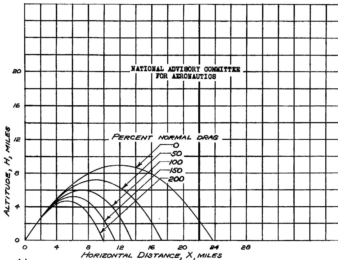
FIGURE 9.- CALCULATED TRAJECTORIES FOR THE MISSILE WITH SEVERAL ASSUMED VARIATIONS OF THE DRAG COEFFICIENT WITH MACH NUMBER, \beta = 11.12 , \theta_0 = 60^\circ
