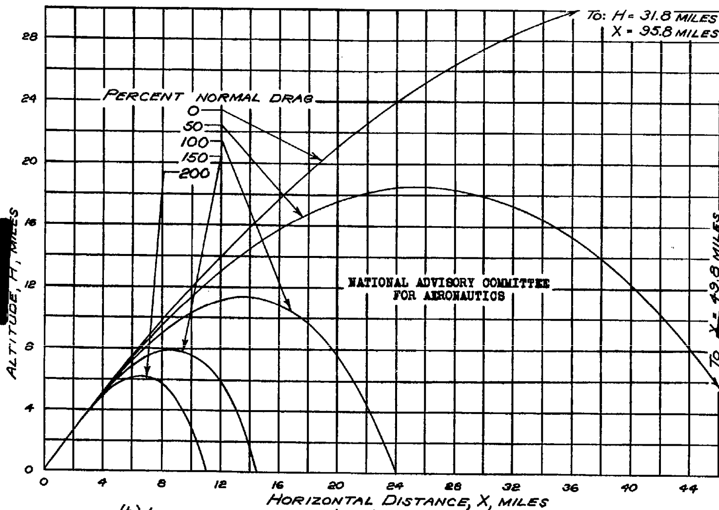
(b) LIQUID FUEL POWER, \lambda = 1.86 FIGURE 3.- CONCLUDED.
