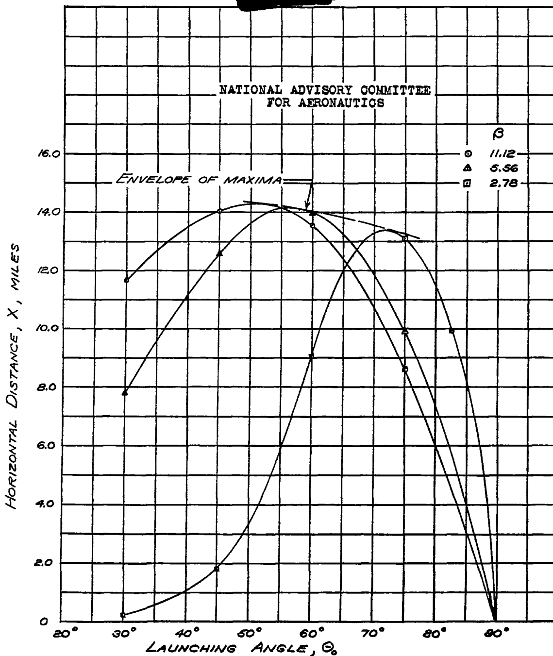
(a) \lambda = 1.53 . FIGURE 19.- VARIATION OF RANGE WITH LAUNCHING ANGLE FOR SOLID-FUEL-POWERED MISSILE WITH THREE VALUES OF INITIAL THRUST RATIO.
