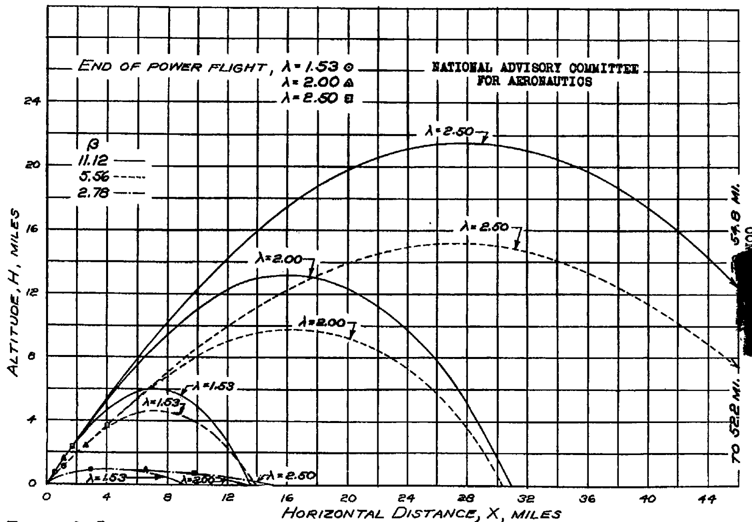
FIGURE 18.—COMPARISON OF TRAJECTORIES FOR SOLID-FUEL ROCKET POWERED MISSILE WITH THREE WEIGHT RATIOS AND THREE INITIAL THRUST RATIOS FOR A LAUNCHING ANGLE OF 60^\circ .
