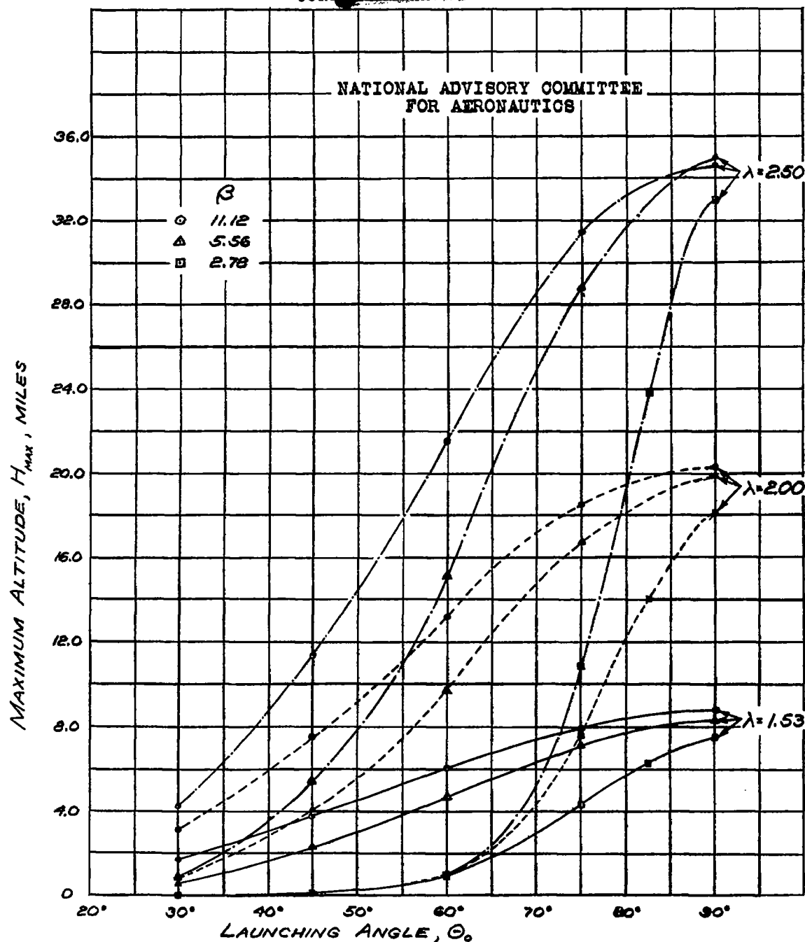
FIGURE 20.—VARIATION OF MAXIMUM ALTITUDE ATTAINED BY SOLID-FUEL-POWERED MISSILE WITH LAUNCHING ANGLE FOR THREE WEIGHT RATIOS AND THREE INITIAL THRUSTS
