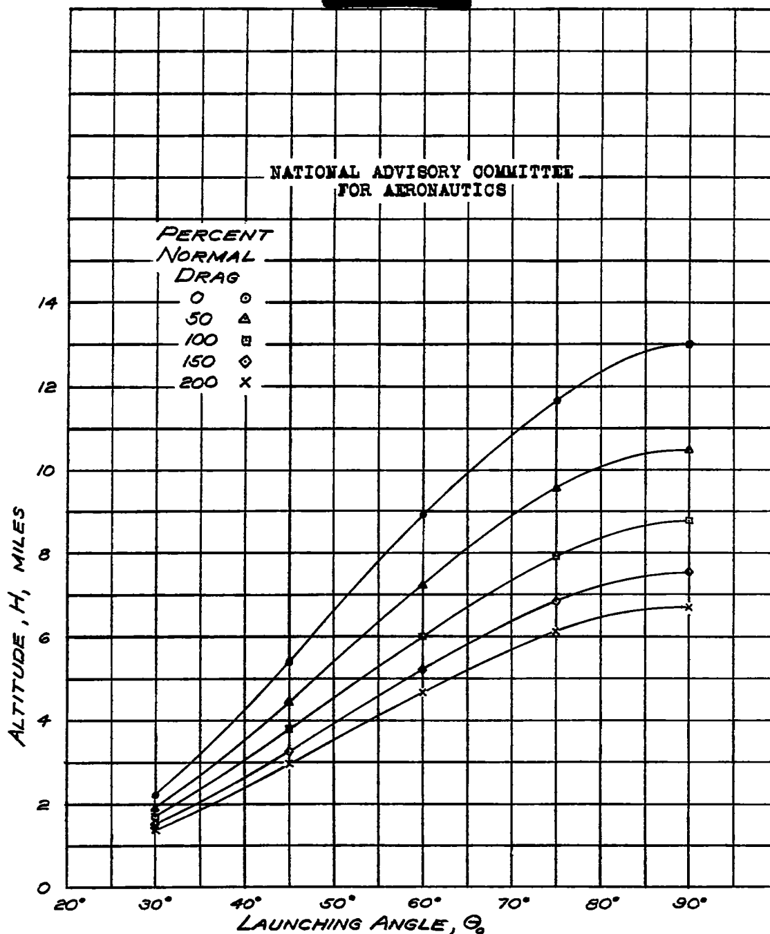
FIGURE 13.-VARIATION OF MAXIMUM ALTITUDE OF THE TRAJECTORY WITH LAUNCHING ANGLE FOR THE MISSILE WITH SOLID-FUEL ROCKET POWER AND SEVERAL ASSUMED VARIATIONS OF THE DRAG COEFFICIENT WITH MACH NUMBER. \beta=11.12
