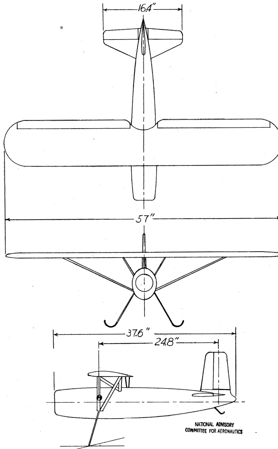
figure 1.- Three-view drawing of the modified \frac{1}{7} -scale model of the Fairchild XR2K-1 airplane.
