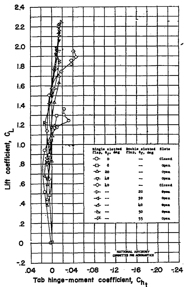
(e) Tab hinge-moment characteristics.
