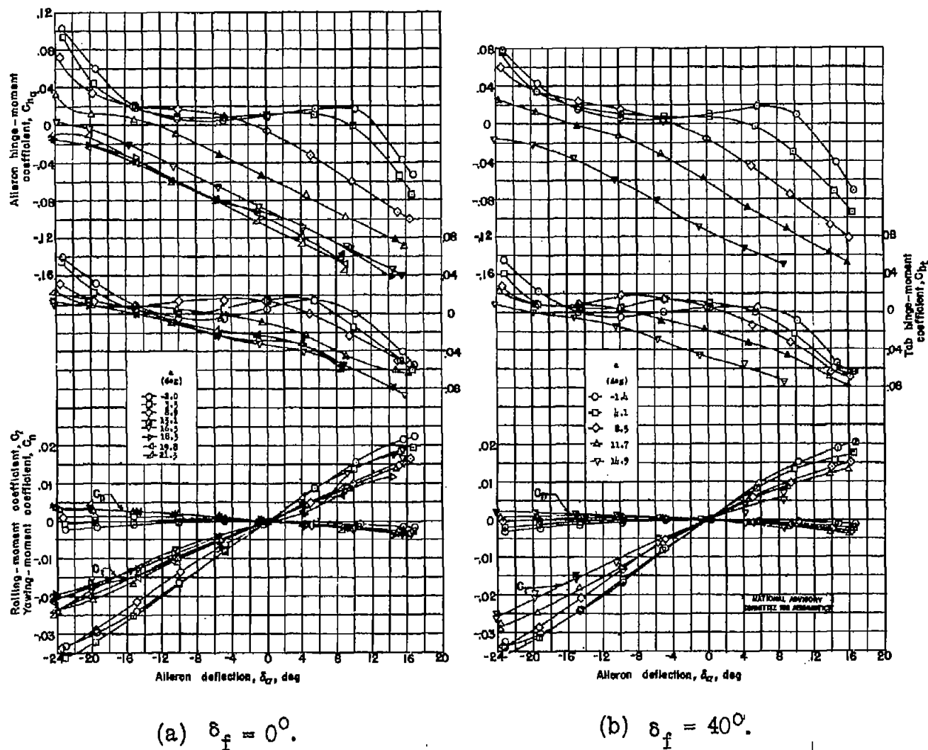
Figure 10.- Characteristics of the aileron with single slotted flaps for various angles of attack. Tabs neutral; slots closed; R \approx 8,800,000 ; M \approx 0.18 .
