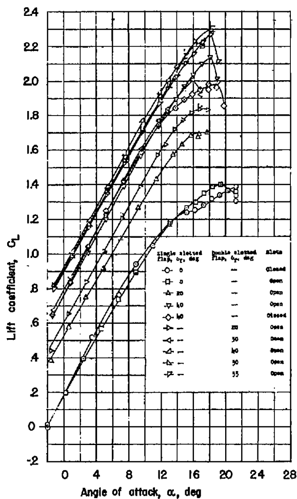
(a) Lift characteristics.
