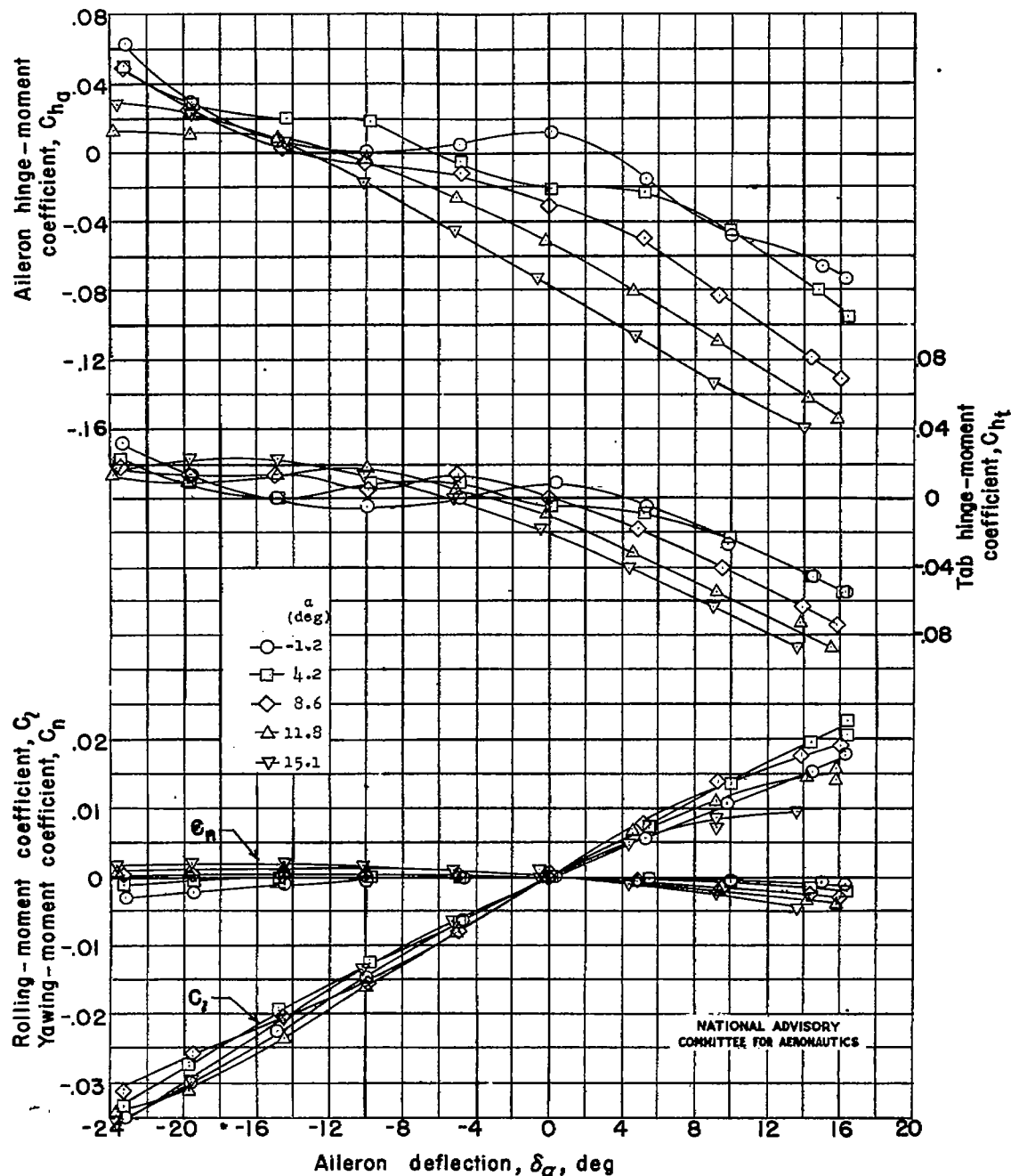
Figure 12.- Characteristics of the aileron and tab for various angles of attack. Double slotted flaps deflected 50^\circ ; slots open; R \approx 8,900,000 ; M \approx 0.18 .
