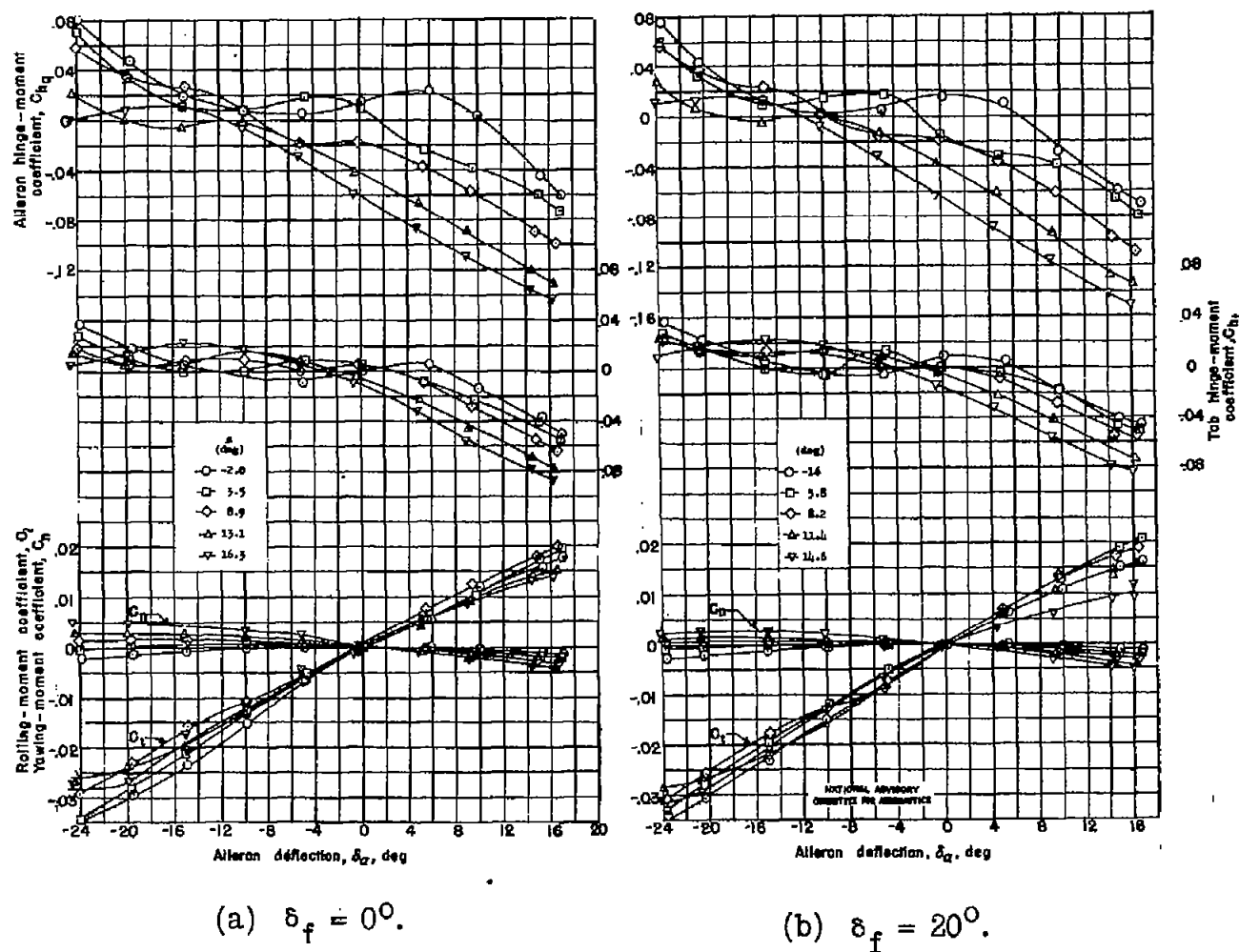
Figure 11.- Characteristics of the aileron with single slotted flaps for various angles of attack. Tabs neutral; slots open; R \approx 8,900,000 ; M \approx 0.18 .
