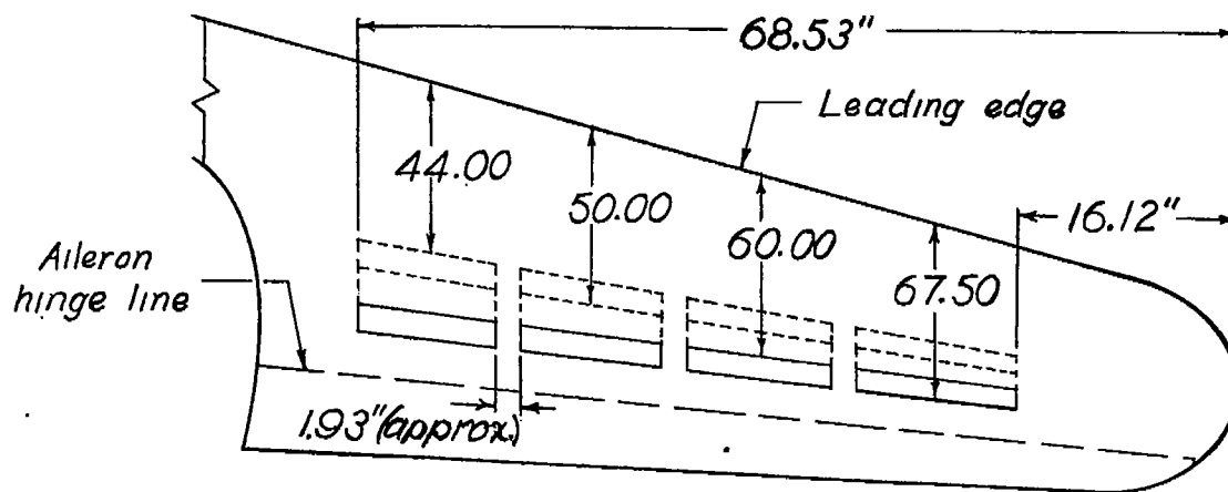
Figure 5.- Arrangement of the midchord slot of the partial-span wing model. (Dimensions in percent of wing section chord except as noted.)
