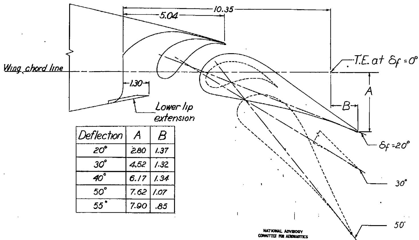
Figure 7.- Inboard double-slotted-flap positions at a typical section of the partial-span wing model. (All dimensions in inches.)
