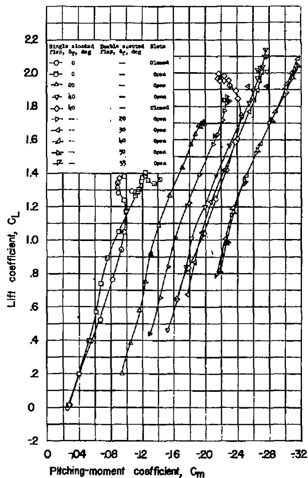
(c) Pitching-moment characteristics.
