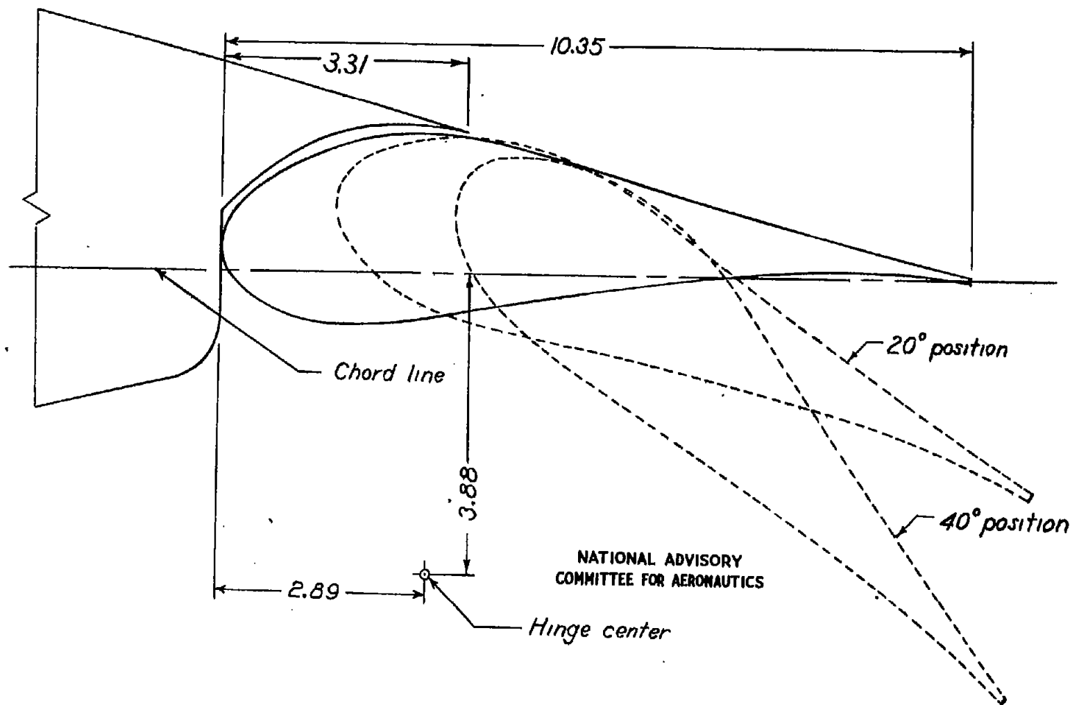
Figure 6.- Inboard single-slotted-flap positions at a typical section of the partial-span wing model. (All dimensions in inches.)
