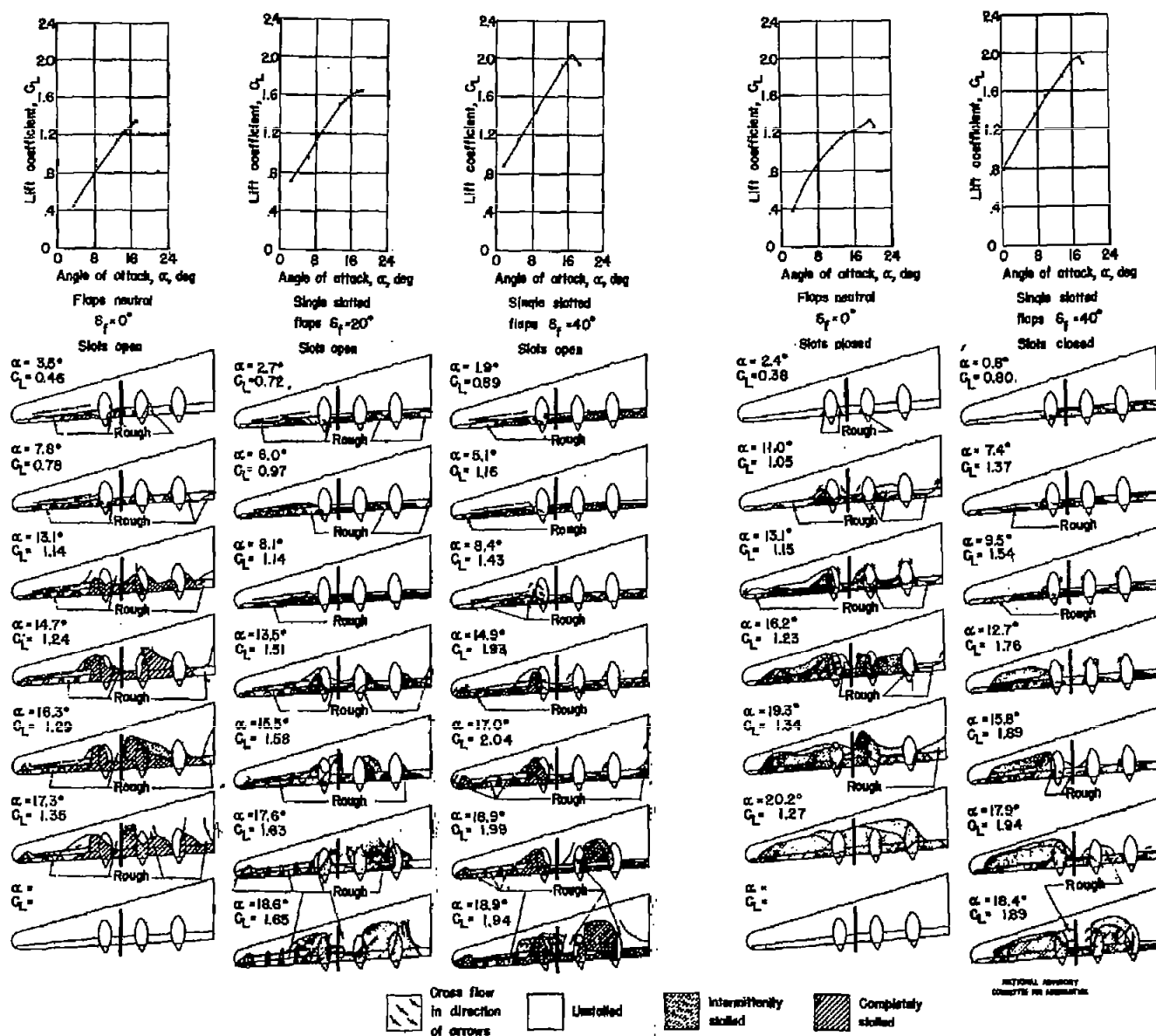
Figure 9.- Stall diagrams of the partial-span wing model with various flap and slot configurations. R \approx 8,900,000 ; M \approx 0.18 .
