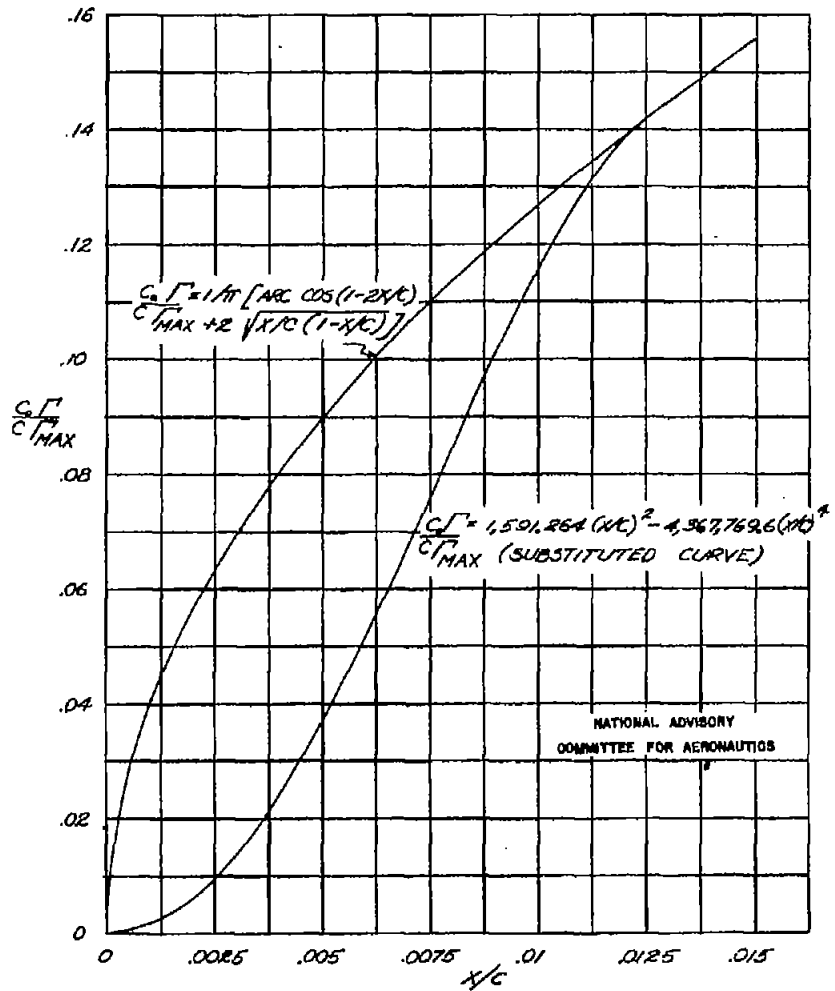
FIGURE 2.- A PORTION OF THE CHORDWISE CIRCULATION DISTRIBUTION NEAR THE LEADING EDGE AND THE FOURTH DEGREE CURVE THAT WAS SUBSTITUTED TO OBTAIN d\Gamma/d(x/c) = 0 AT x/c = 0 .
