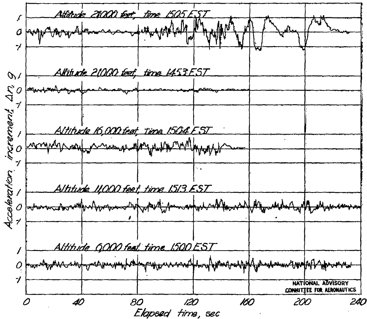
Figure 2.- Time histories of acceleration for traverses through a thundercloud on July 2, 1946.
