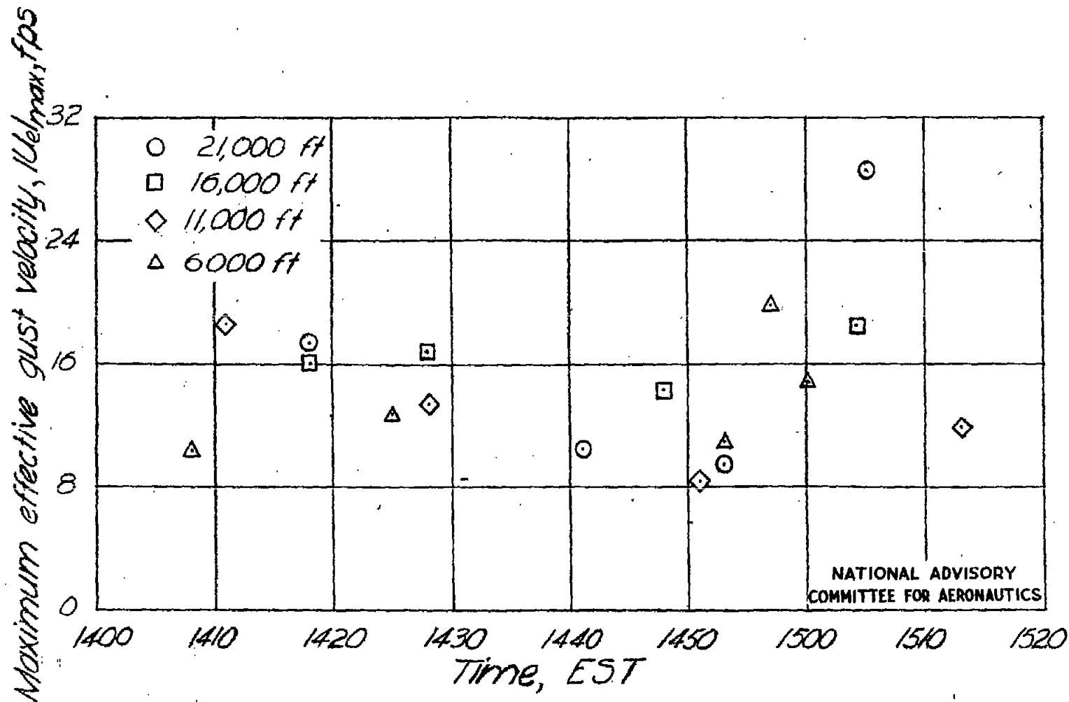
Figure 3.- Time variation of atmospheric turbulence measured within thunderclouds.
