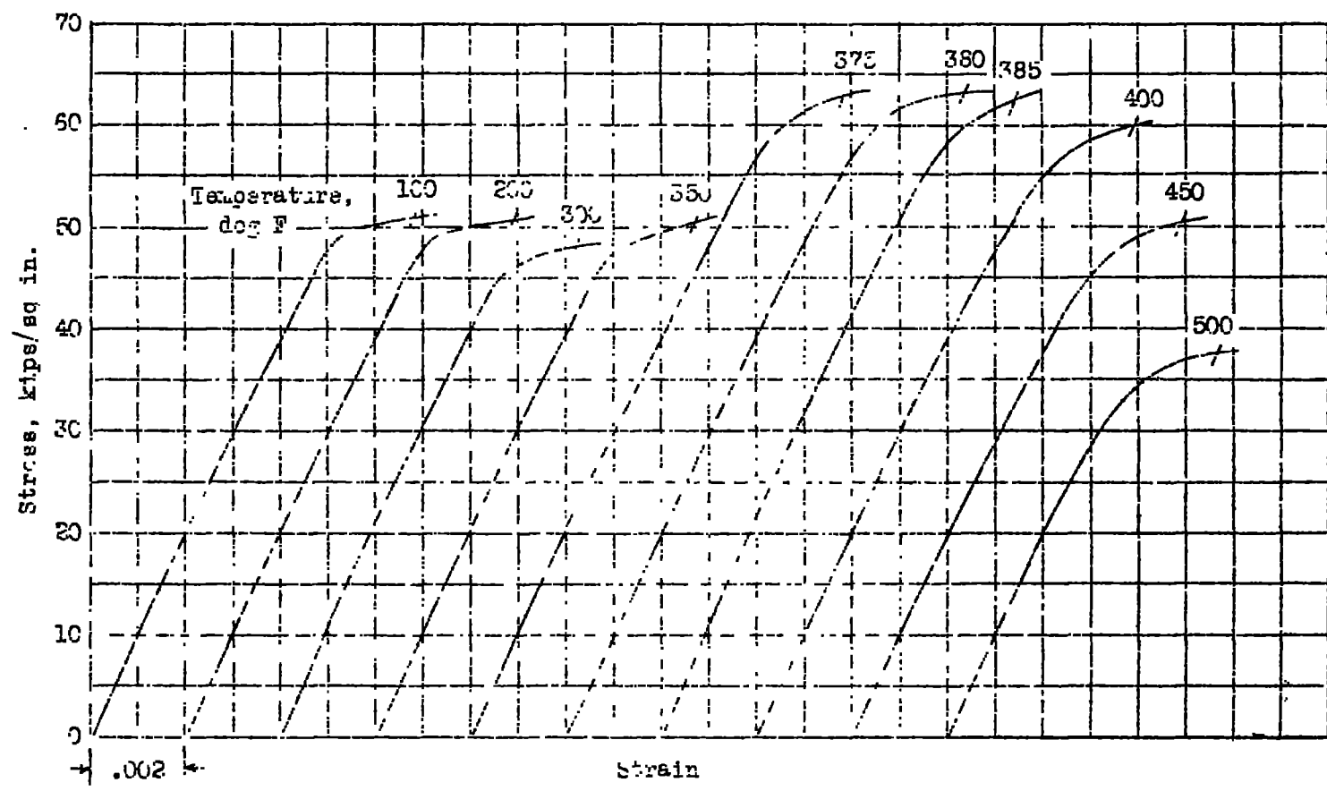
Figure 8.- Stress-strain curves for alloyed 2024-T3 aluminum alloy aged for four hours at various temperatures.
