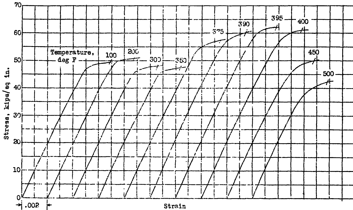
Figure 7.- Stress-strain curves for alclad 24S-T aluminum alloy aged for two hours at various temperatures.
