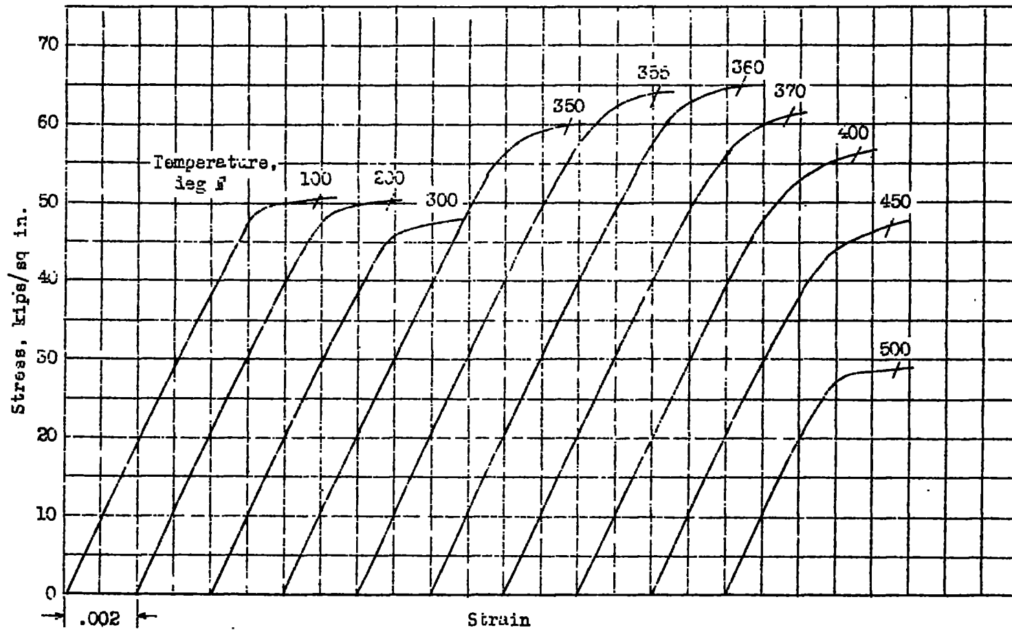
Figure 11.- Stress-strain curves for alclad 24S-T aluminum alloy aged for ten hours at various temperatures.
