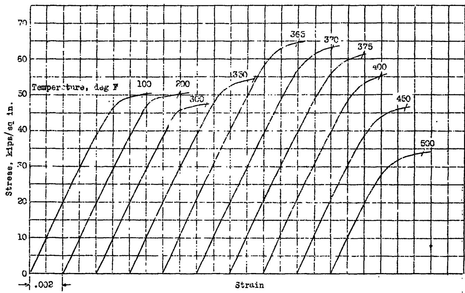
Figure 10.- Stress-strain curves for alclad 24S-T aluminum alloy aged for seven hours at various temperatures.
