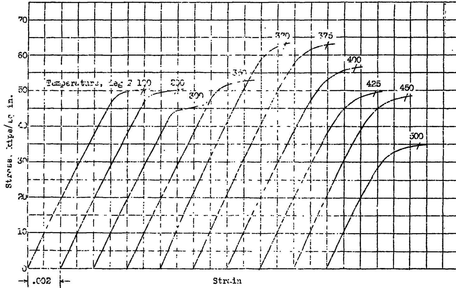
Figure 9.- Stress-strain curves for clad 24S-T aluminum alloy aged for six hours at various temperatures.
