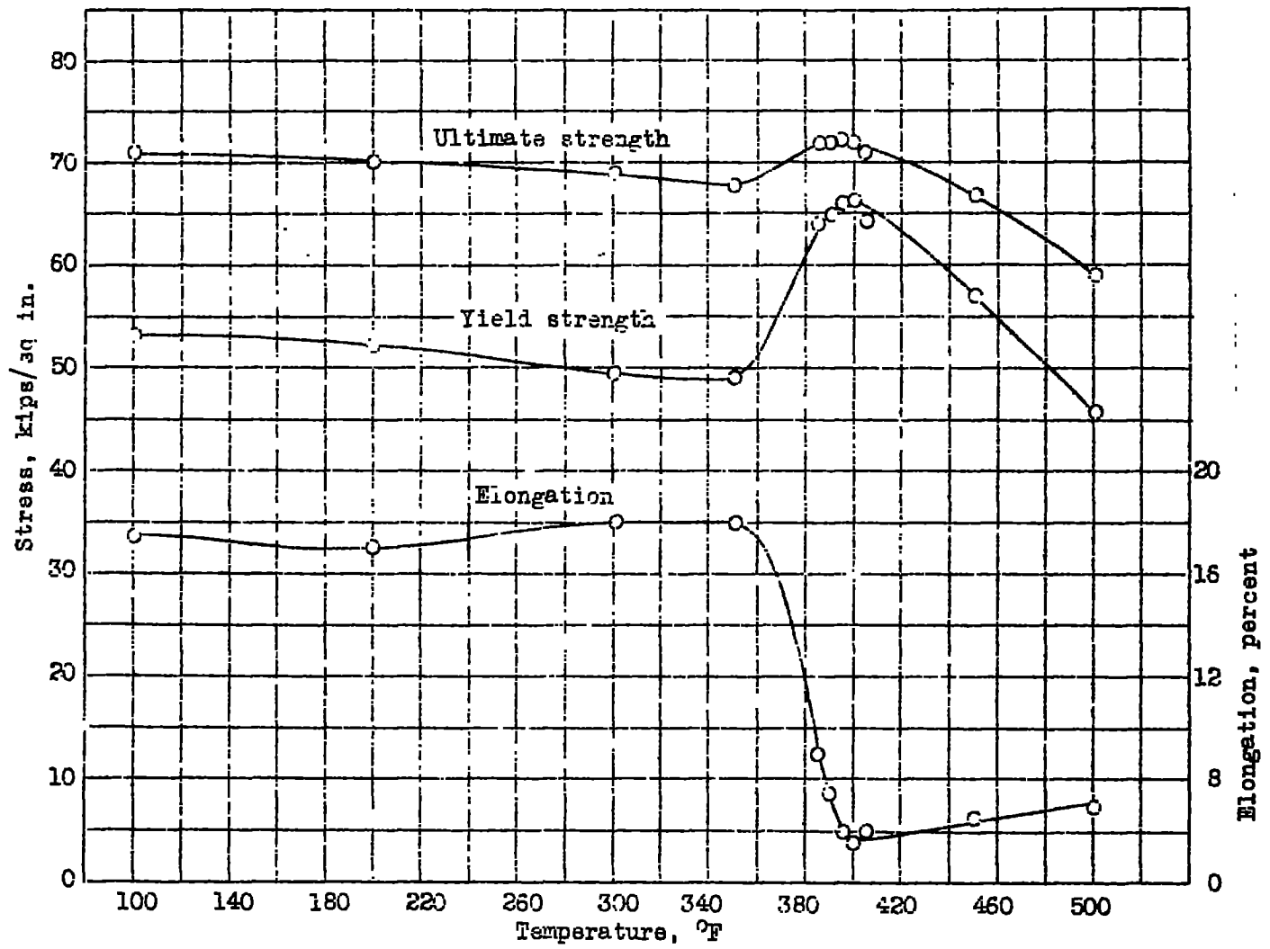
Figure 5.- Tensile properties of 24S-T aluminum alloy aged for two hours at various temperatures.
