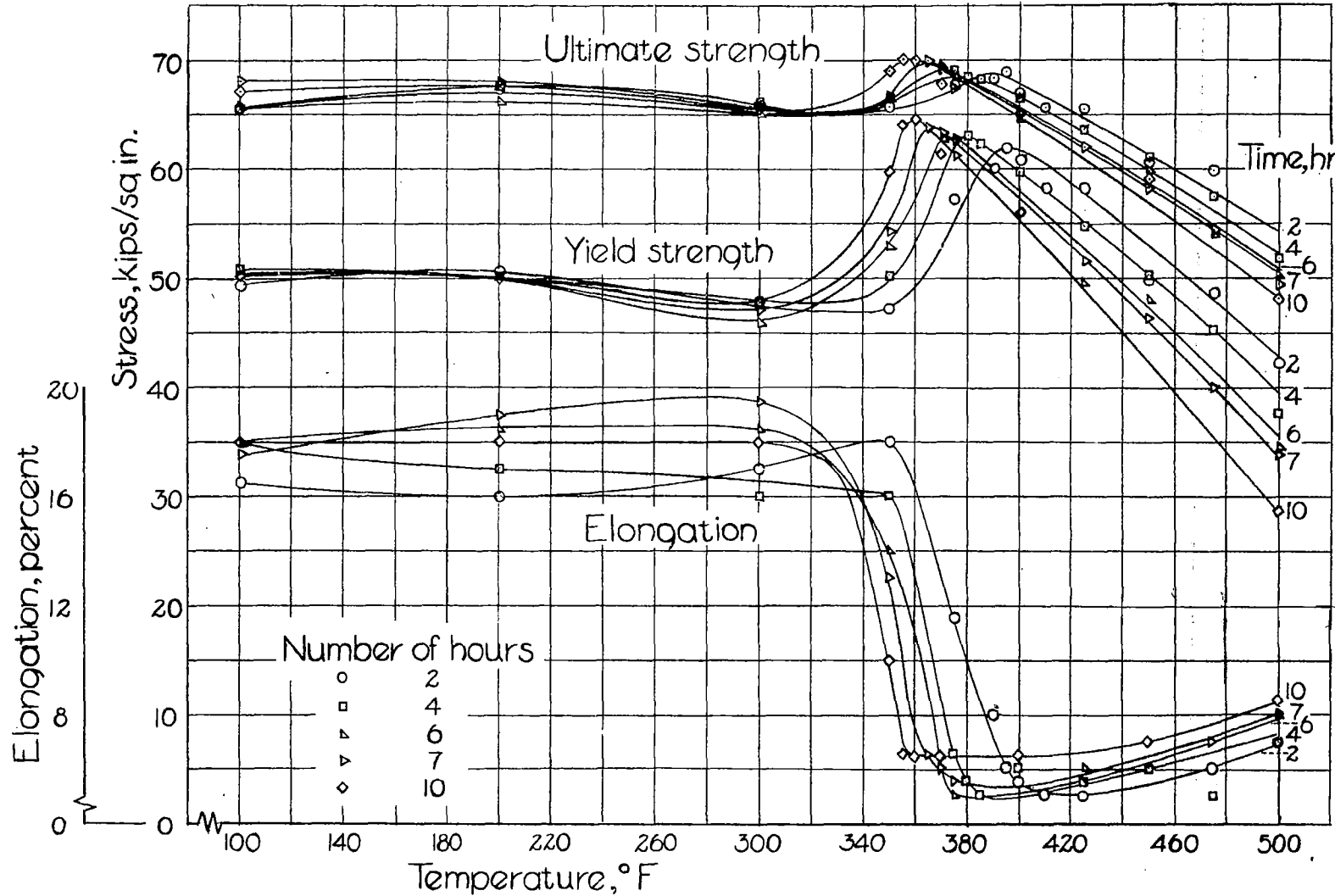
Figure 2.- Tensile properties of alclad 24S-T aluminum alloy aged for constant periods of time at various temperatures.
