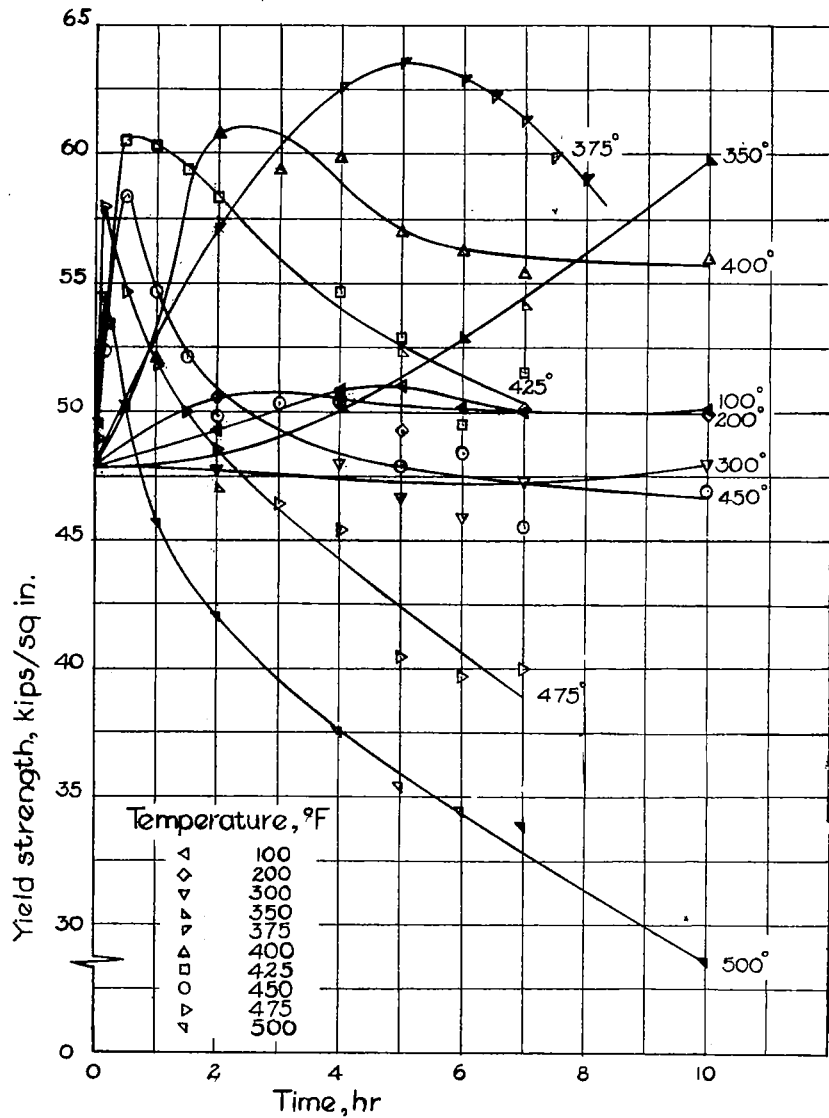
Figure 3.-Tensile yield strength for alclad 24S-T aluminum alloy aged at constant temperatures and various times.
