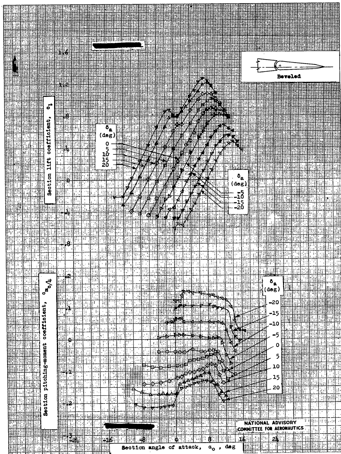
Figure 16.- Lift and pitching-moment characteristics of an NACA 651-210 airfoil equipped with a sealed-gap 0.20c plain aileron with beveled trailing edge. Tests, TDT 858, 859.
