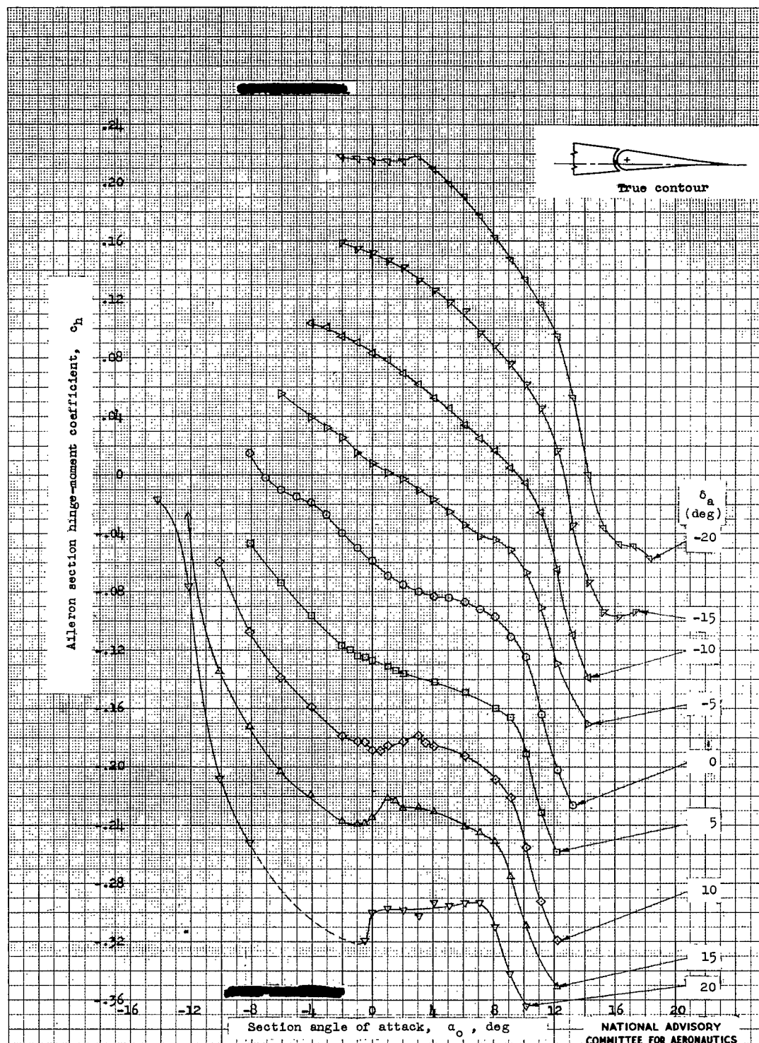
(a) R = 1 \times 10^6 . Figure 4.- Hinge-moment characteristics of a sealed-gap 0.20c plain aileron of true airfoil contour on an NACA 65 1 -210 airfoil section. Tests, TDT 847, 853.
