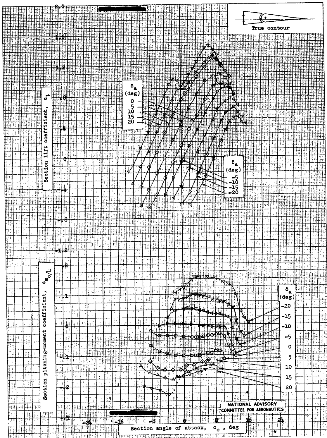
Figure 3.- Lift and pitching-moment characteristics of an NACA 65 1 -210 airfoil section equipped with a sealed-gap 0.20c plain aileron of true airfoil contour. Tests, TDT 847, 849, and 850.
