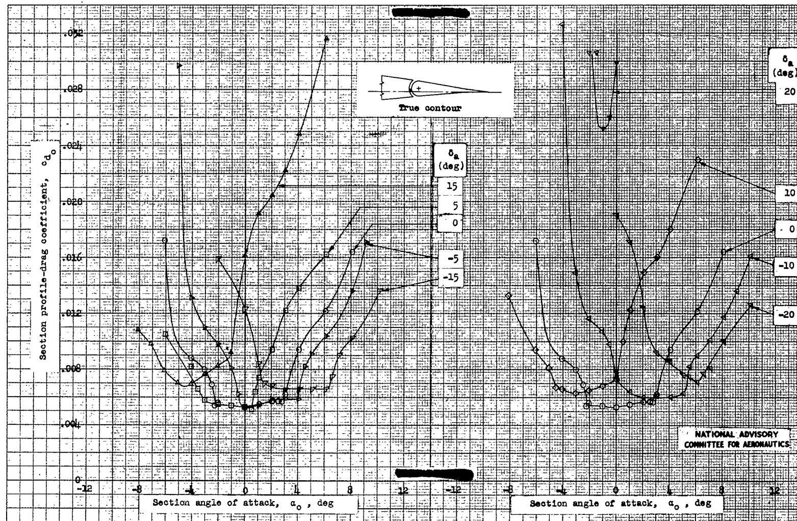
Figure 6.- Drag characteristics of an NACA 65 1 -210 airfoil section equipped with a sealed-gap 0.20c plain aileron of true airfoil contour. Tests, TDT 845, 847, and 848.
