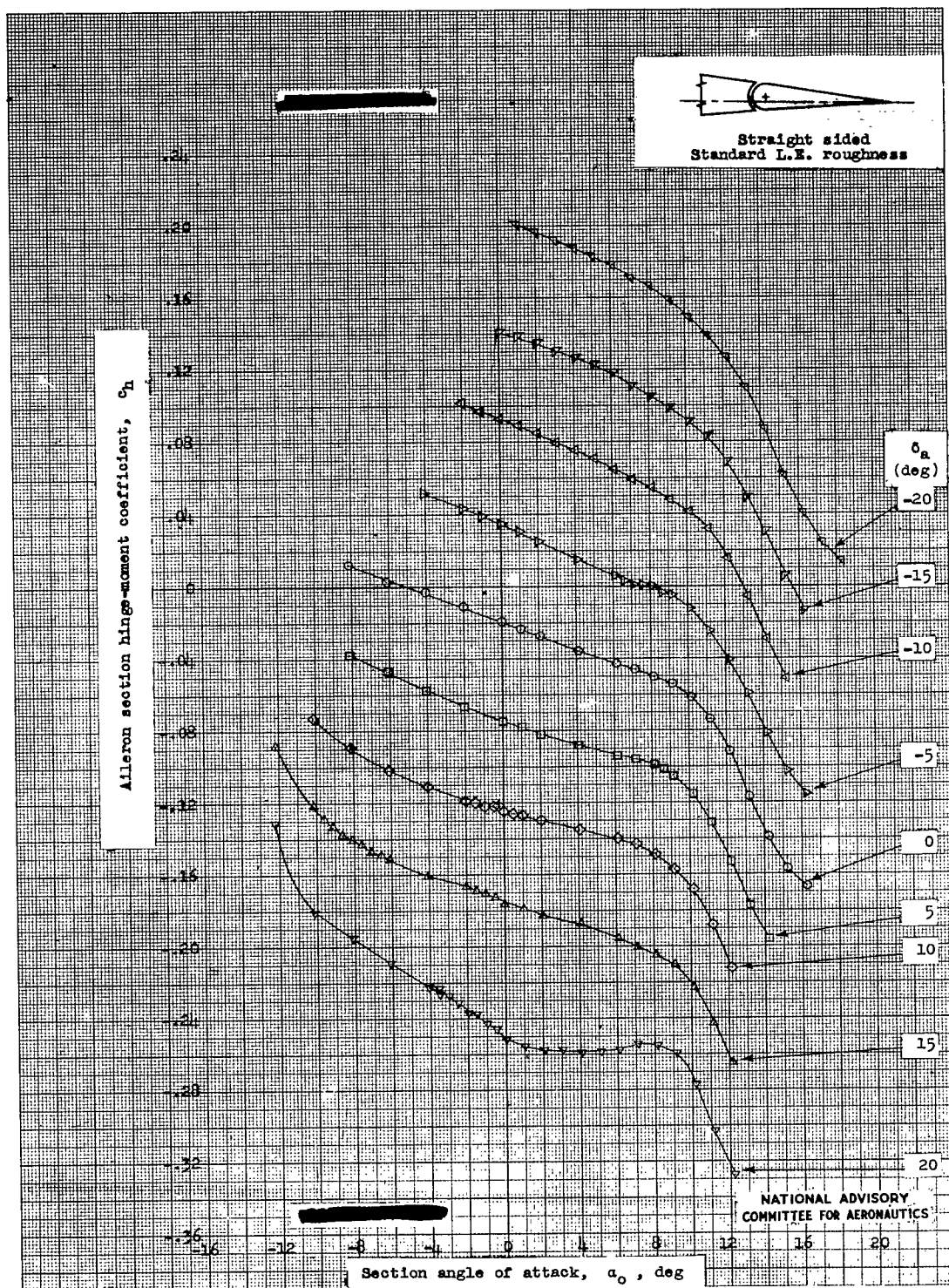
Figure 14.- Hinge-moment characteristics of a sealed-gap 0.20c plain aileron with straight sides on an NACA 651-210 airfoil section having standard leading-edge roughness. R = 9 \times 10^6 ; test, TDT 863.
