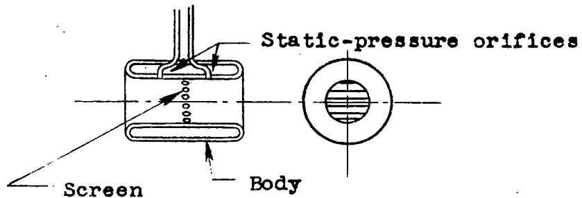
Figure 11.- Sketch of proposed rate-of-icing head with static-pressure orifices replacing pitot tube.
