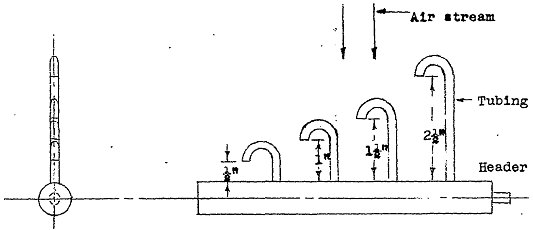
Figure 13.- Rate-of-icing indicator A.
