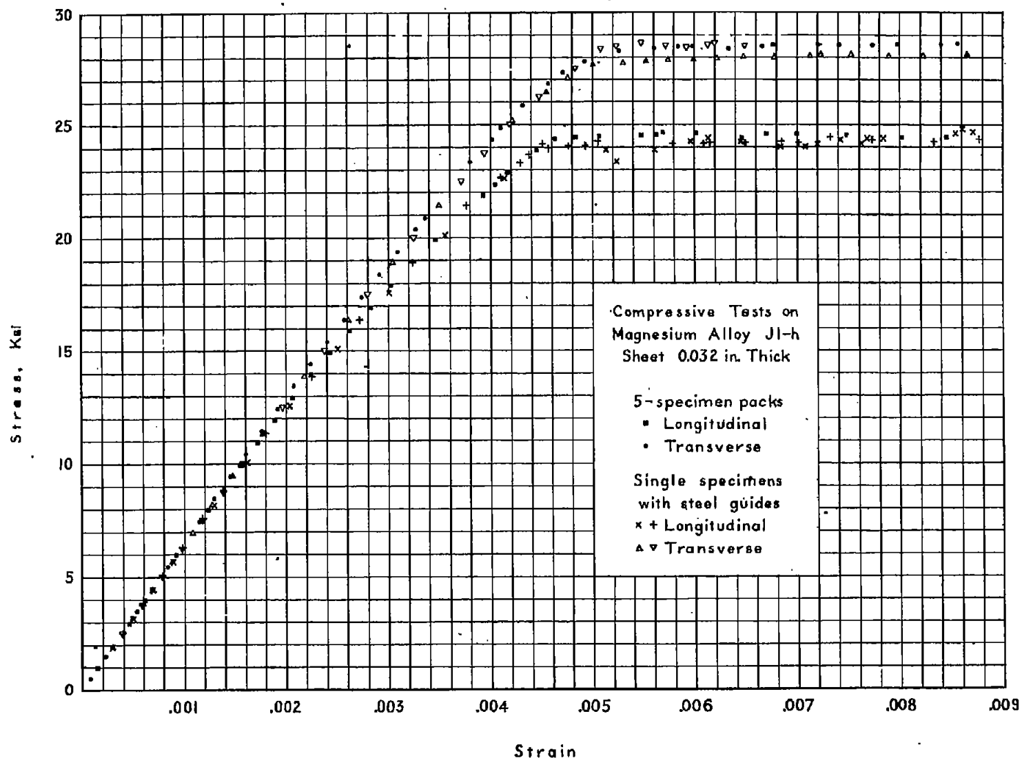
Figure 7.- Compressive stress-strain graphs, .032-inch magnesium alloy J1-h sheet.
