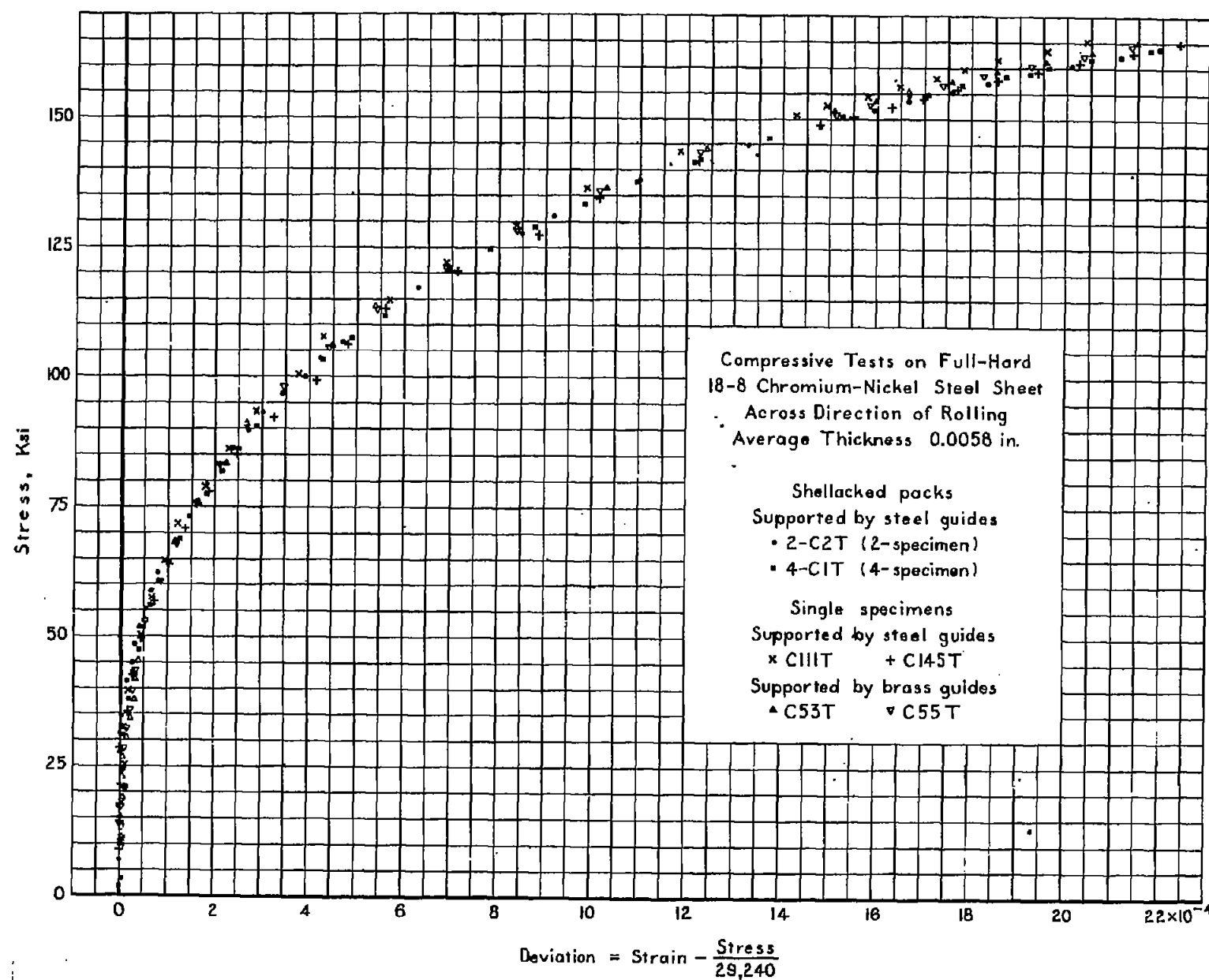
Figure 9.- Compressive stress-deviation graphs, .005-inch full-hard 18-8 chromium-nickel steel sheet, transverse specimens.
