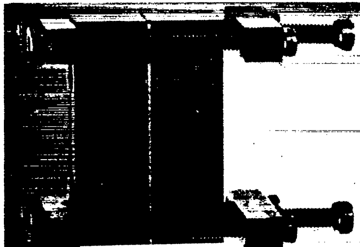
Figure 1.- Improvised solid brass guide fixture for compressive tests of thin sheet metal.
