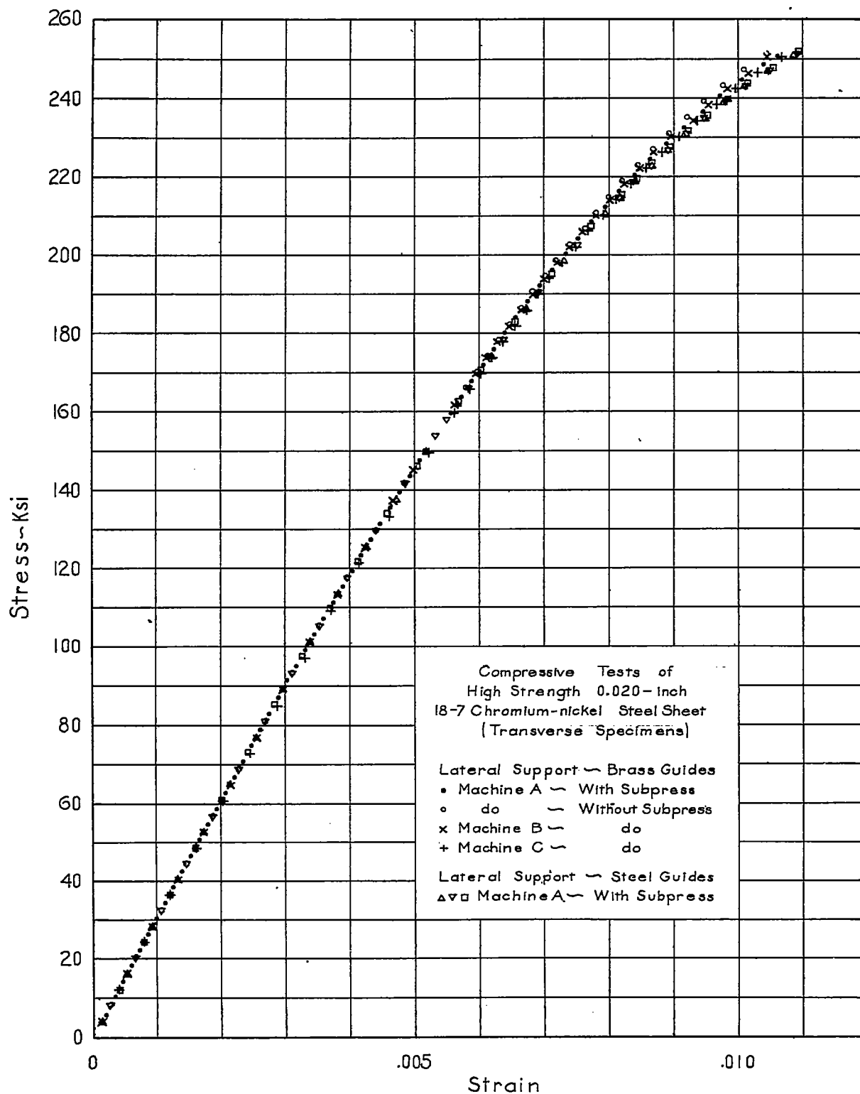
Figure 8.- Compressive stress-strain graphs, .020-inch 18-7 chromium-nickel steel sheet, transverse specimens.
