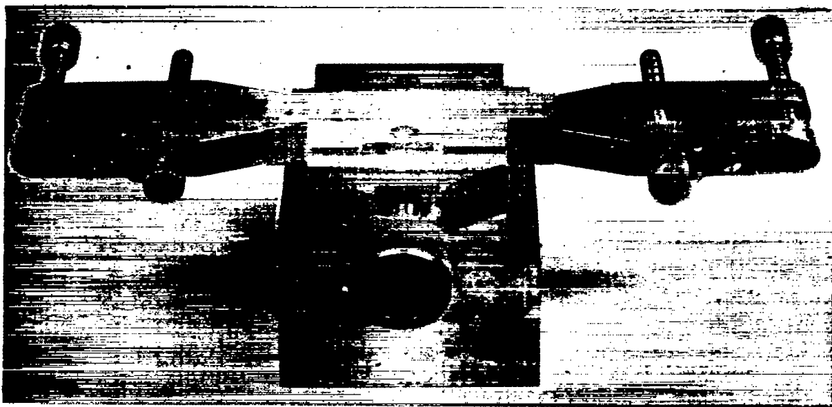
Figure 4.- Pack of specimens in machining fixture ready for grinding one side.
