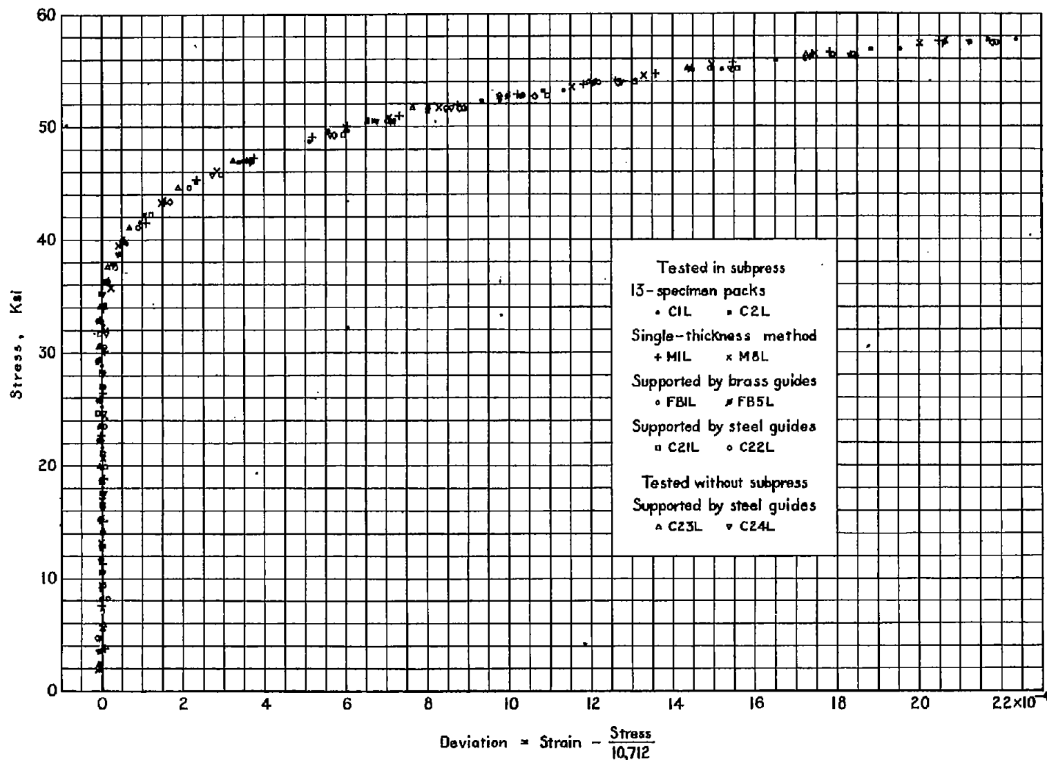
Figure 6.- Compressive stress-deviation graphs, .032-inch aluminum alloy 248-RT sheet, longitudinal specimens.
