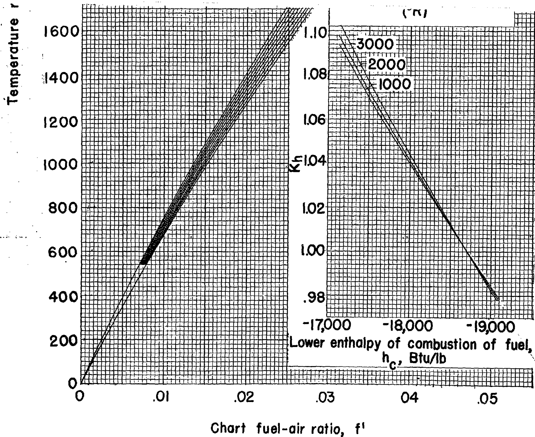
Figure 5.- Temperature rise during ideal constant-pressure combustion as a
