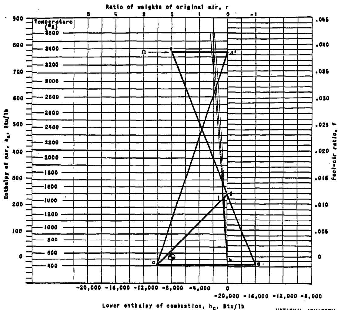
Figure 4. - Use of the constant pressure alignment chart to determine the temperature of after burning of richer-than-stoichiometric exhaust gas.
