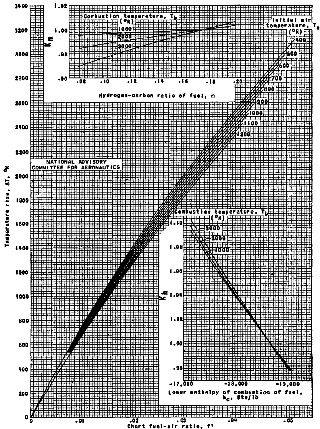
Figure 5. - Temperature rise during ideal constant-pressure combustion as a function of initial temperature; f = f' K_m K_h . (A 15- by 21-in. print of this figure is attached.)
