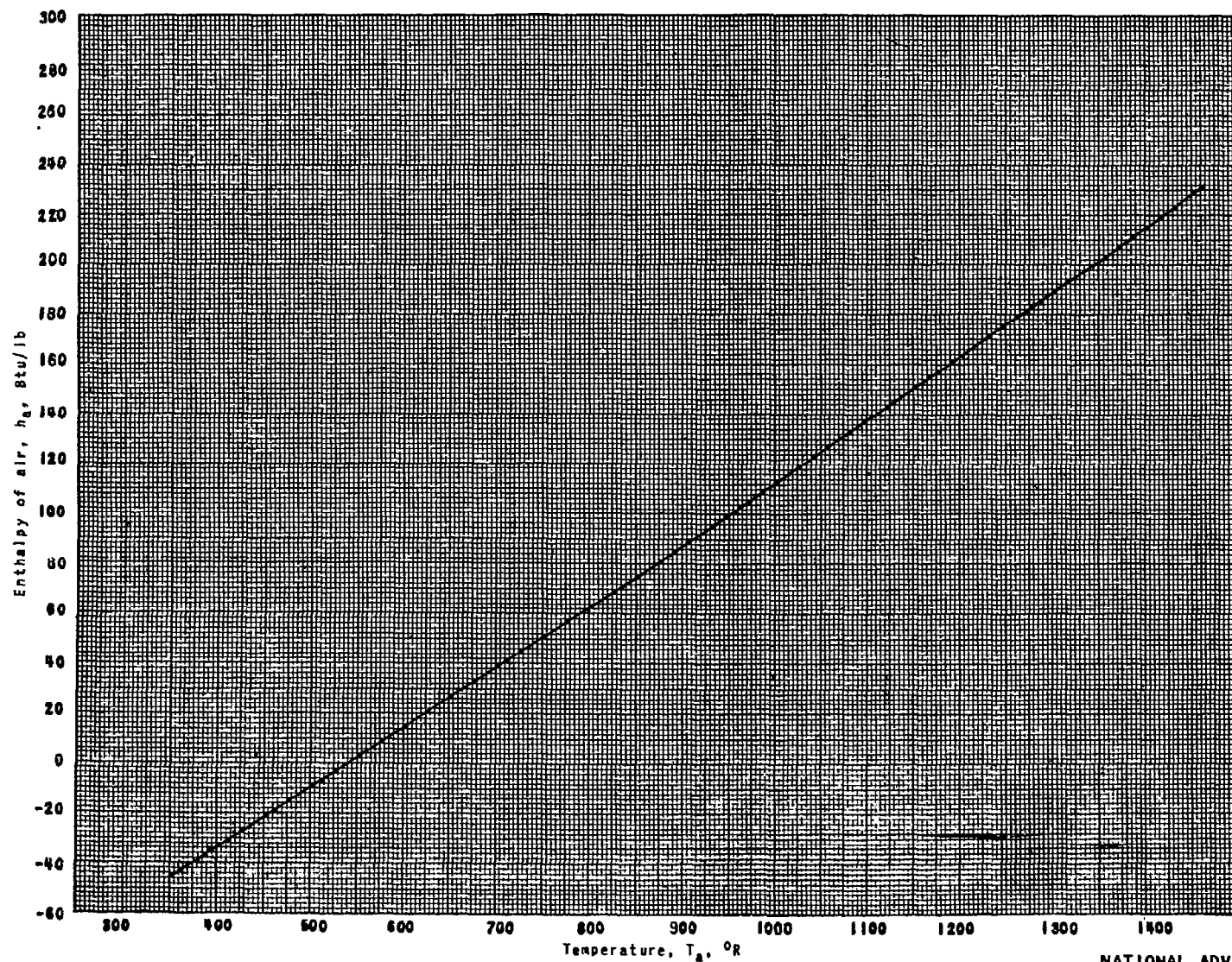
Figure 7. - Enthalpy of air.
