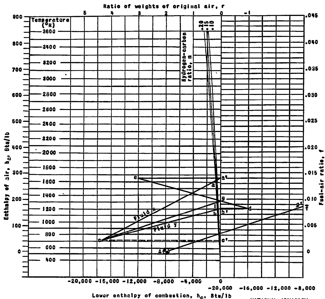
(d) Temperature of a mixture of combustion gases. Figure 2. - Concluded.
