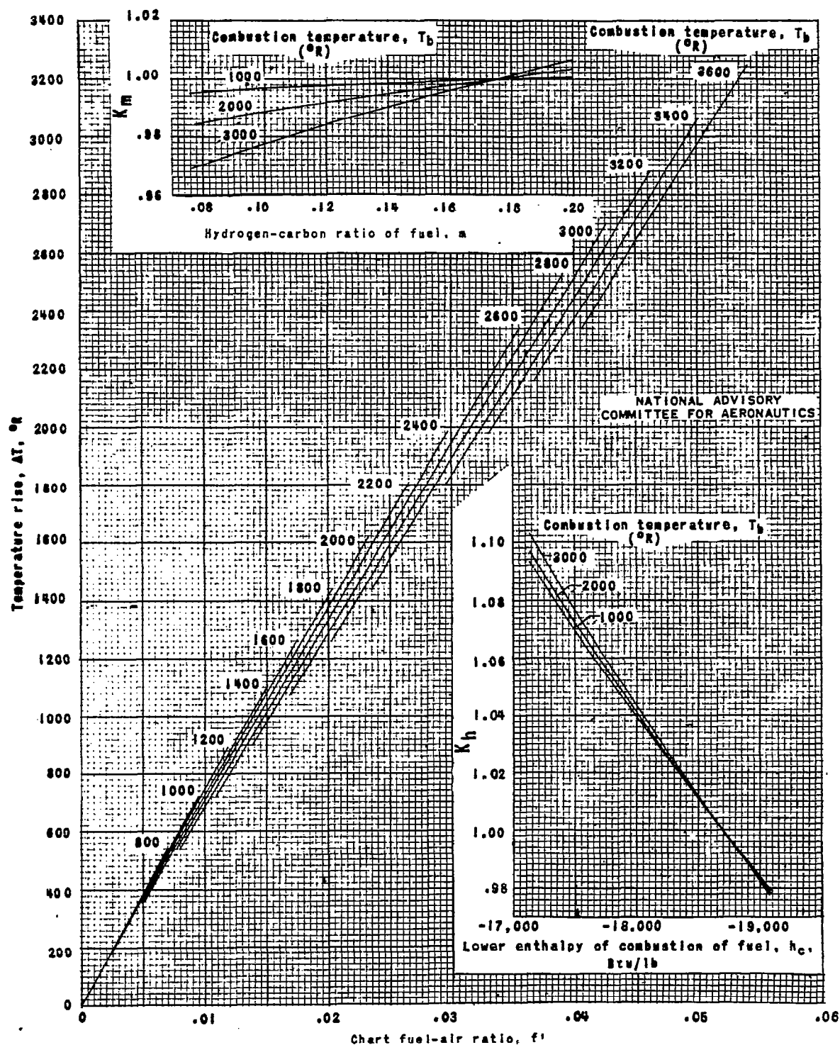
Figure 6. - Temperature rise during ideal constant pressure combustion as a function of the combustion temperature; f = f' K_M K_h . (A 16- by 21-in. print of this figure is attached.)
