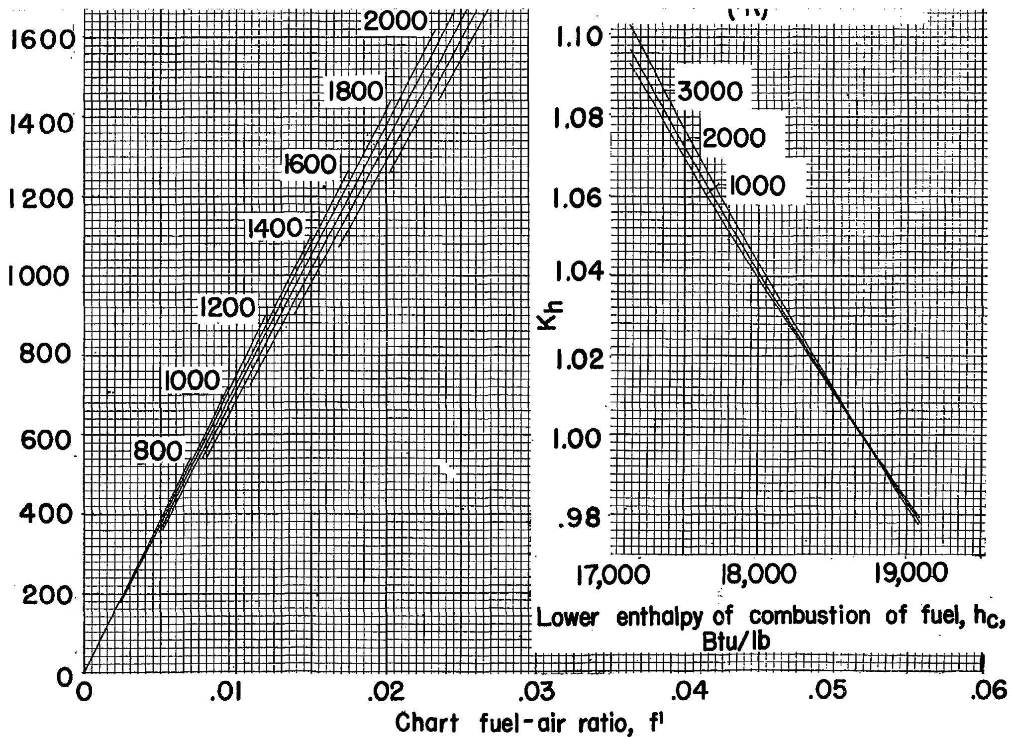
Figure 6.- Temperature rise during ideal constant-pressure combustion as a function of the combustion temperature: f = f' K_m K_h .
