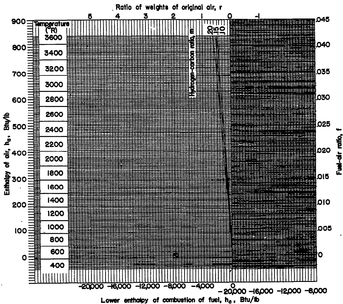
Figure 1. - Constant-pressure alignment chart. (A 25- by 25-in. print of this figure is attached.)
