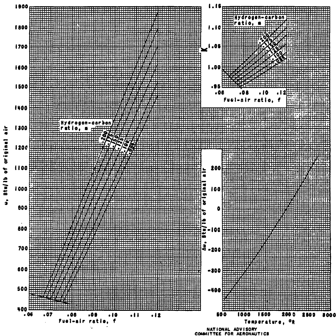
Figure 3. - Total enthalpy \Omega of richer-than-stoichiometric exhaust gas. \Omega = \omega + K\Delta\omega . (A 17 \frac{1}{2} - by 19-in. print of this figure is attached.)
