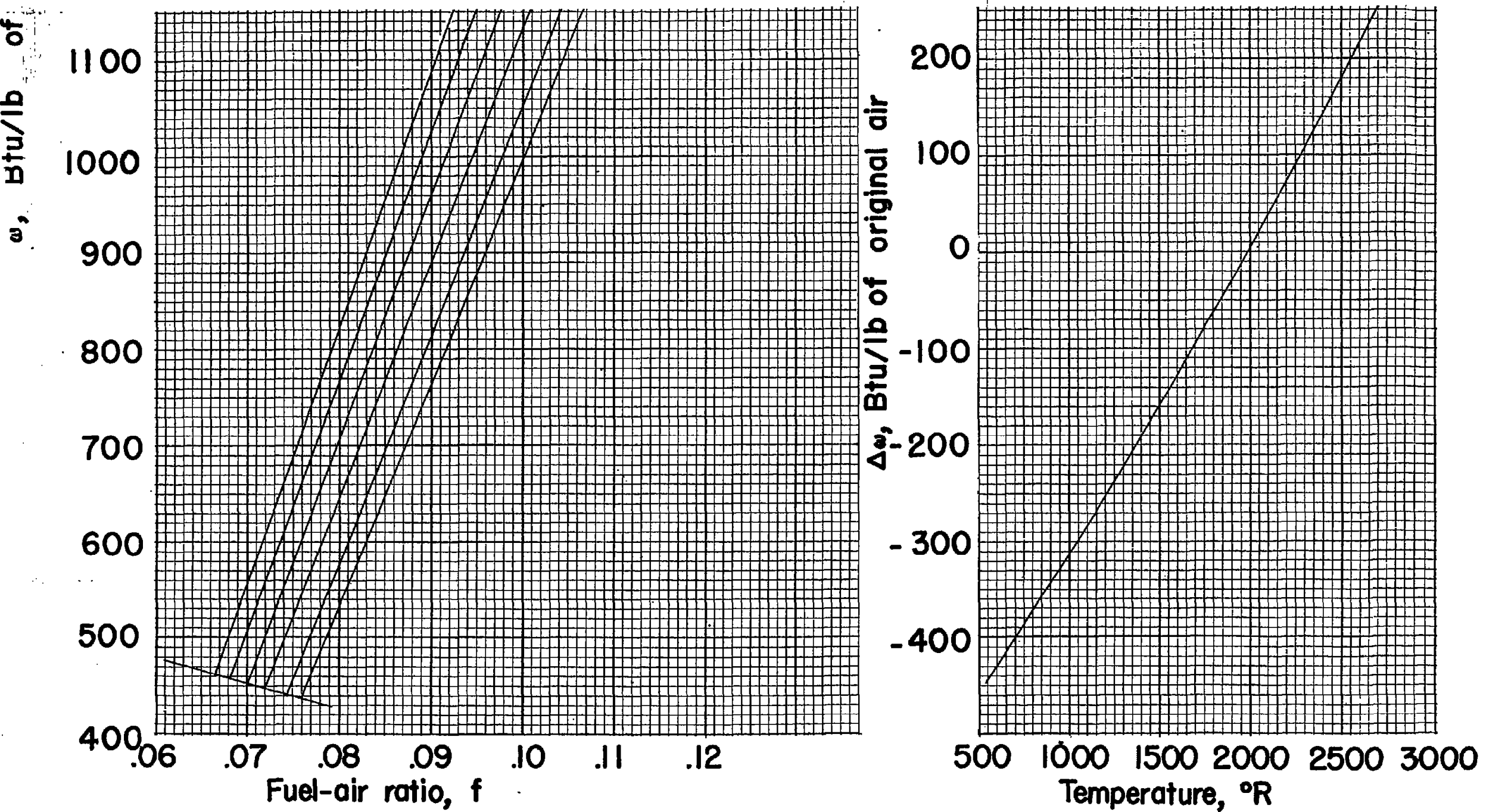
Figure 3.- Total enthalpy \Omega of richer-than-stoichiometric exhaust gas. \Omega = \omega + K\Delta\omega
