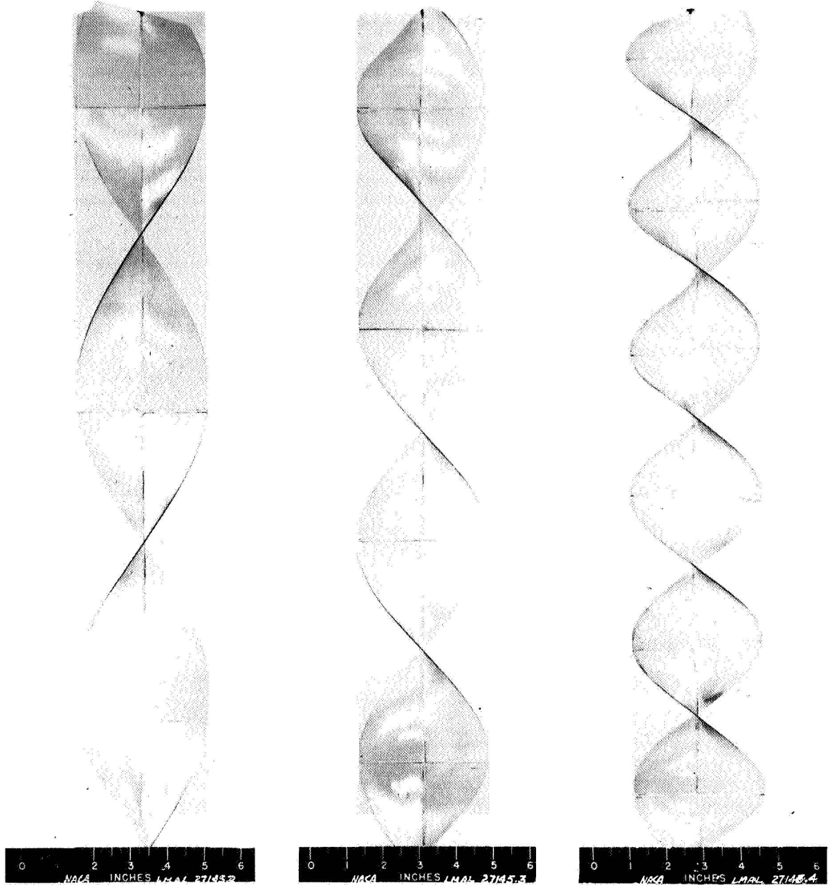
Figure 8.- Two-blade single-rotation helix surfaces with guide vanes.
