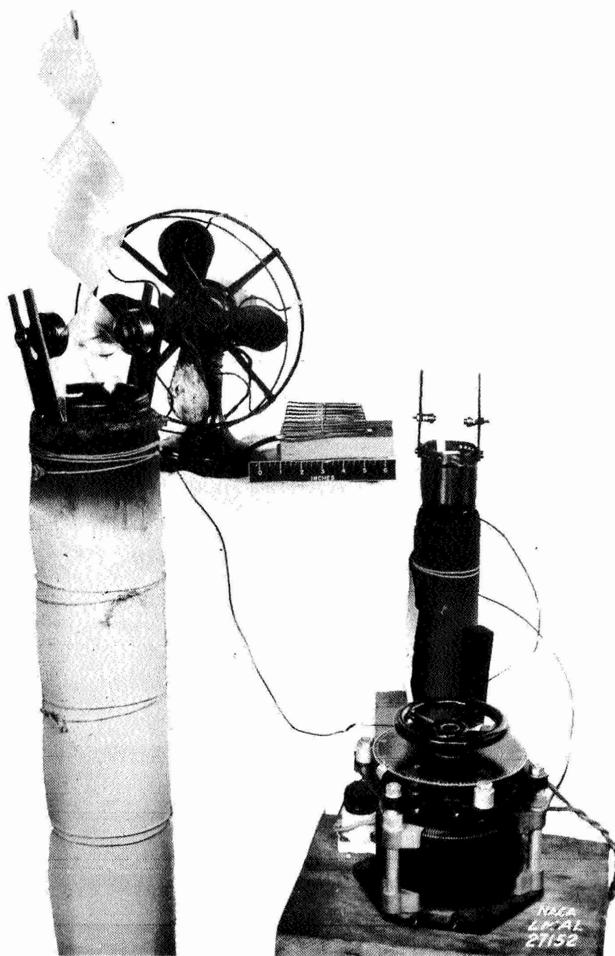
Figure 5.- Equipment for constructing celluloid helix surfaces.
