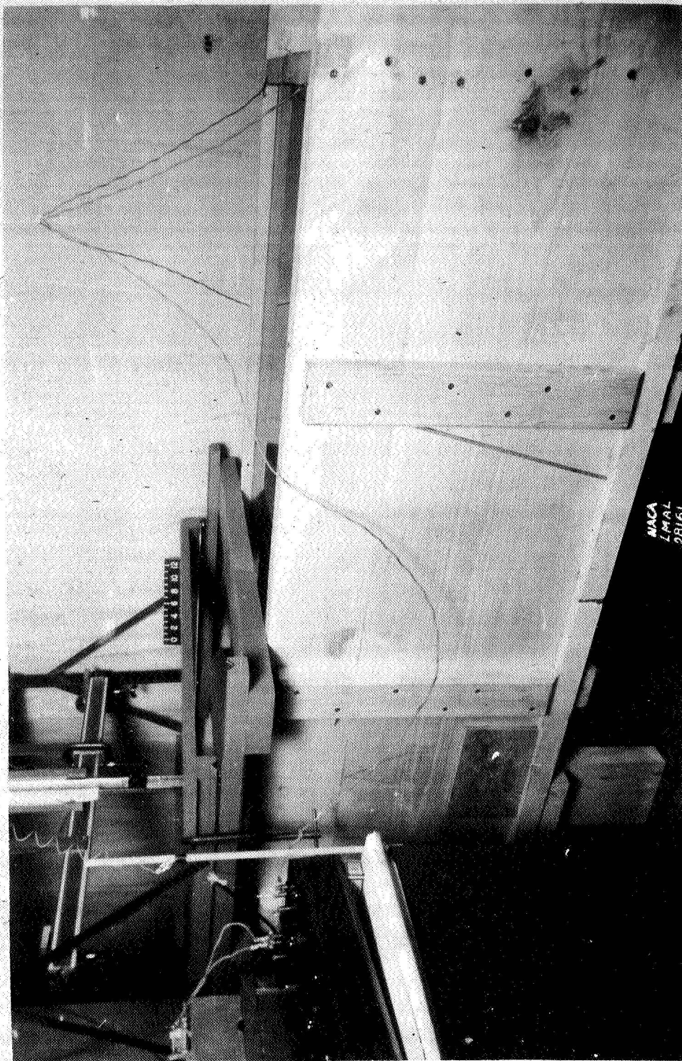
Figure 14.- Unit cell for high pitch.
