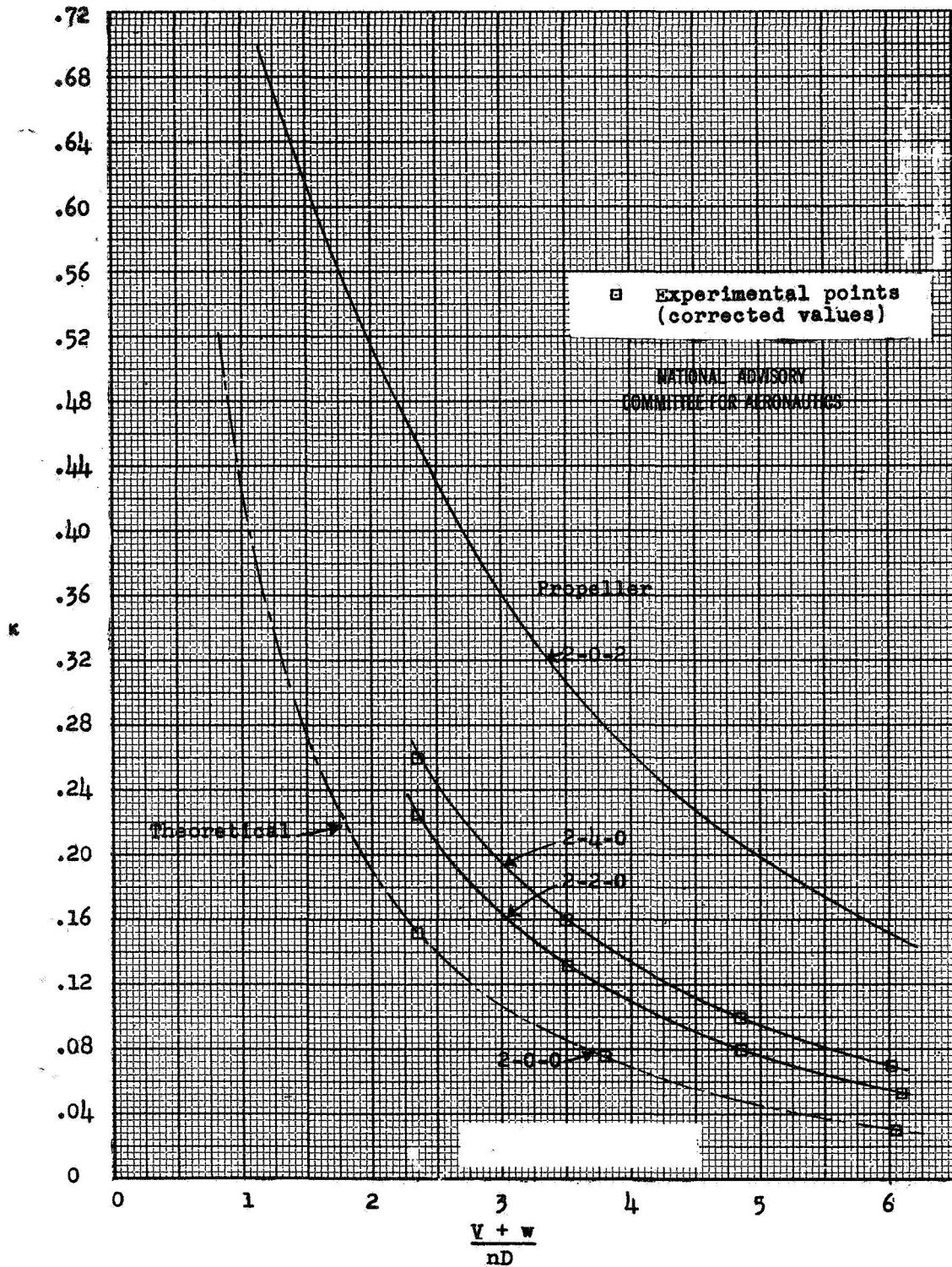
(a) Single-rotating two-blade propellers.
