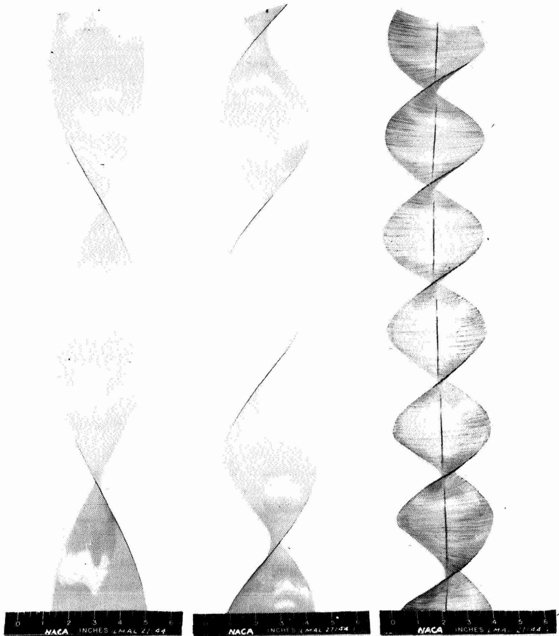
Figure 6.- Celluloid single helix surfaces. (On right, preliminary laminated construction.)
