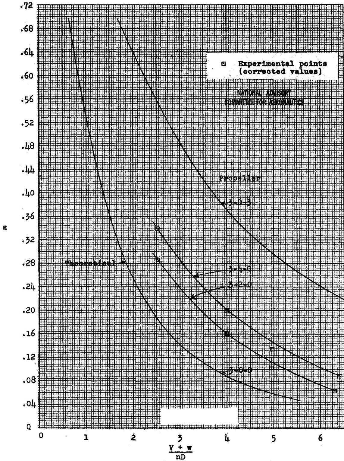
(b) Single-rotating three-blade propellers.
