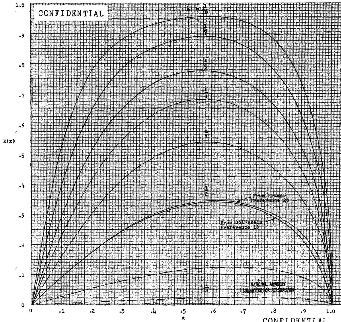
Figure 1.- The function K(x) for several values of \lambda for two-blade propellers.
