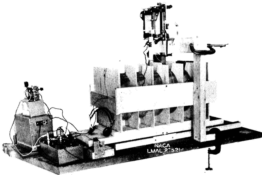
Figure 10.- Setup for measuring the potential distribution K(x) for single-rotation wake models.
