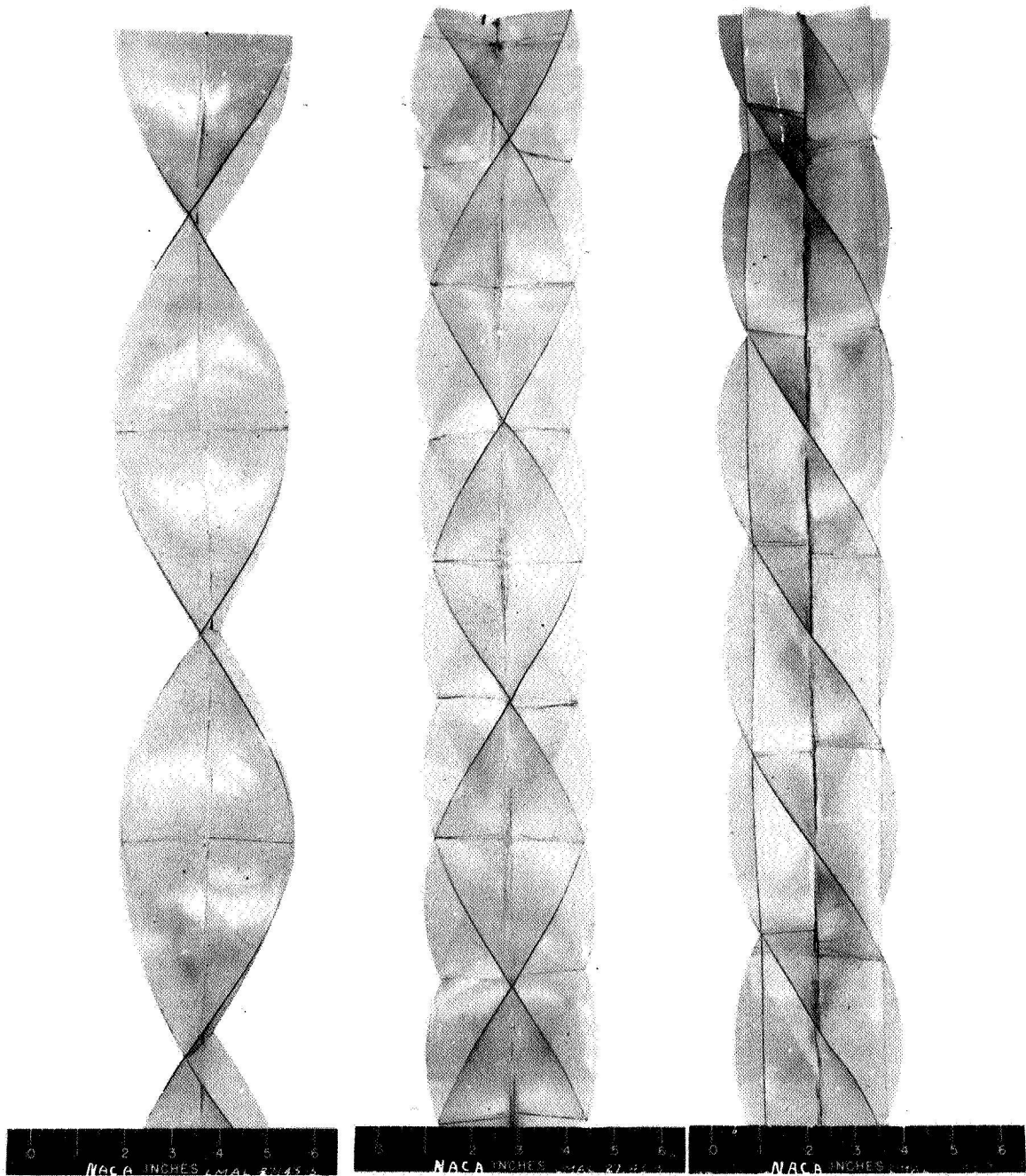
(a) Left and center - for four and six blades, dual rotation. Right - for four blades, single rotation, with four-blade guide vanes.
