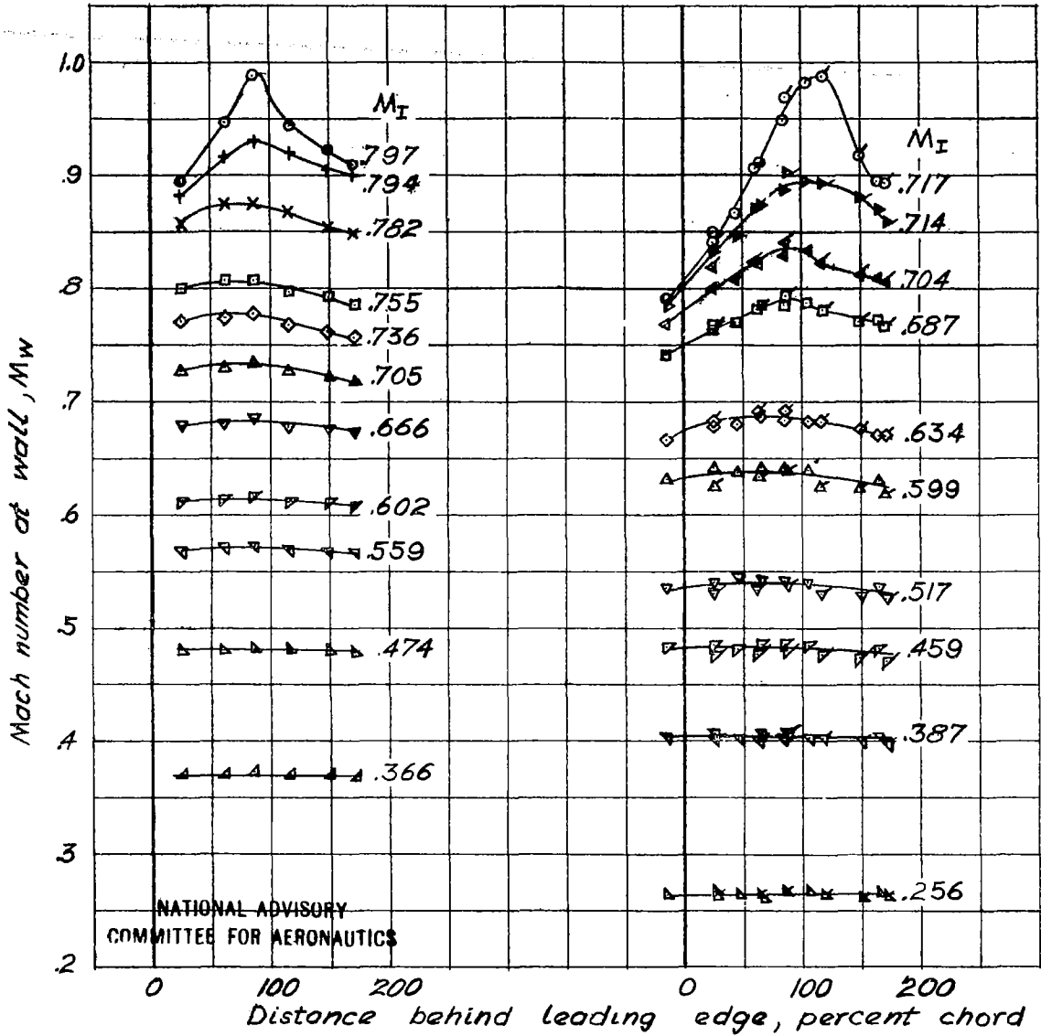
(c) NACA 16-215 airfoil section, 5-inch chord; M_{cr} = 0.71 .
