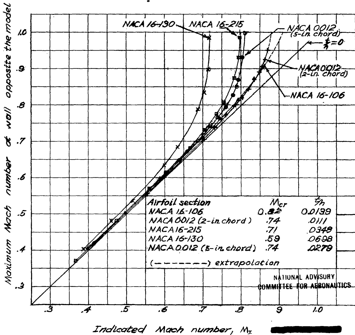
Figure 4.-Variation in the maximum Mach number at the tunnel wall opposite the model with indicated Mach number.
