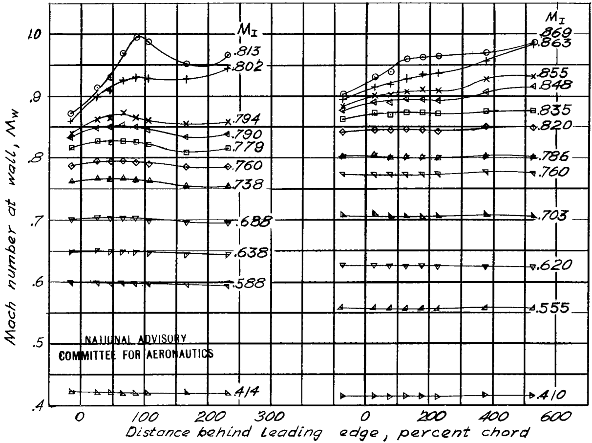
(e) NACA 0012 airfoil section, 5-inch chord; M_{cr} = 0.74 .
