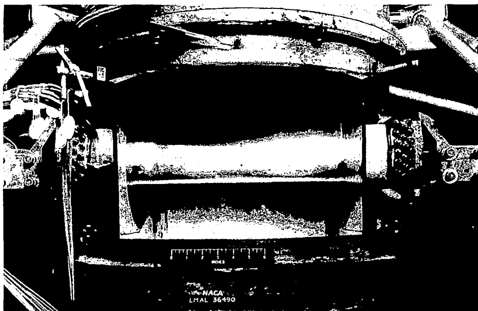
(a) Test section, access door removed.
