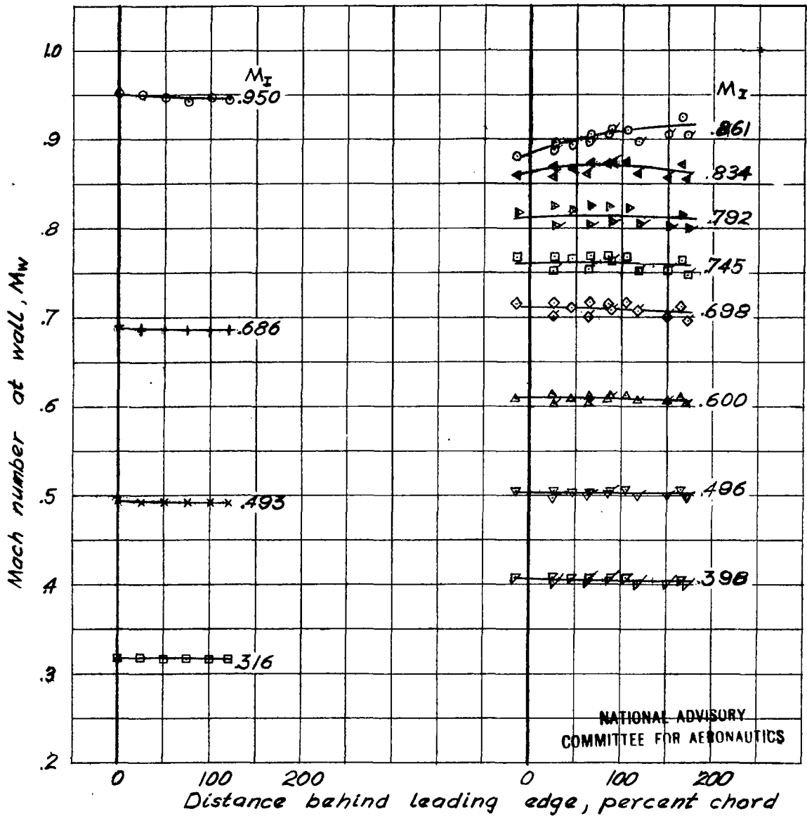
(a) Tunnel empty.
