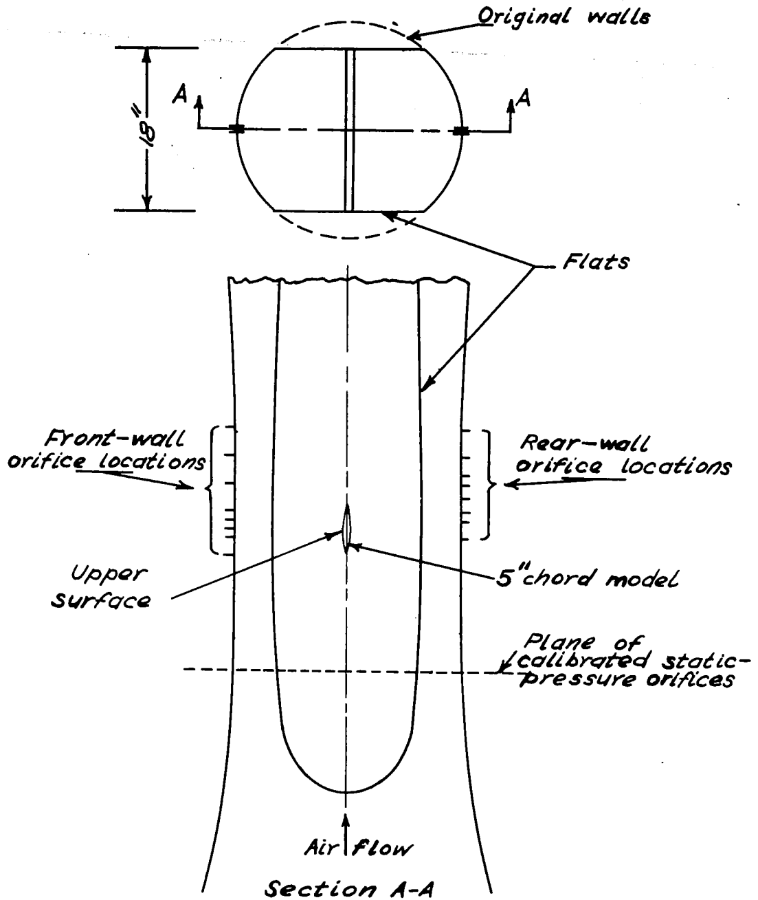
Figure 2. - Modified Langley 24-inch high-speed tunnel.
