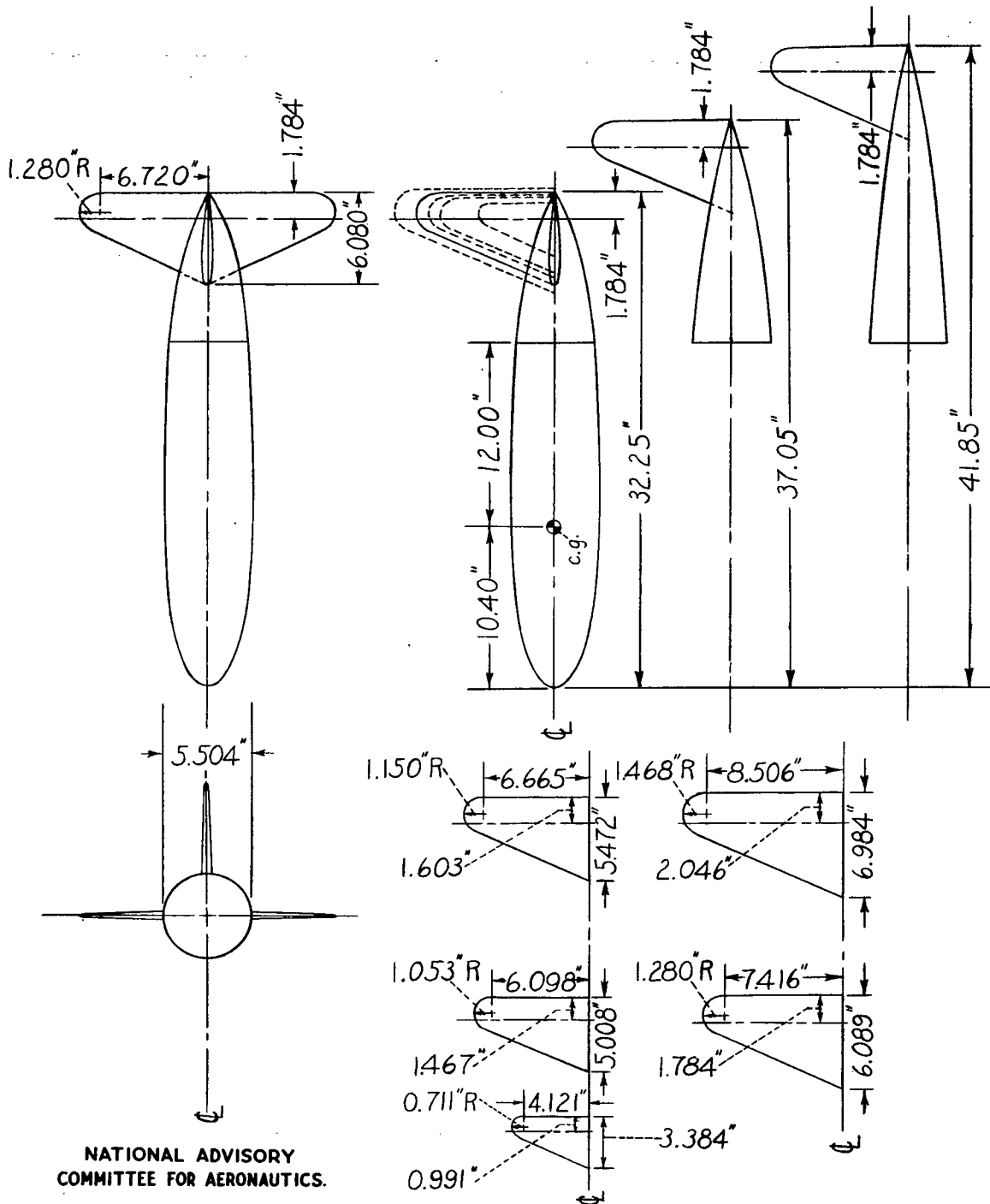
Figure 1.- The circular fuselage, vertical and horizontal tails, and tail cones with the principal dimensions for assembly.
