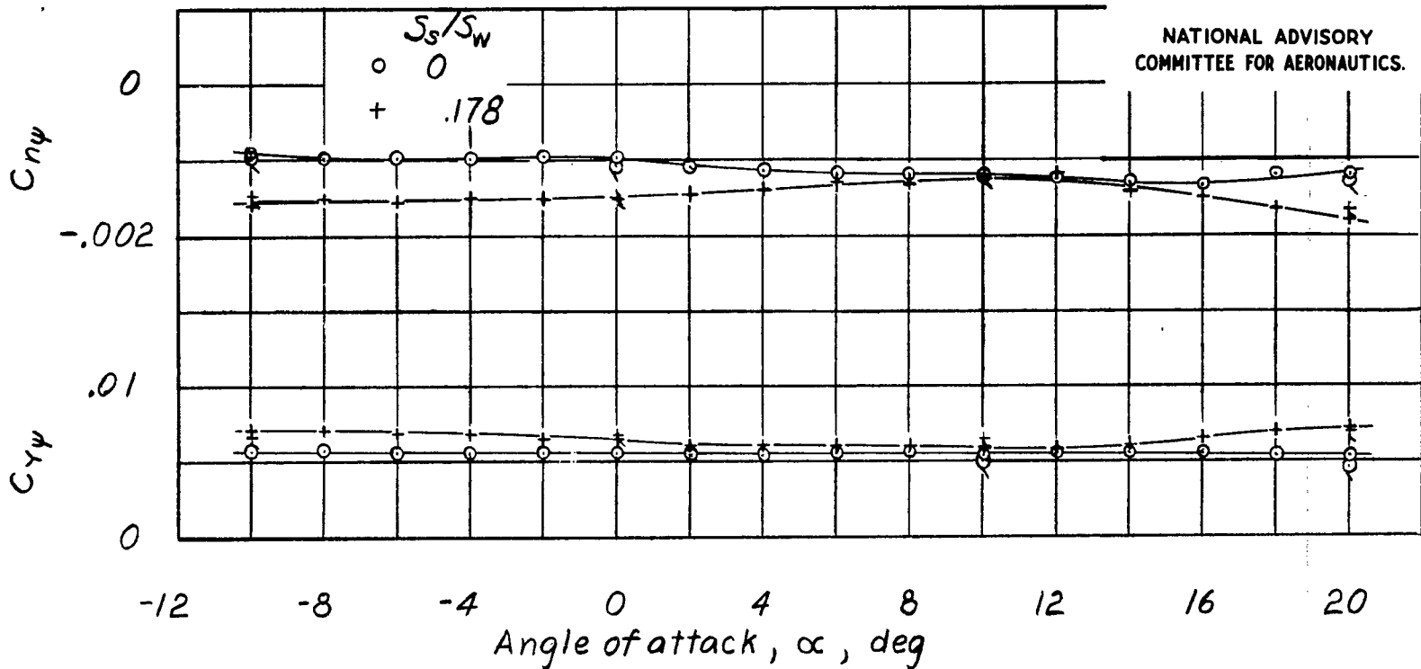
Figure 16.- Effect of horizontal tail surface on rate of change of stability derivatives C_{Y\psi} and C_{n\psi} with angle of attack.
