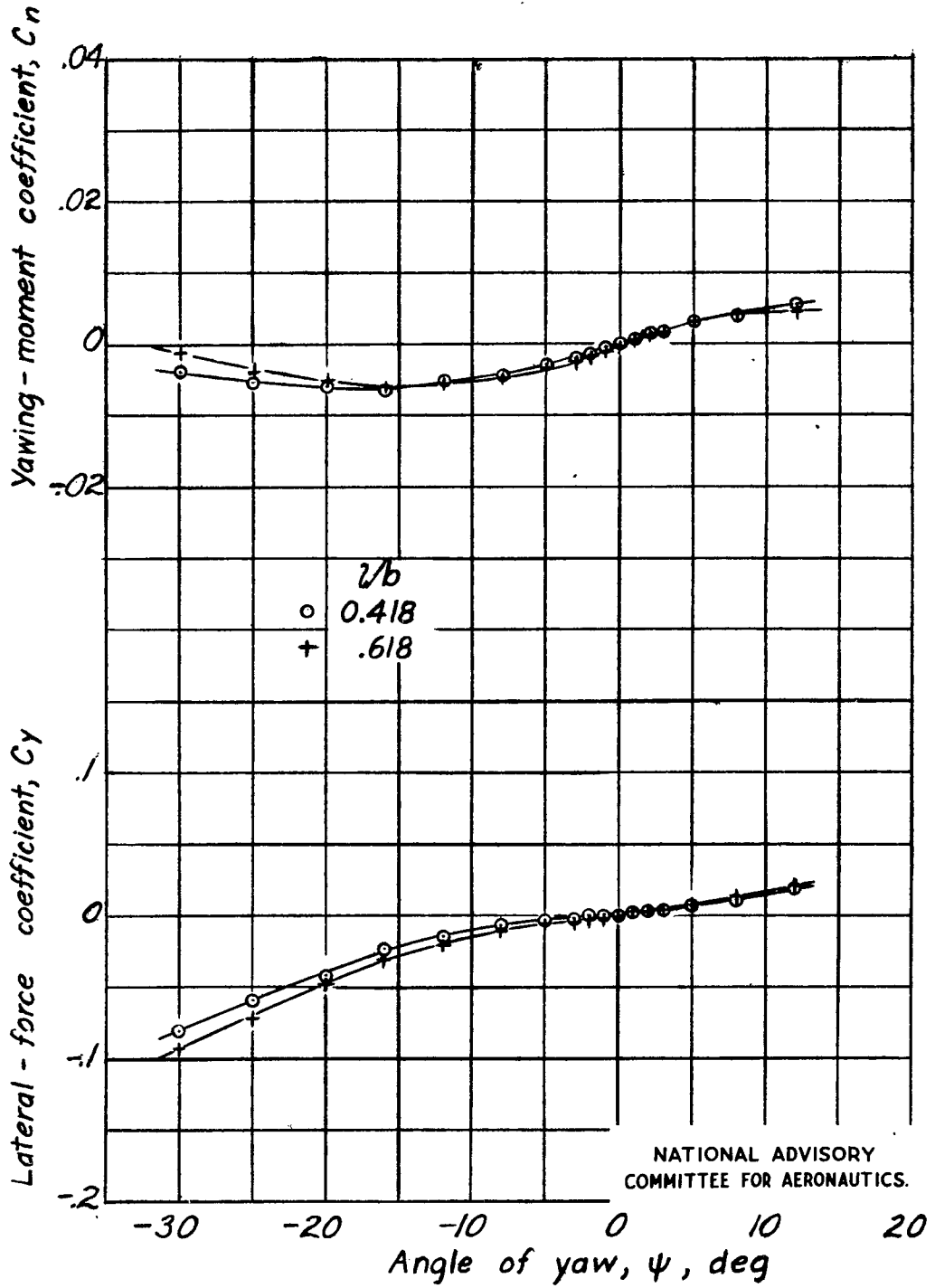
Figure 7.- Effect of changing fuselage length on rate of change of lateral-force and yawing-moment coefficients with angle of yaw. No horizontal or vertical tail surfaces; \alpha = 0^\circ .
