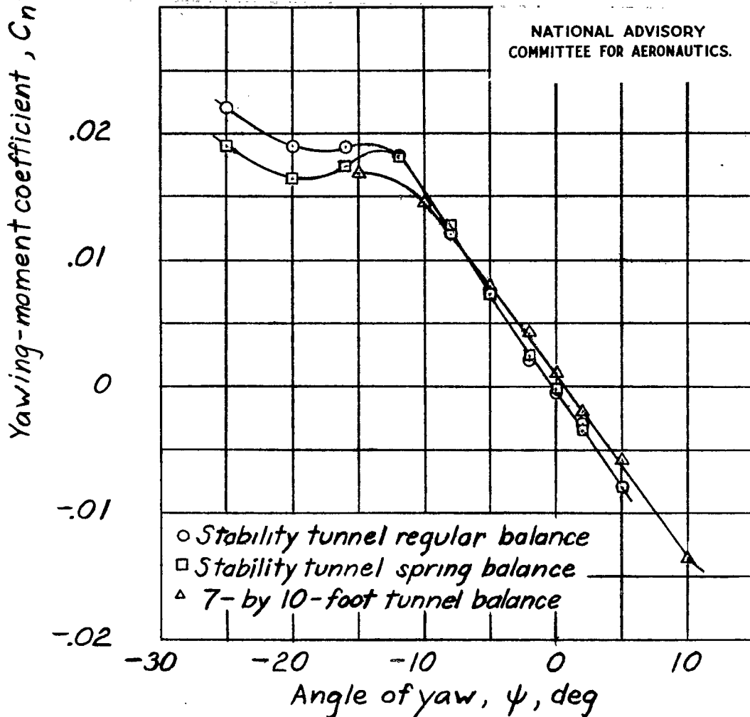
Figure 6.- Comparison of data obtained with NACA stability tunnel regular balance, NACA stability tunnel spring balance, and LMAL 7- by 10-foot tunnel balance for rate of change of yawing-moment coefficient with angle of yaw. Horizontal tail surface on; \frac{l}{b} = 0.418 ; vertical tail surface 4, \frac{S_f}{S_w} = 0.0974 ; \alpha = 0^\circ .
