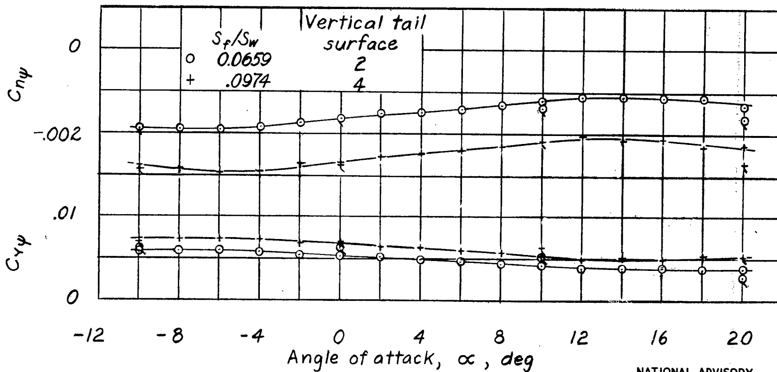
Figure 10.- Effect of changing vertical-tail area on rate of change of stability derivatives C_{Y\psi} and C_{N\psi} with angle of attack. Horizontal tail surface on; \frac{z}{b} = 0.618 .
