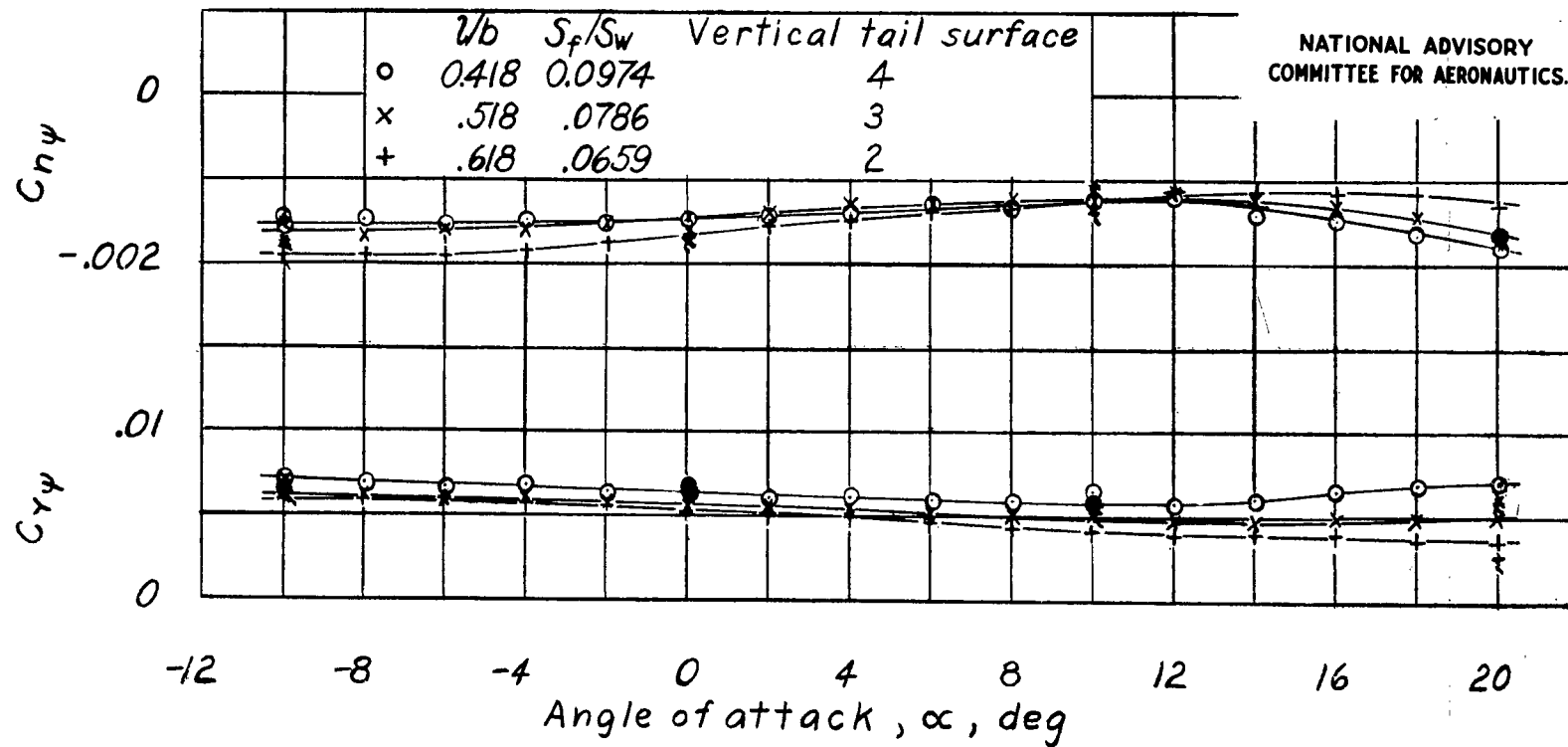
Figure 18.- Effect of different combinations having constant tail volume on rate of change of stability derivatives C_{Y\psi} and C_{N\psi} with angle of attack. Horizontal tail surface on.
