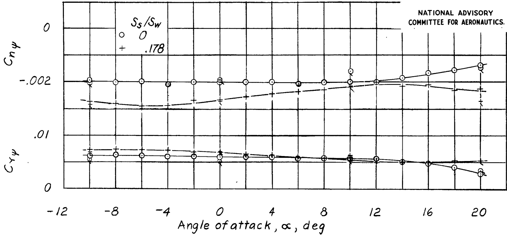
Figure 15.- Effect of horizontal tail surface on rate of change of stability derivatives C_{Y\psi} and C_{N\psi} with angle of attack.
