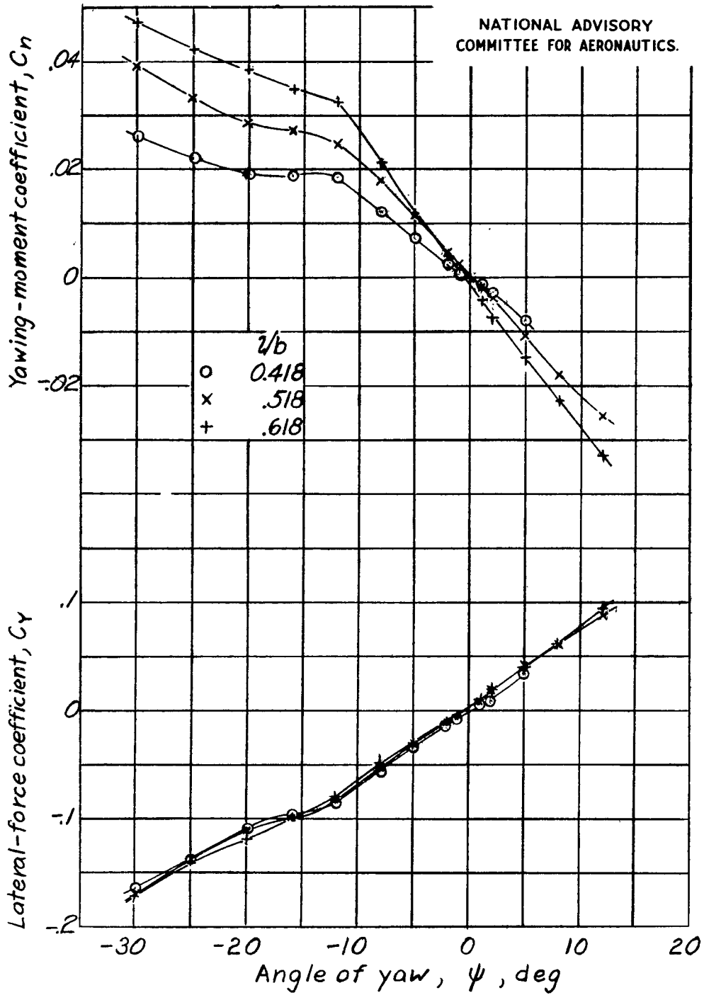
Figure 11.- Effect of changing tail length on rate of change of lateral-force and yawing-moment coefficients with angle of yaw. Horizontal tail surface on; vertical tail surface 4 , \frac{S_f}{S_w} = 0.0974 ; \alpha = 0^\circ .
