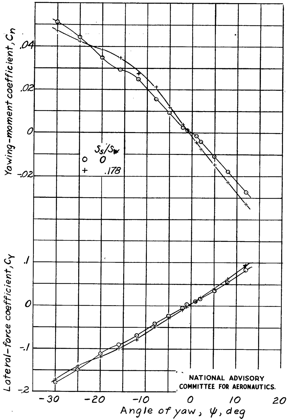
Figure 14.- Effect of horizontal tail surface on rate of change of lateral-force and yawing-moment coefficients with angle of yaw. \frac{l}{b} = 0.618 ; vertical tail surface \frac{l}{b} = 0.0974 ; \alpha = 0^\circ .
