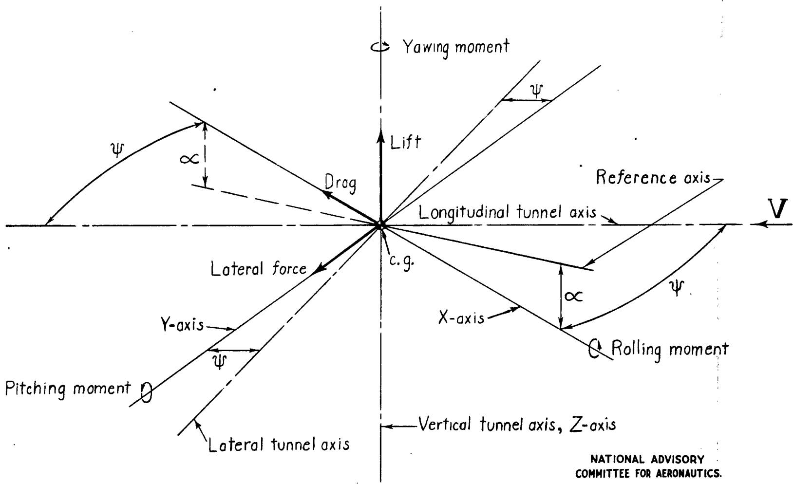
Figure 4.— System of axes used in the measurement of forces, moments, and angles.
