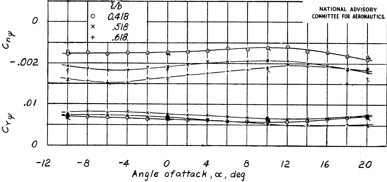
Figure 12.- Effect of changing tail length on rate of change of stability derivatives C_{y\psi} and C_{n\psi} with angle of attack. Horizontal tail surface on; vertical tail surface 4, \frac{S_f}{S_w} = 0.0974 .
