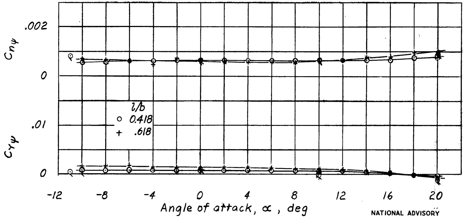
Figure 8.- Effect of changing fuselage length on rate of change of stability derivatives C_{Y\psi} and C_{n\psi} with angle of attack. No horizontal or vertical tail surfaces.
