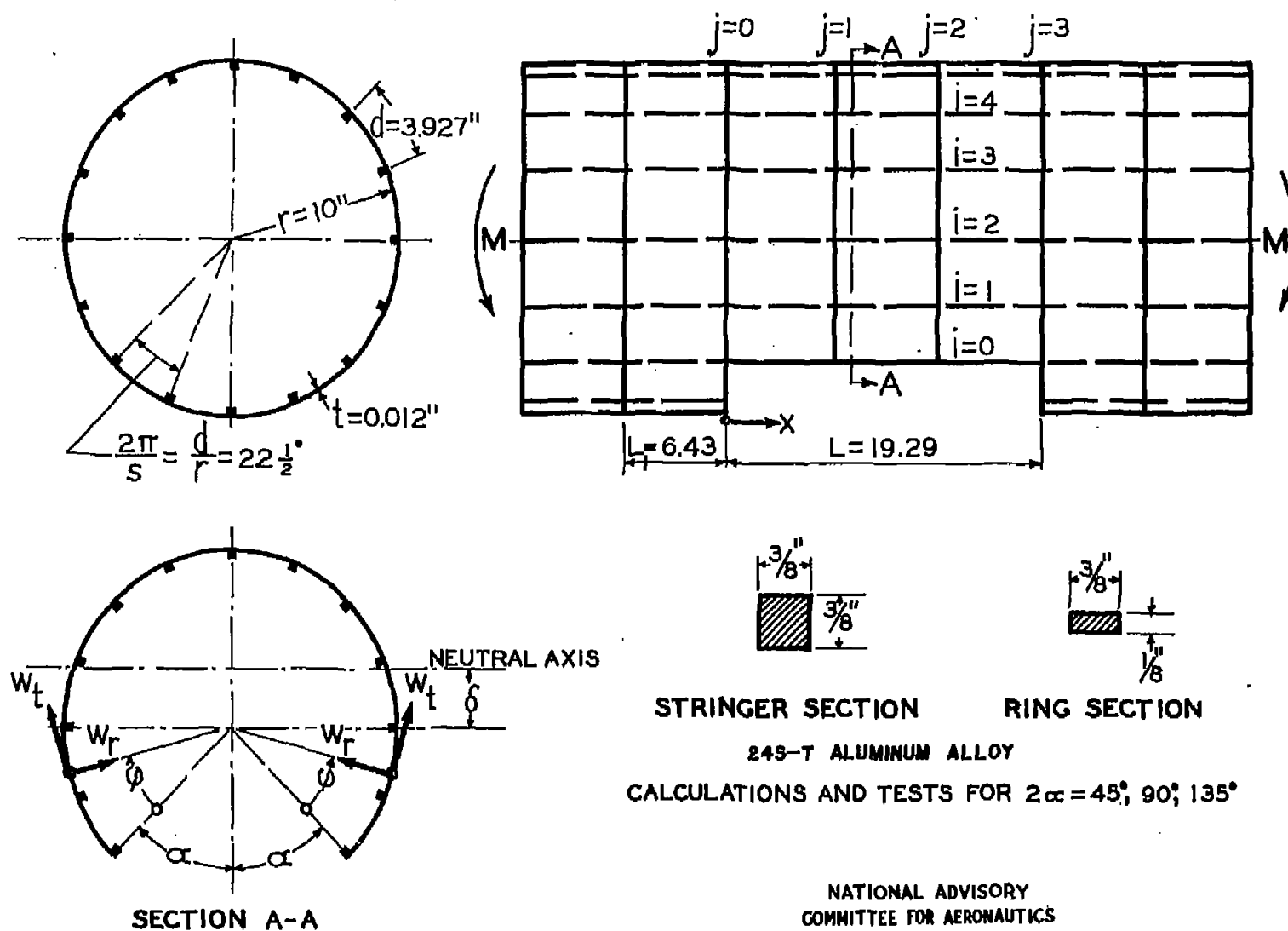
FIGURE 1.- MONOCOQUE CYLINDER.
