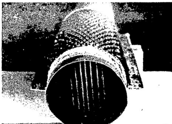
Figure 3.- Photograph of the flattened- tube crossflow type heat exchanger.
