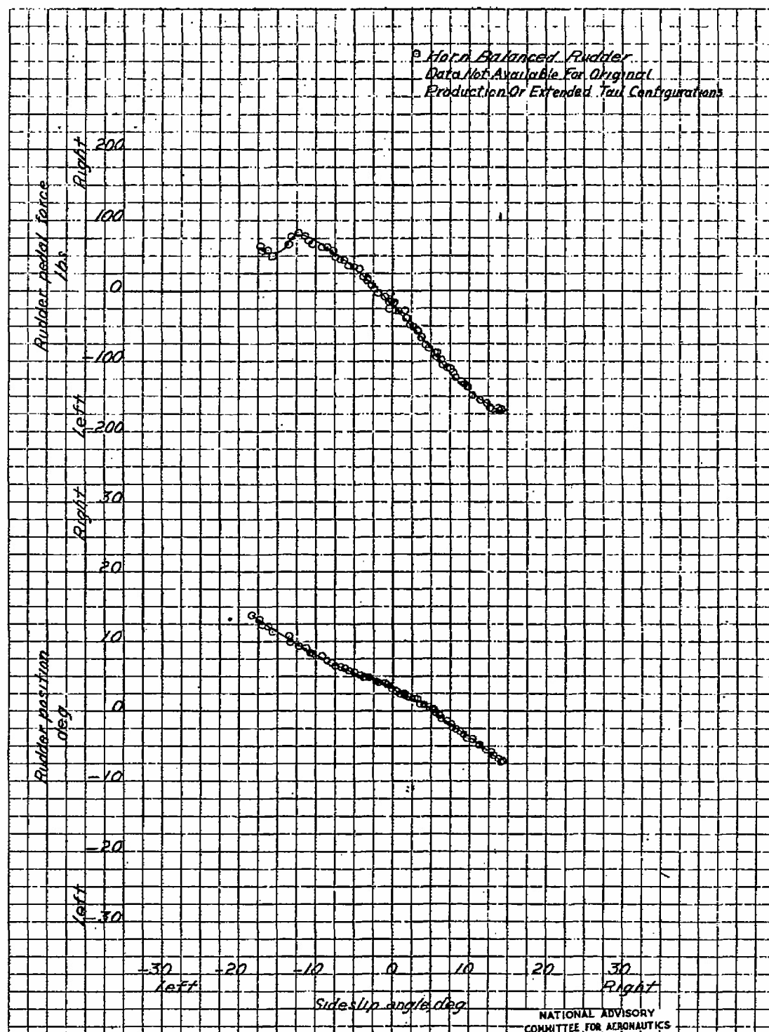
Figure 13.- Steady sideslip characteristics at 10,000 feet altitude, climbing condition V_{1S} = 200 miles per hour. P-51D-20-NA airplane with a horn balanced rudder, tab locked.
