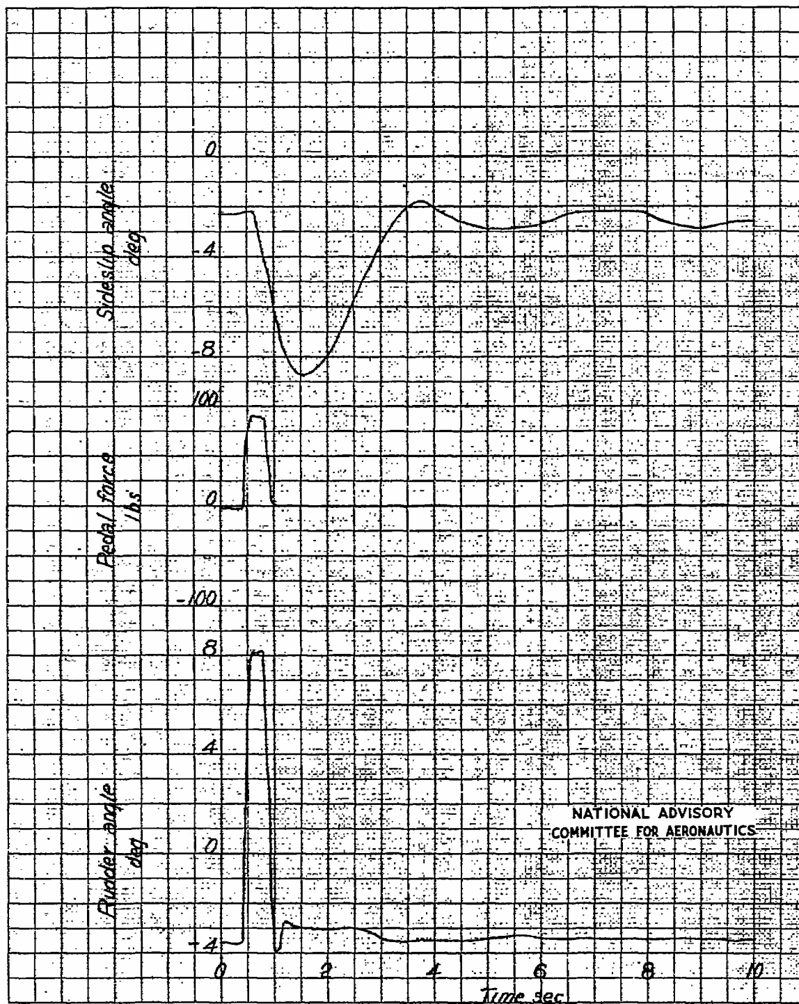
Figure 17.- A typical right rudder kick at 11,000 feet altitude, climbing condition V_{1S} = 150 miles per hour. P-51D-20-NA airplane with horn balanced rudder having the unbalancing tab locked.
