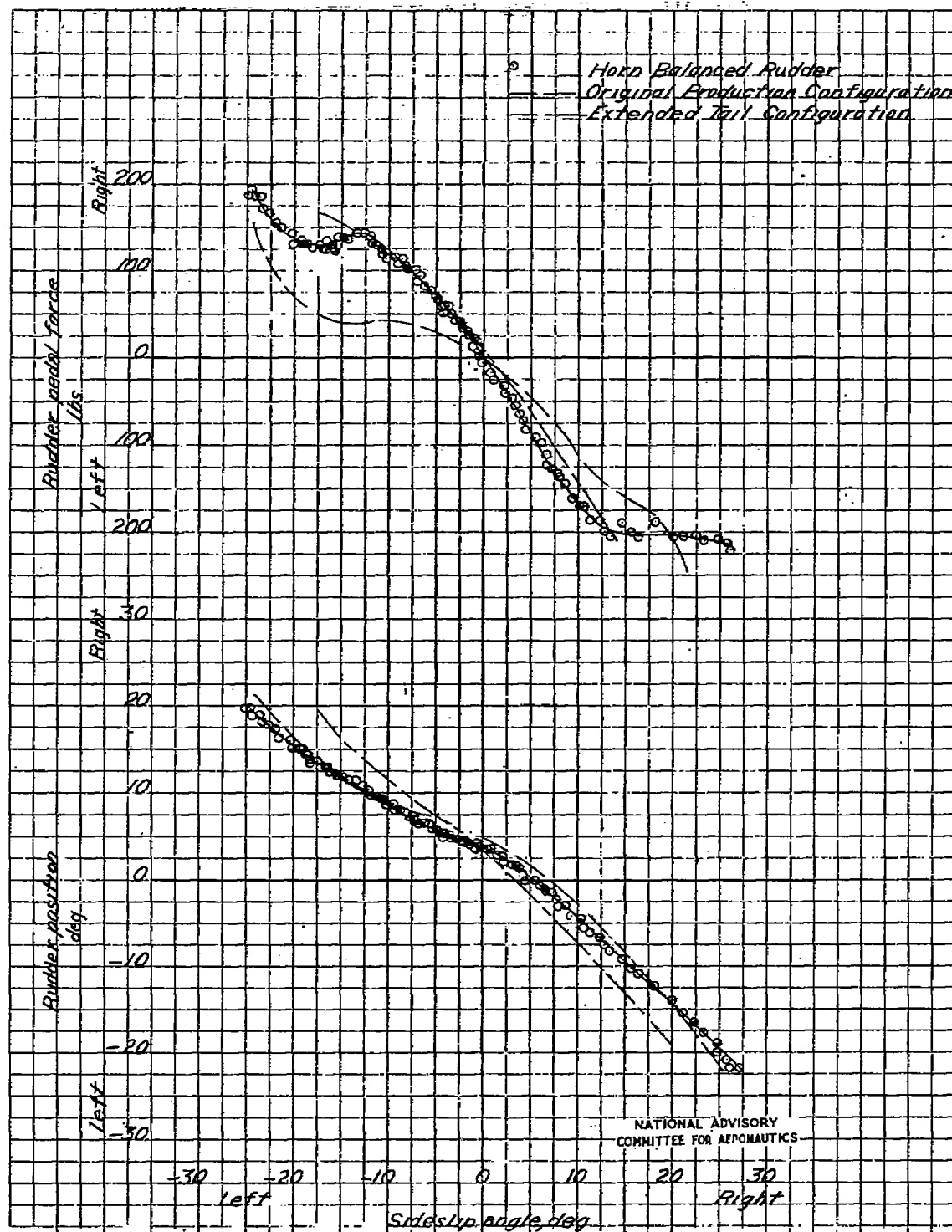
Figure 7.- Steady sideslip characteristics at 10,000 feet altitude, climbing condition V_{1s} = 200 miles per hour. P-51D-20-NA airplane with a horn balanced rudder, original and extended tail configurations.
