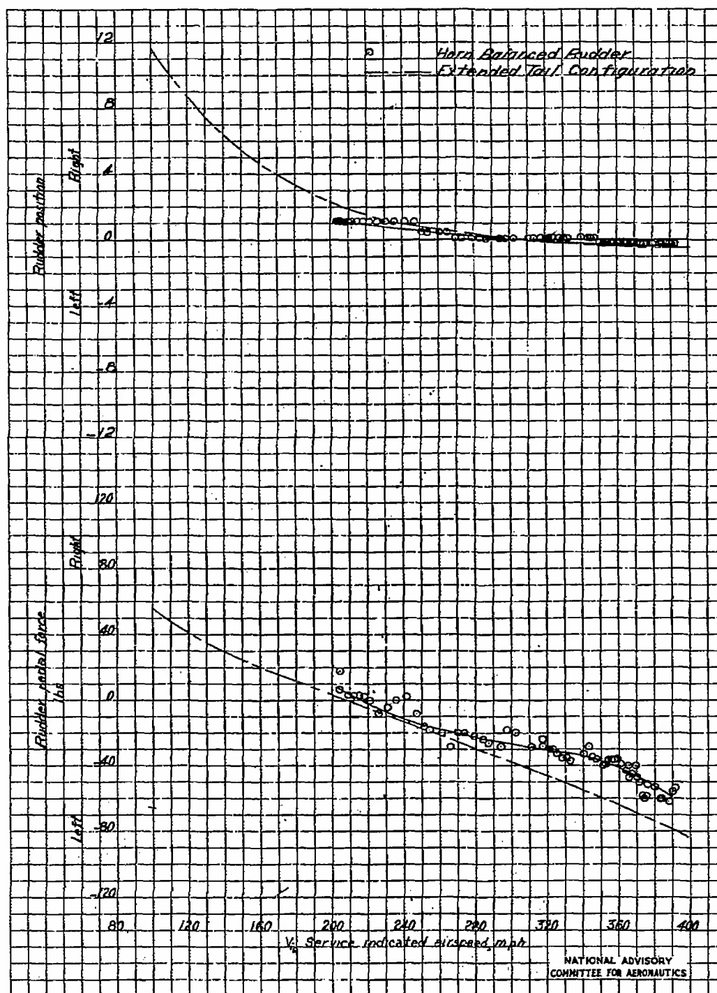
Figure 16.- Rudder trim force characteristics in a dive through the speed range from near 30,000 to 20,000 feet altitude. P-51D-20-NA airplane with a horn balanced rudder and extended tail configuration.
