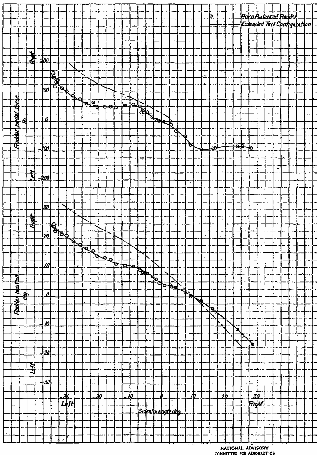
Figure 9.- Steady sideslip characteristics at 25,000 feet altitude, climbing condition V_{IS} = 100 miles per hour. P-51D-20-NA airplane with a horn balanced rudder, and extended tail configurations.
