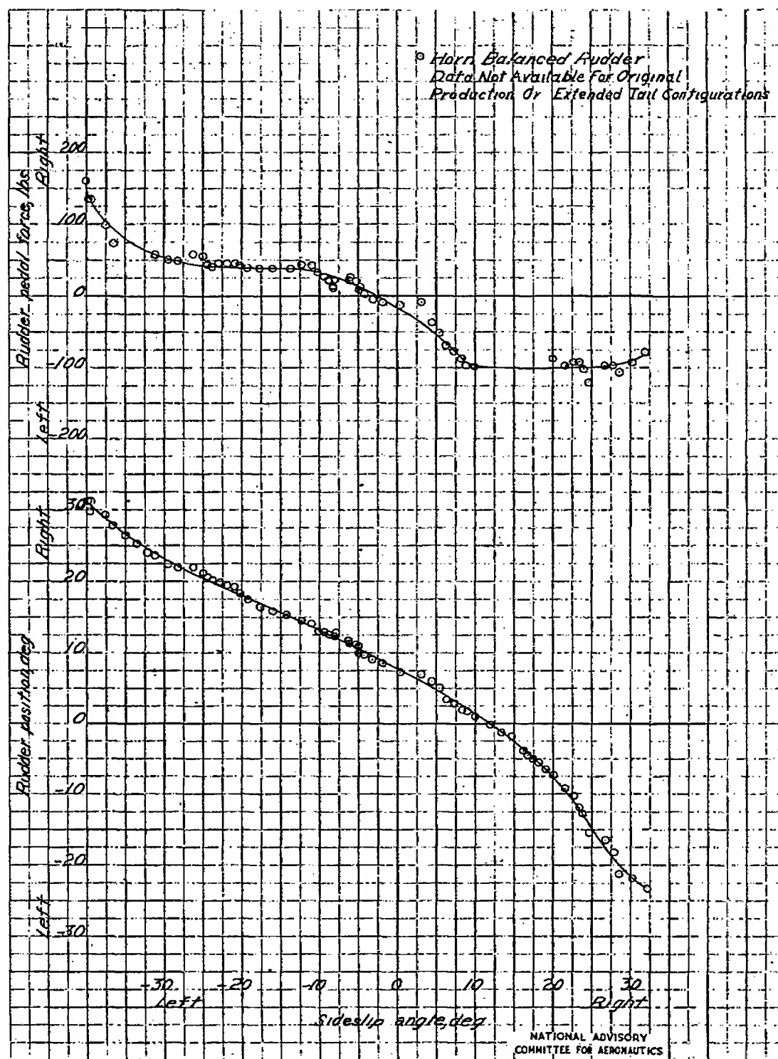
Figure 12.- Steady sideslip characteristics of 10,000 feet altitude, climbing condition V_{1S} = 103 miles per hour. P-51D-20-NA airplane with horn balanced rudder with tab locked.
