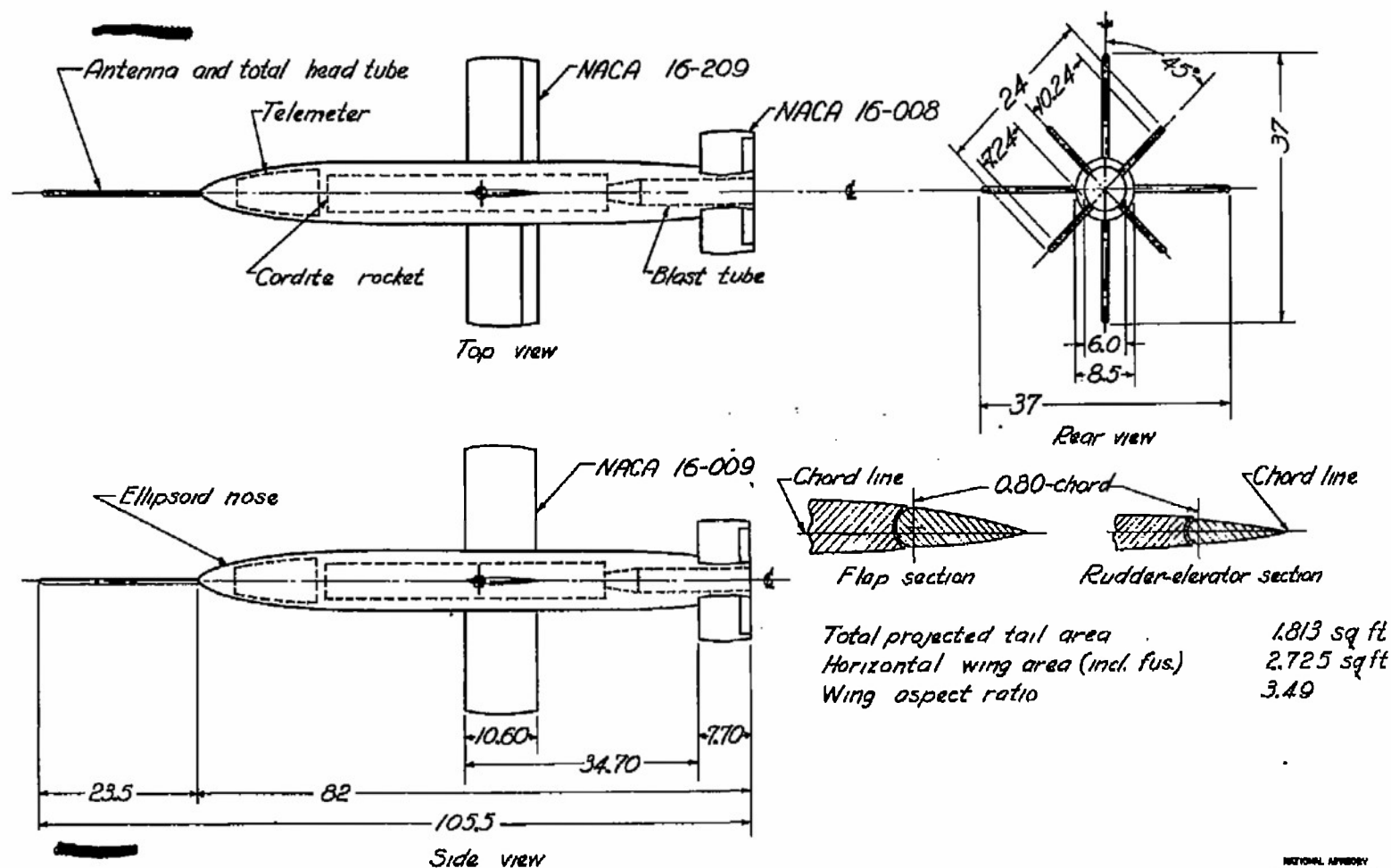
Figure 4.- General arrangement of 0.5-scale model of Fairchild Lark Pilotless Aircraft ; all dimensions in inches ; all wing and tail tips are solids of revolution.
