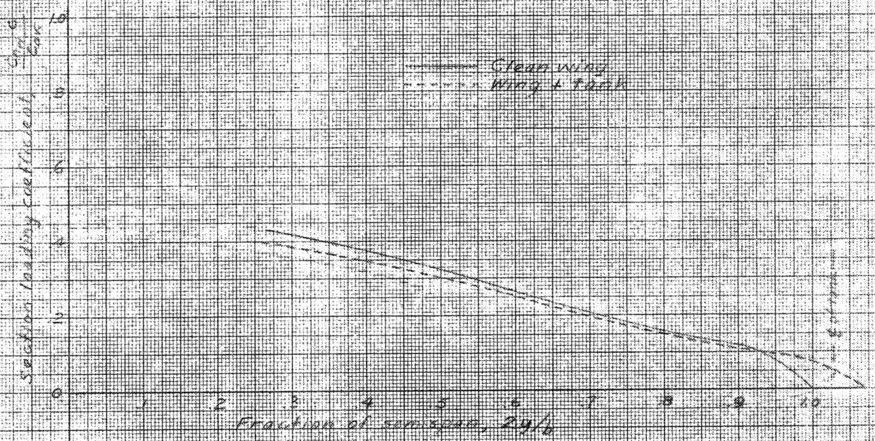
(a) Section loading coefficient
