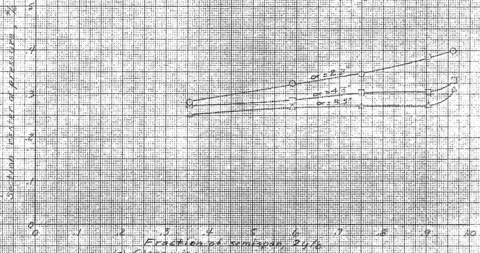
(a) Glarewing. Figure B - Spanwise center-of-pressure location on the wing for several angles of attack. Test airspeed, 126 mph; \beta, 0^\circ
