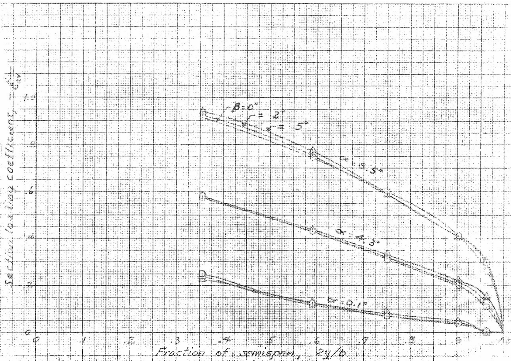
Figure 6.- Effect of sideslip on the spanwise loading of the wing at several angles of attack. Test airspeed, 124 mph.
