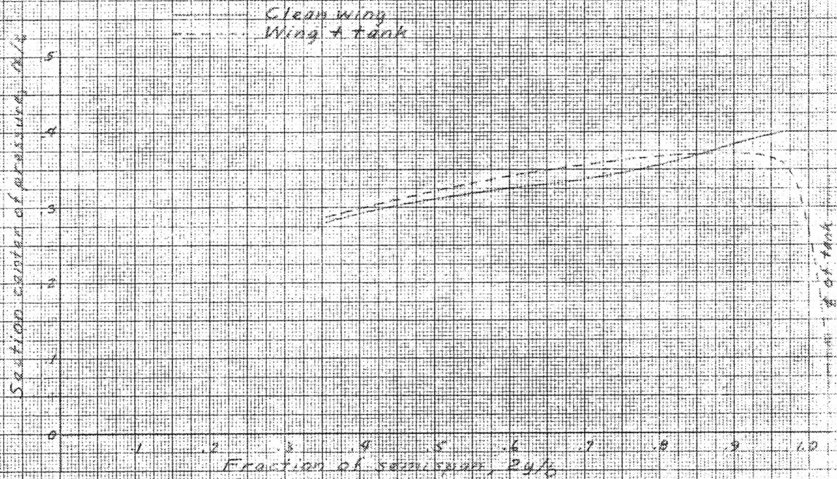
(b) Section center-of-pressure location.
