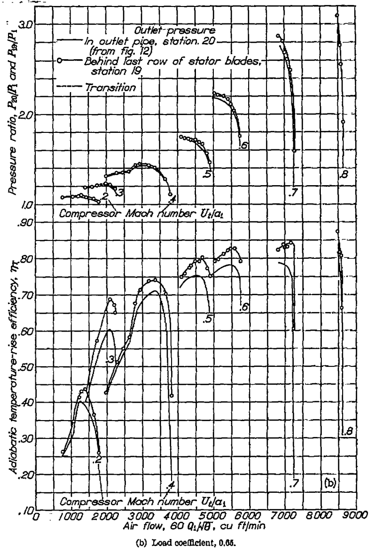
FIGURE 21.—Concluded. Comparison of performance characteristics of axial-flow compressor based on total-pressure measurements in outlet pipe and behind last row of stator blades. Stator blades reset for 75 percent of design speed.
