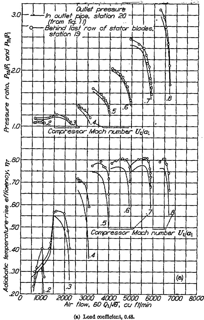
FIGURE 21.—Comparison of performance characteristics of axial-flow compressor based on total-pressure measurements in outlet pipe and behind last row of stator blades. Stator blades reset for 75 percent of design speed.
