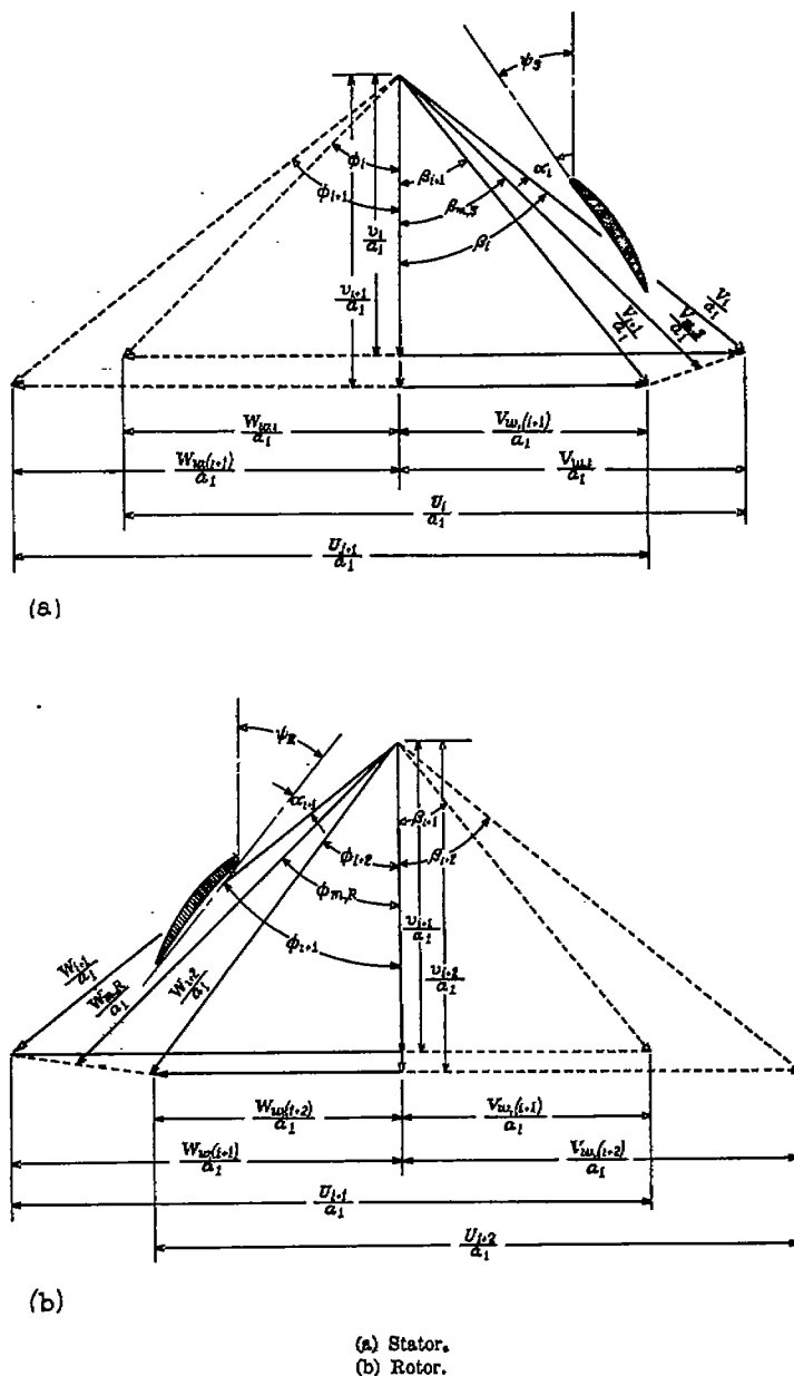
FIGURE 7.—Velocity diagram for typical stage of axial-flow compressor.
