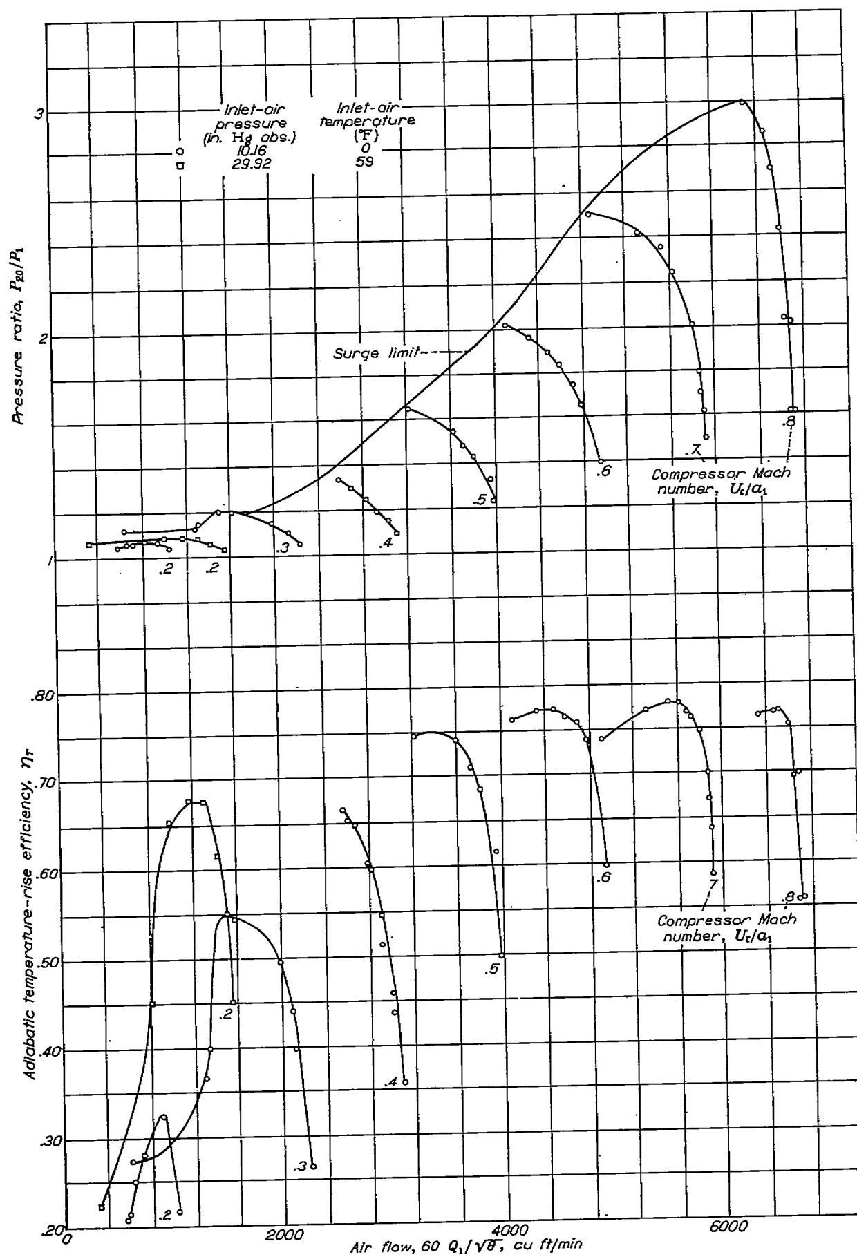
FIGURE 11.—Performance characteristics of axial-flow compressor with stator blades reset for 75 percent of design speed and load coefficient of 0.49.
