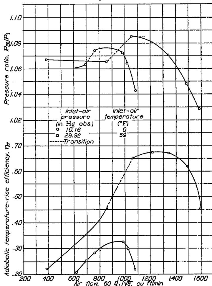
FIGURE 17.—Performance of axial-flow compressor with reset stator blades at compressor Mach number of 0.2 showing effect of inlet-air conditions and range within which transition occurs.
