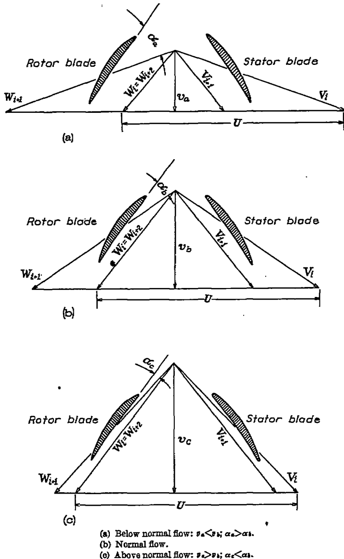
FIGURE 3.—Effect of flow on angle of attack for typical stage of axial-flow compressor.
