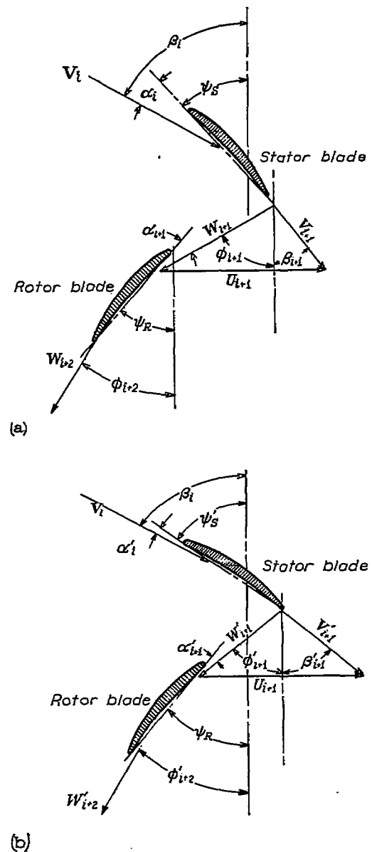
FIGURE 4.—Effect of change in stator-blade angle on angles of attack for stator blades and following rotor blades.
