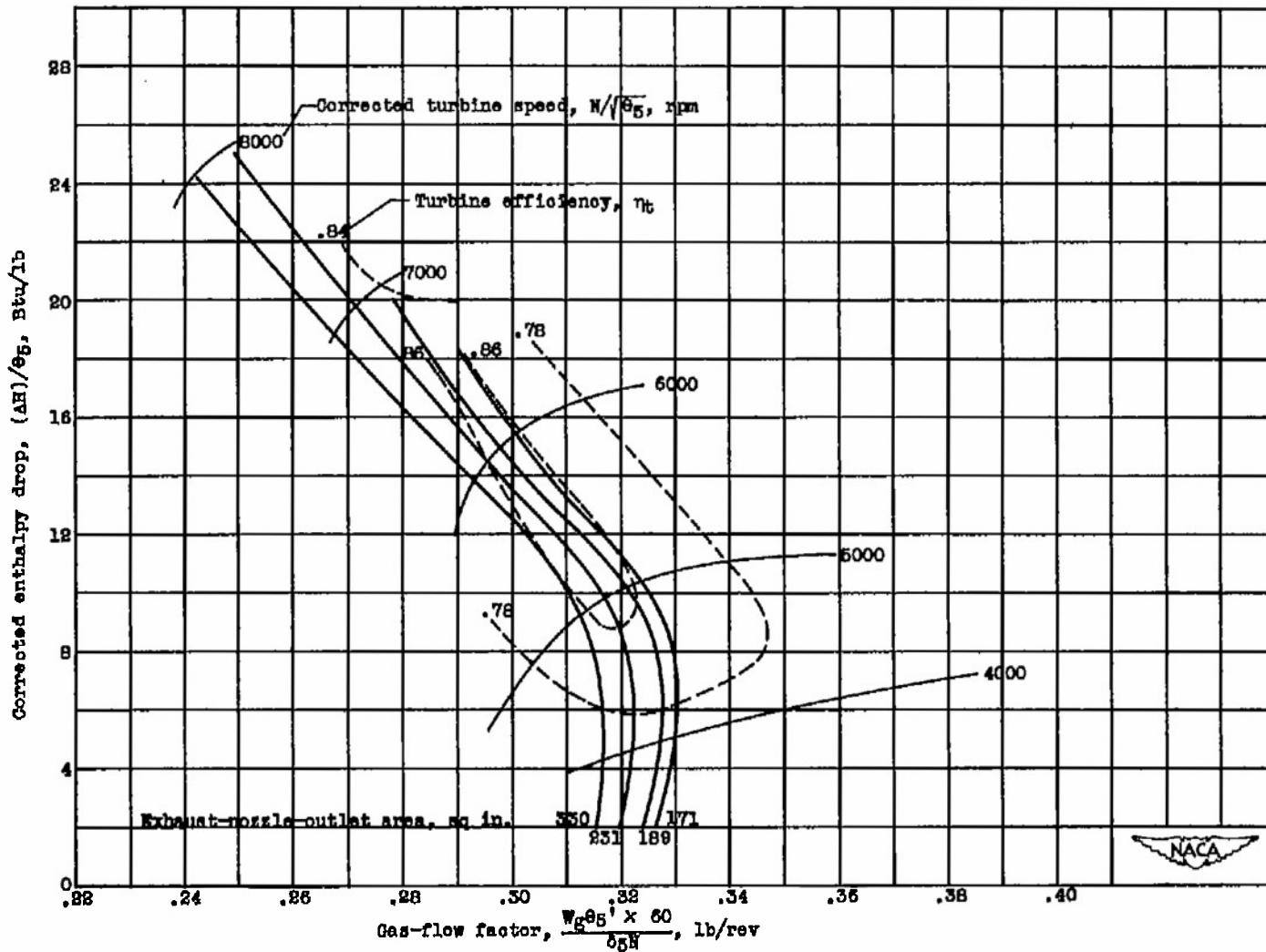
(c) Turbine operating lines for various exhaust-nozzle-outlet areas. Altitude, 25,000 feet; flight Mach number, 0.55.
