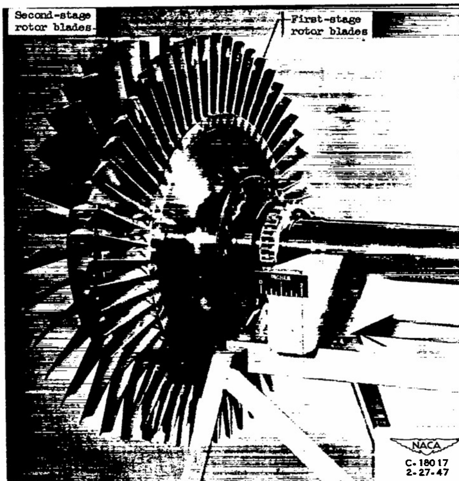
Figure 4. - Turbine-rotor assembly.
