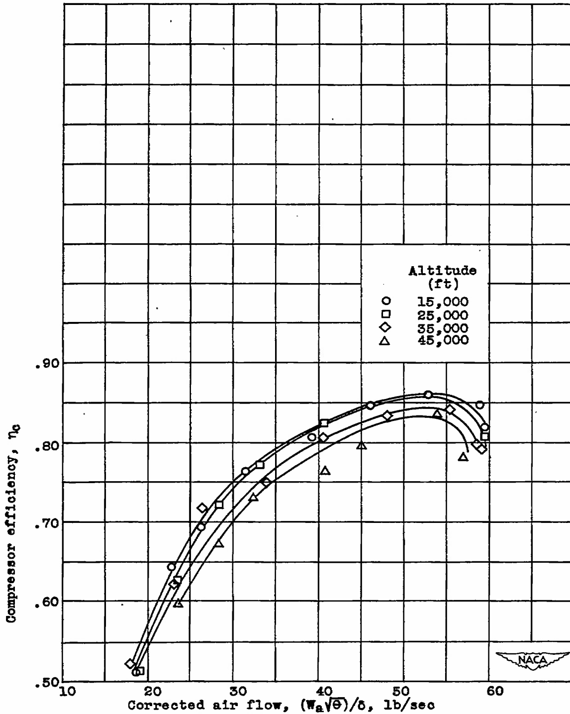
Figure 15. - Relation between compressor efficiency and corrected air flow for modified compressor at various altitudes. Flight Mach number, 0.53; exhaust-nozzle-outlet area, 171 square inches.
