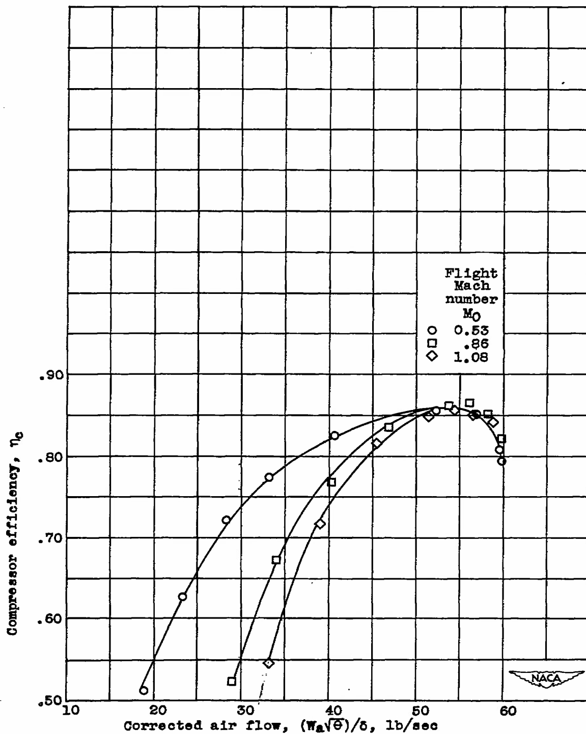
Figure 17. - Relation between compressor efficiency and corrected air flow for modified compressor at various flight Mach numbers. Simulated altitude, 25,000 feet; exhaust-nozzle-outlet area, 171 square inches.
