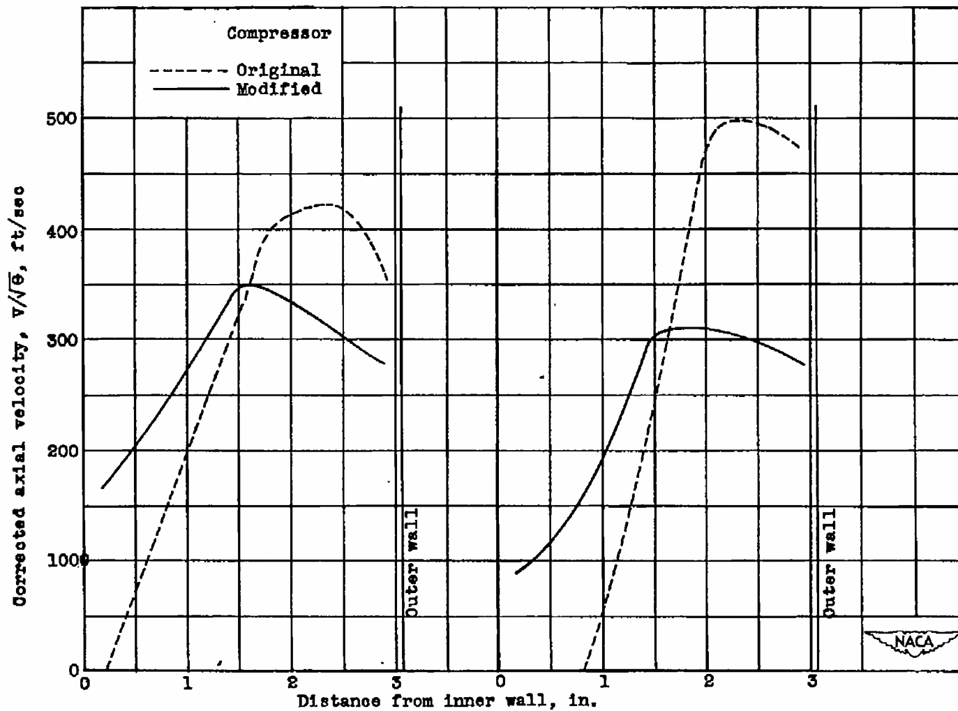
Figure 12. - Radial distribution of corrected axial velocity at outlet of original and modified compressors. Corrected engine speed, 12,000 rpm; flight Mach number, 0.53.
