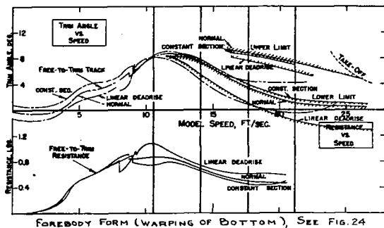
FOREBODY FORM (WARPING OF BOTTOM), SEE FIG. 24
