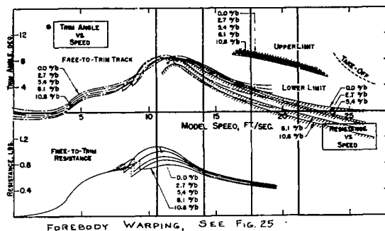
FOREBODY WARPING, SEE FIG. 25
