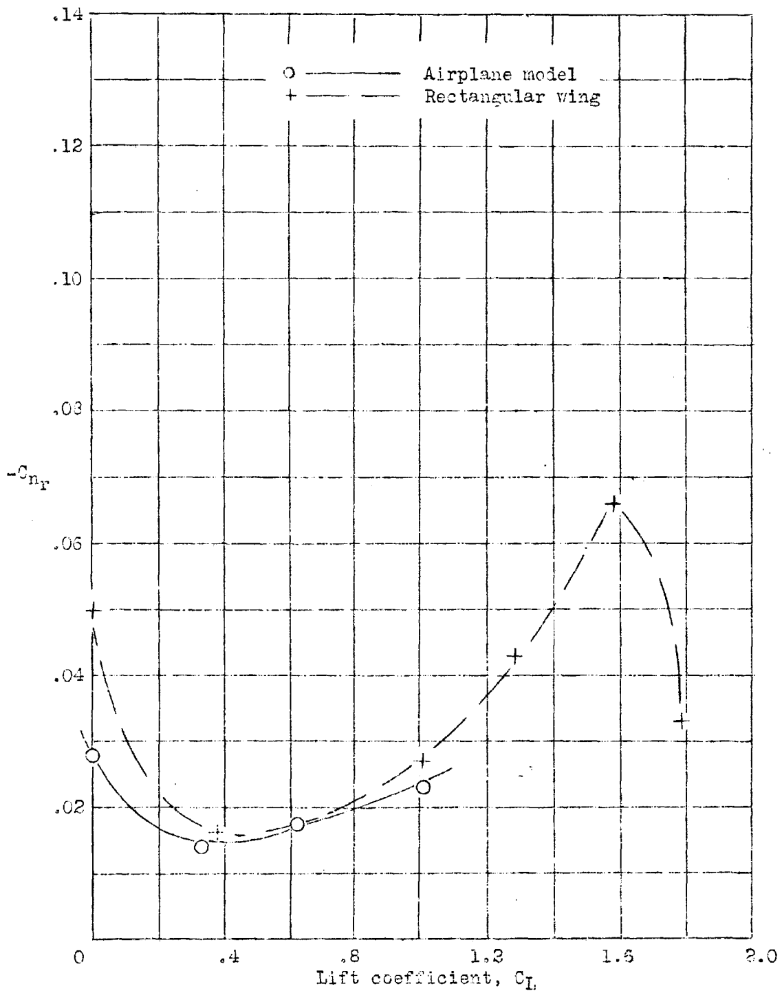
Figure 4.- Variation of damping in yaw with lift coefficient. Flaps extended; vertical tail removed.
