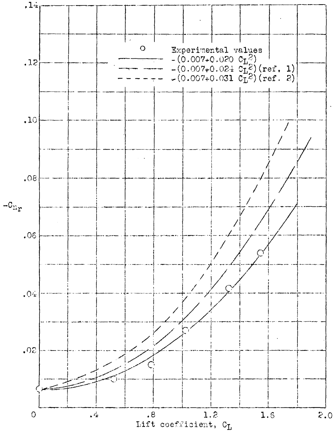
Figure 5.- Variation of damping in yaw with lift coefficient. Rectangular wing; flaps retracted.
