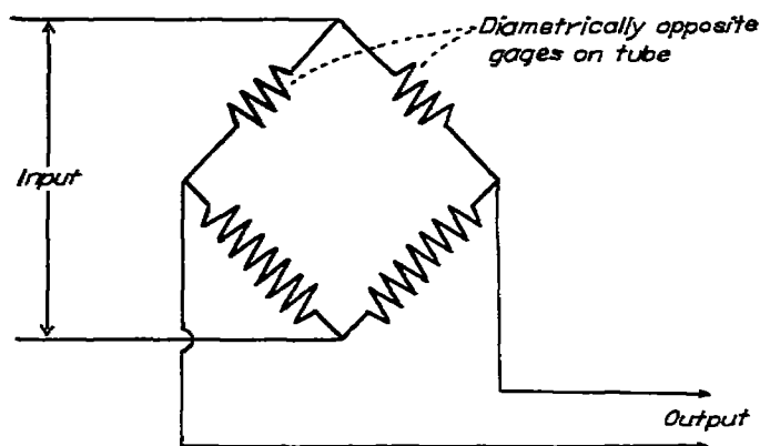
FIGURE 8.—Bridge circuit used in tests.
