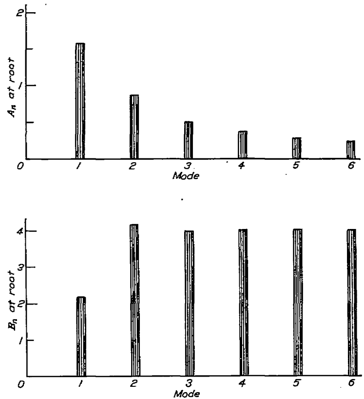
FIGURE 4.—Values of bending-stress coefficient A_n and shear-stress coefficient B_n at root.
