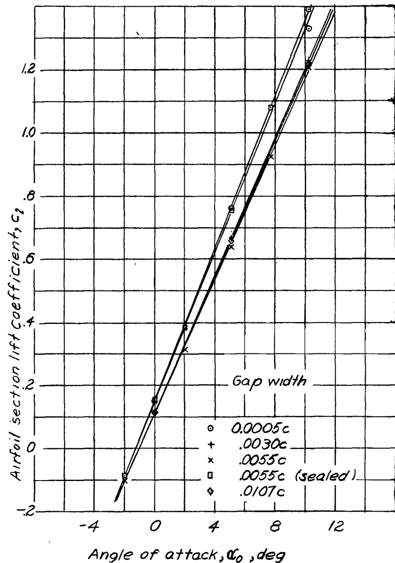
Figure 19.- Effect of variation of gap width on slope of lift curve, \delta_a = 0^\circ . Nose radius = .002c; Mach number = 0.417
