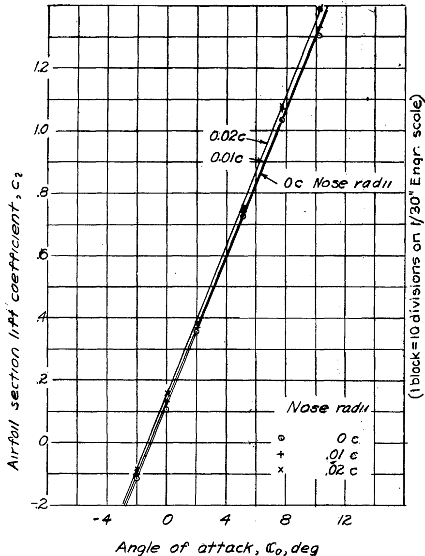
Figure 20.- Effect of variation of aileron nose radius on slope of lift curve, \delta_a = 0^\circ . Gap width = .0055c sealed; Mach number = 0.417
