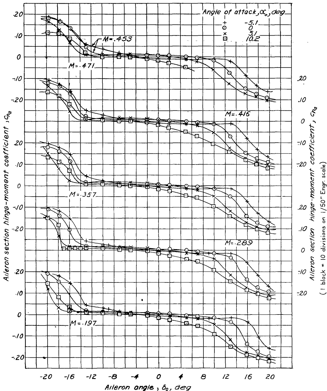
Figure 5.—Variation of aileron section hinge-moment coefficient with aileron angle. Nose radius = 0.01c ; gap width = 0.0053c .
