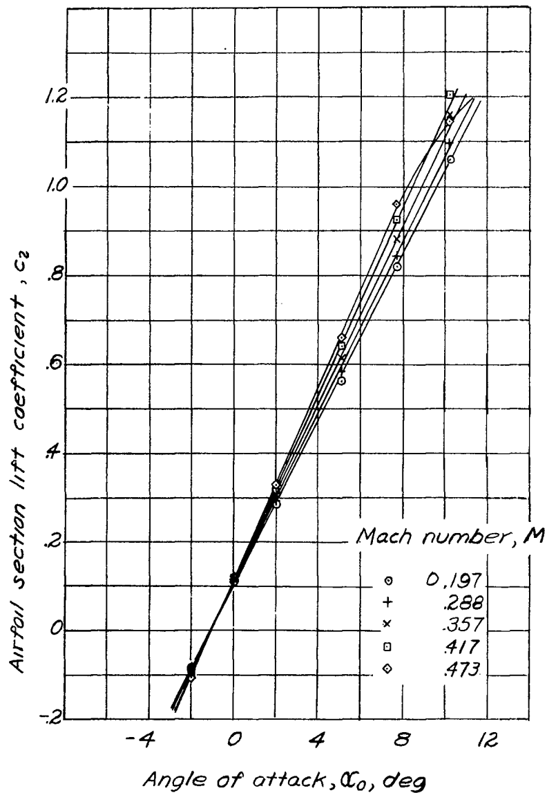
Figure 17.- Effect of variation of Mach number on slope of lift curve, \delta_a = 0^\circ . Nose radius = 0.02c ; gap width = 0.0055c .
