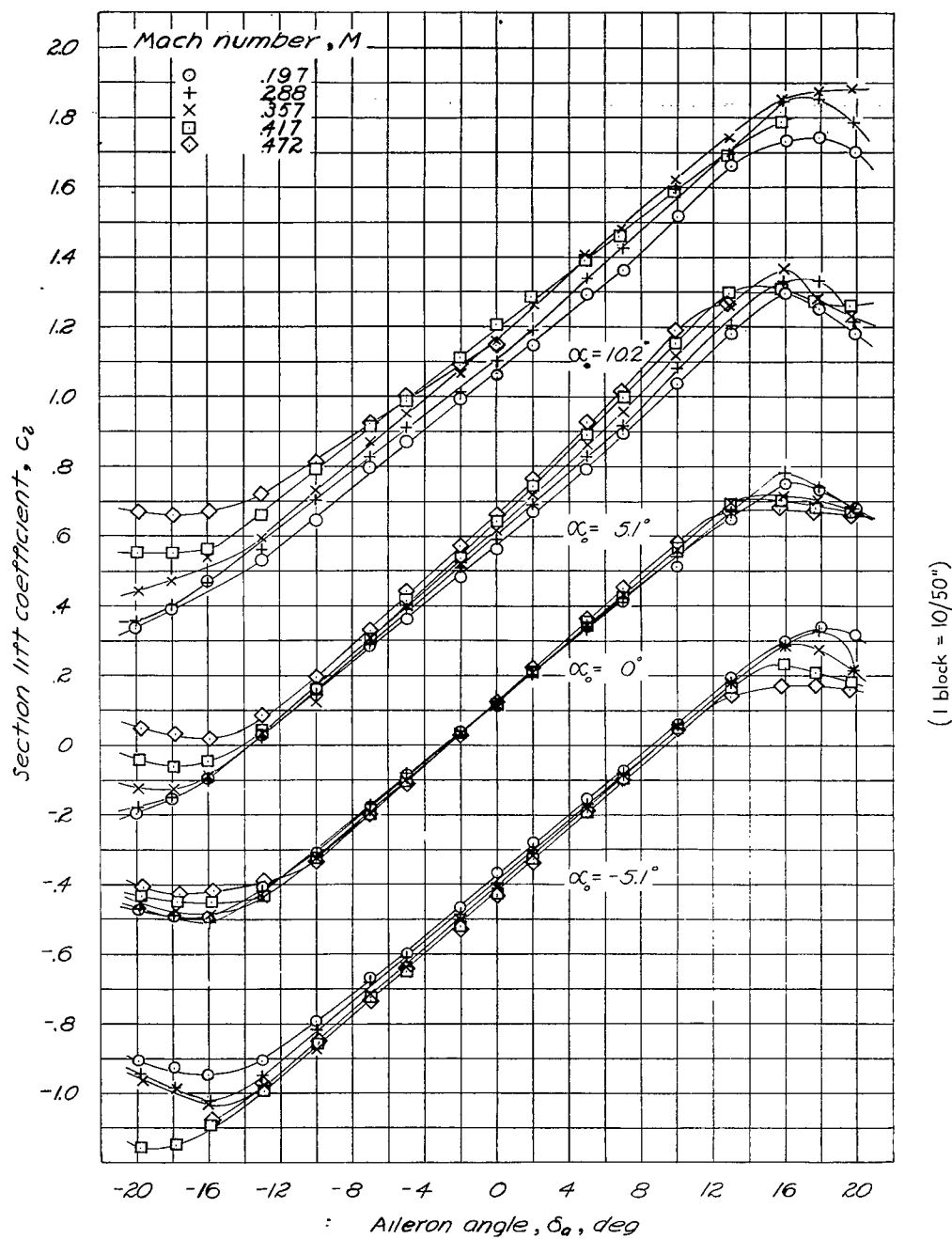
Figure 25.- Variation of section lift coefficient with aileron angle. Nose radii = 0.02c ; gap width = 0.0055c .
