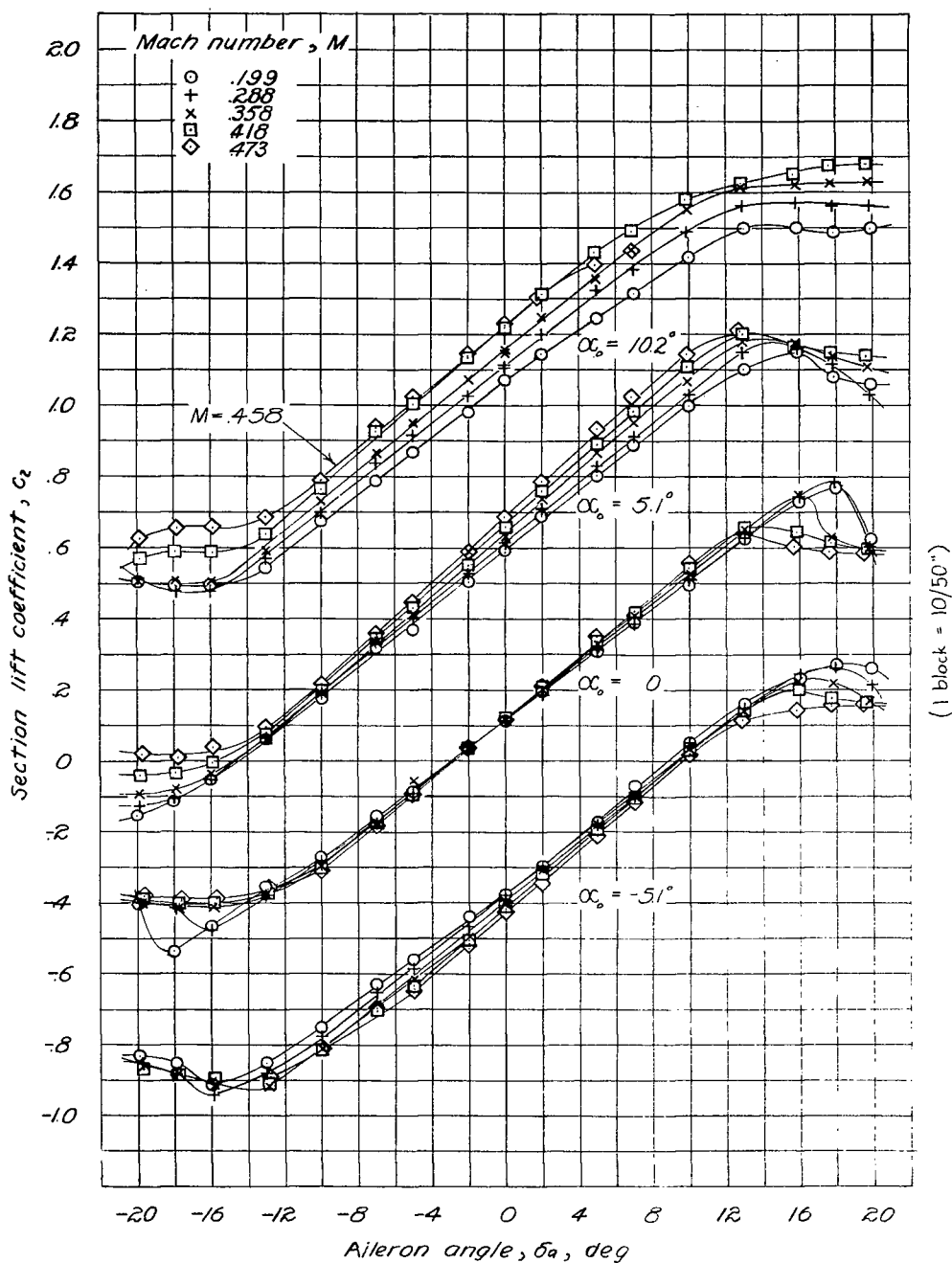
Figure 27.- Variation of section lift coefficient with aileron angle. Nose radii = 0.02c ; gap width = 0.0127c .
