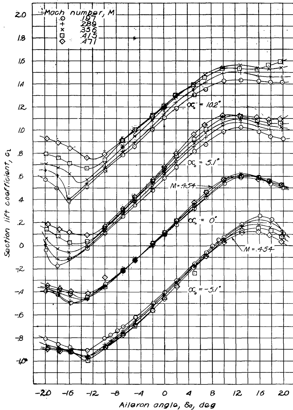
Figure 22:- Variation of section lift coefficient with aileron angle. Nose radii = 0.01c , gap width = 0.0035c .
