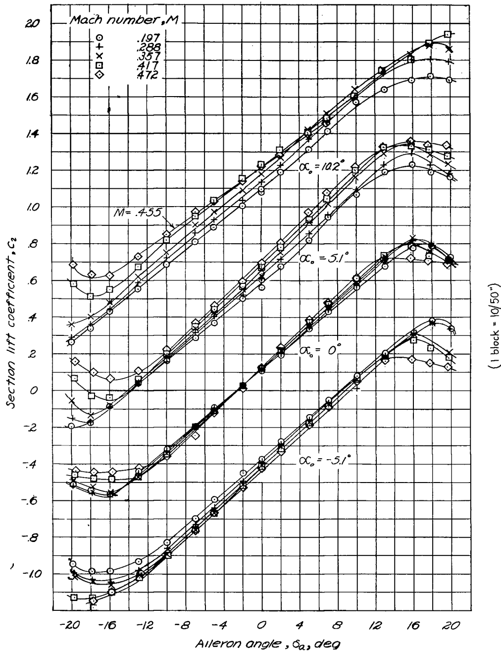
Figure 24.-Variation of section lift coefficient with aileron angle. Nose radii = 0.02c ; gap width = 0.0030c .
