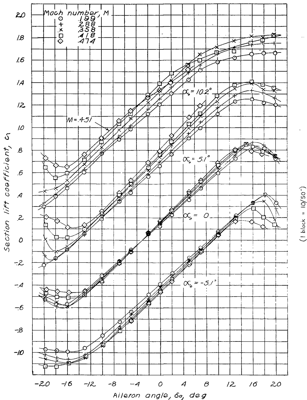
Figure 26.- Variation of section lift coefficient with aileron angle. Nose radii=0.02c; gap width = 0.0055c sealed.
