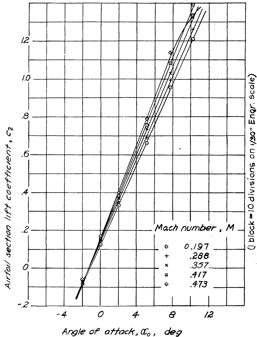
Figure 18.- Effect of variation of Mach number on slope of lift curve, \delta_a = 0^\circ . Nose radius = 0.02c ; gap width = 0.0055c (sealed).
