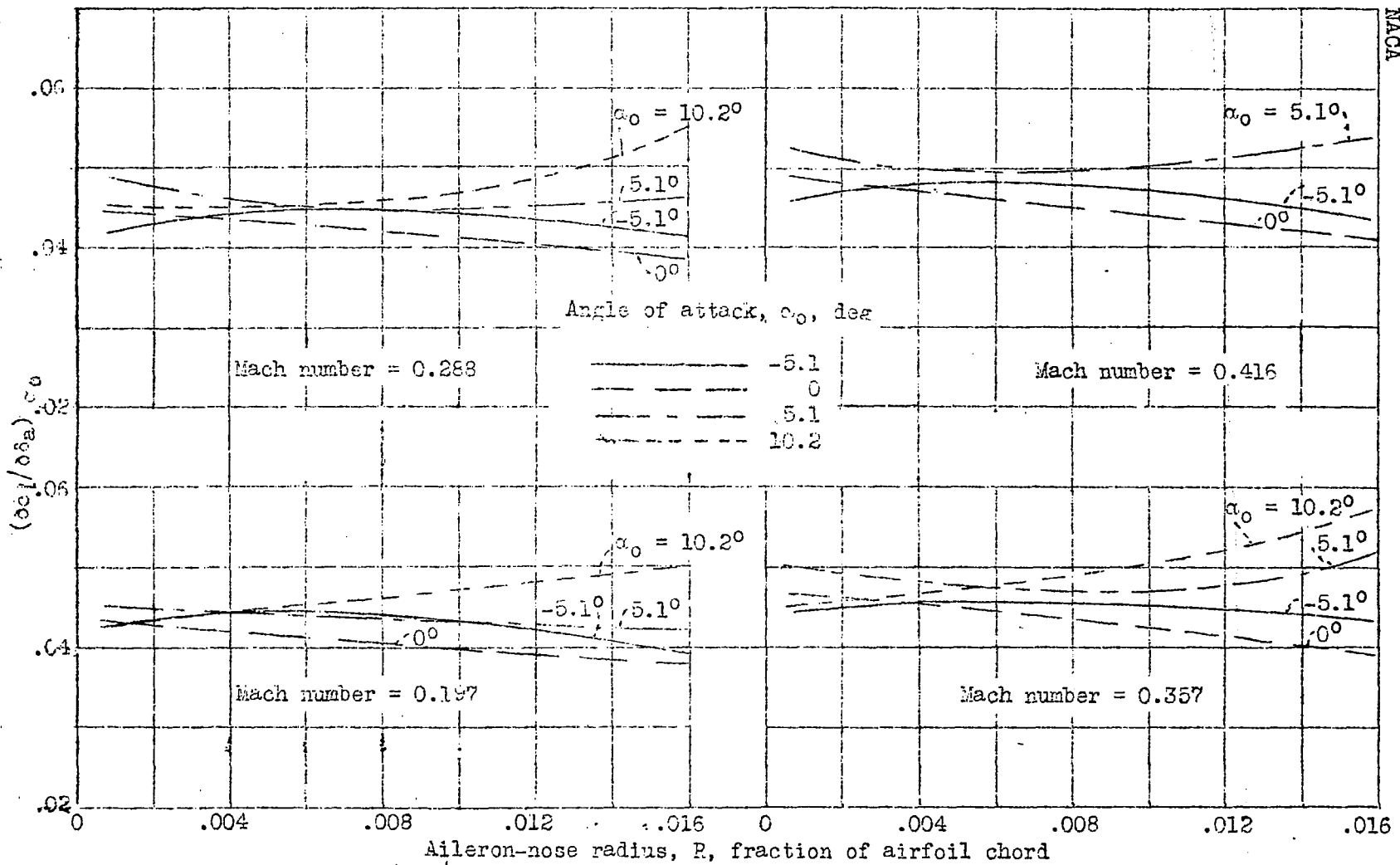
Figure 20.- Variation of (\partial c_l / \partial \delta_a)_{\alpha_0} with aileron nose radius. Lower-surface radius = 0; vent gap = 0.0055c.
