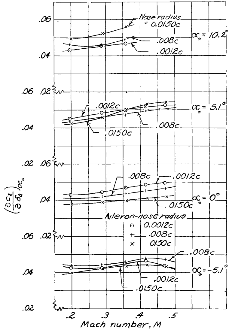
(a) Lower-surface radius = 0; vent gap = 0.0055c.
