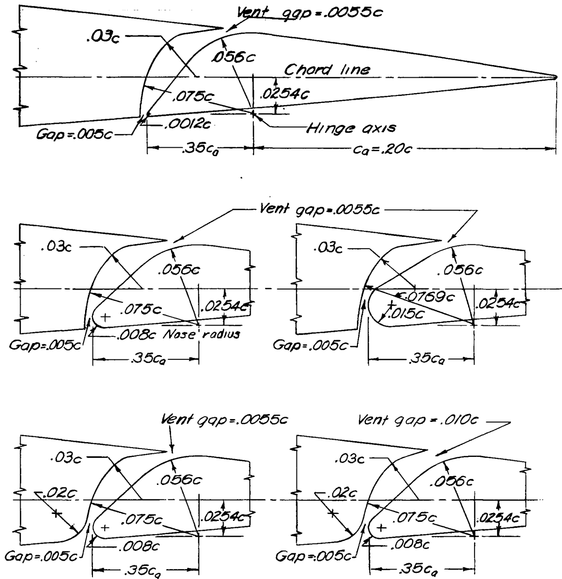
Figure 2.- Dimensions of Frise ailerons.
