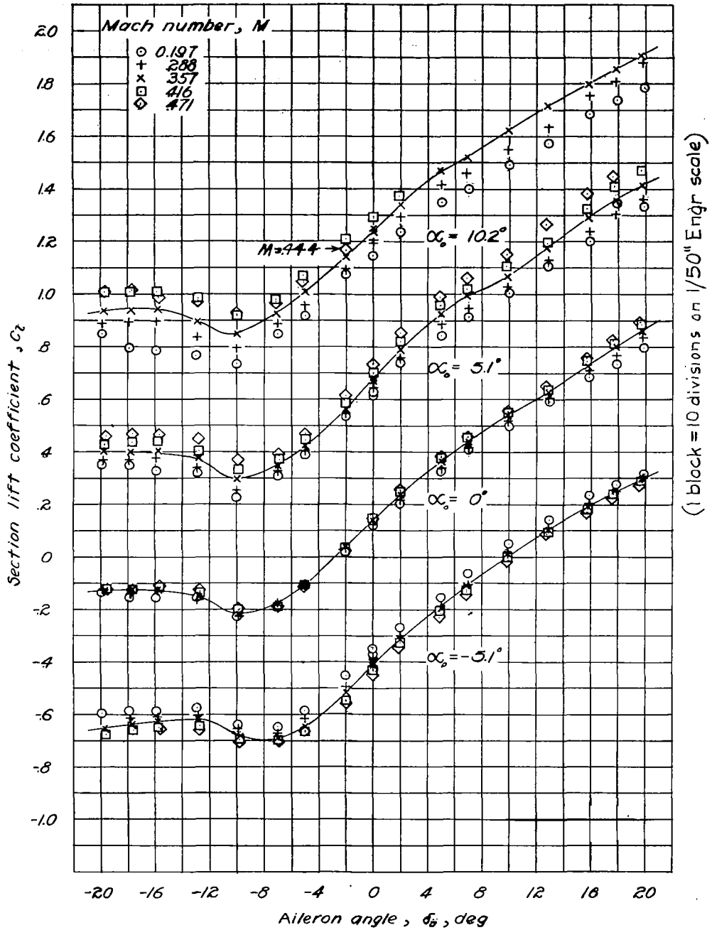
Figure 14.- Variation of section lift coefficient with aileron angle. Aileron-nose radius = 0.0012c; lower-surface radius = 0; vent gap = 0.0055c.
