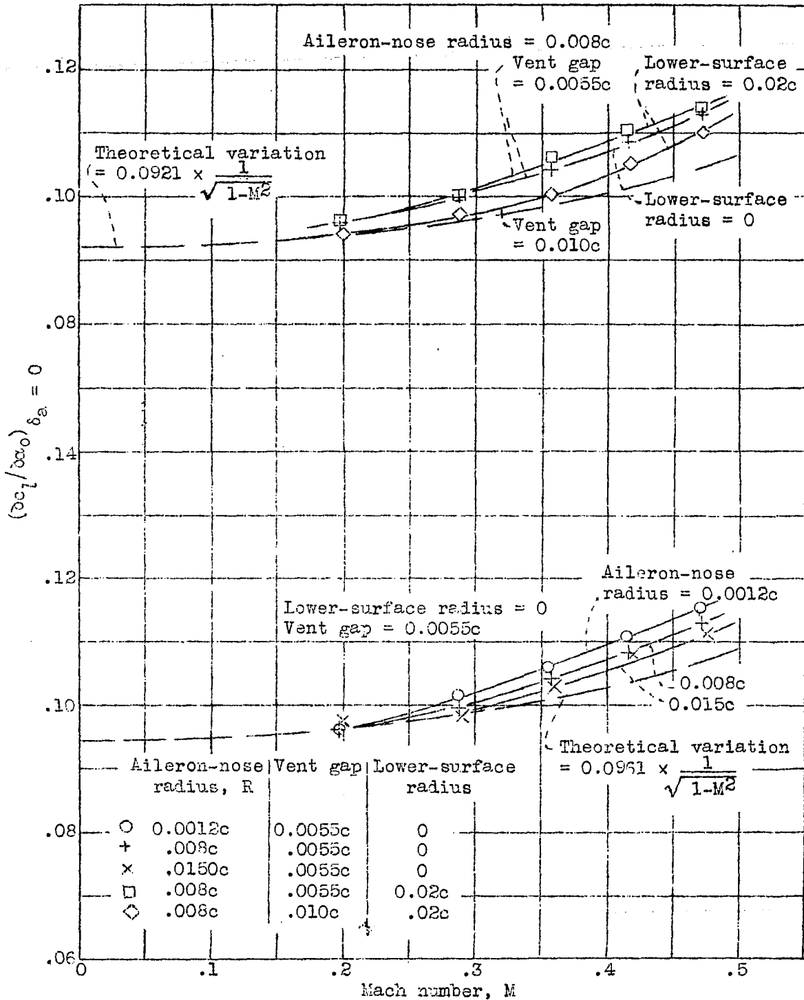
Figure 13.- Variation of lift-curve slope with Mach number, \delta_a = 0 .
