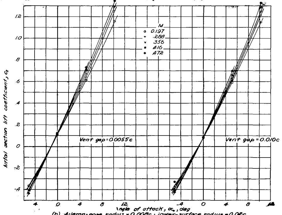
Figure 12a- Concluded. (b) Aileron-nose radius = 0.008c; lower-surface radius = 0.02c.
