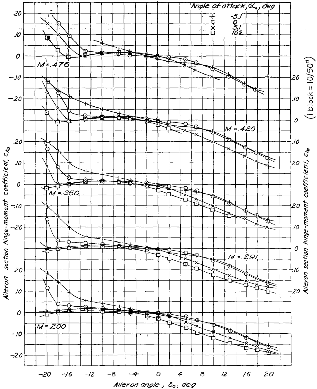
Figure 7. —Variation of aileron section hinge-moment coefficient with aileron angle. Aileron-nose radius = 0.0150c; lower-surface radius = 0; vent gap = 0.0055c.
