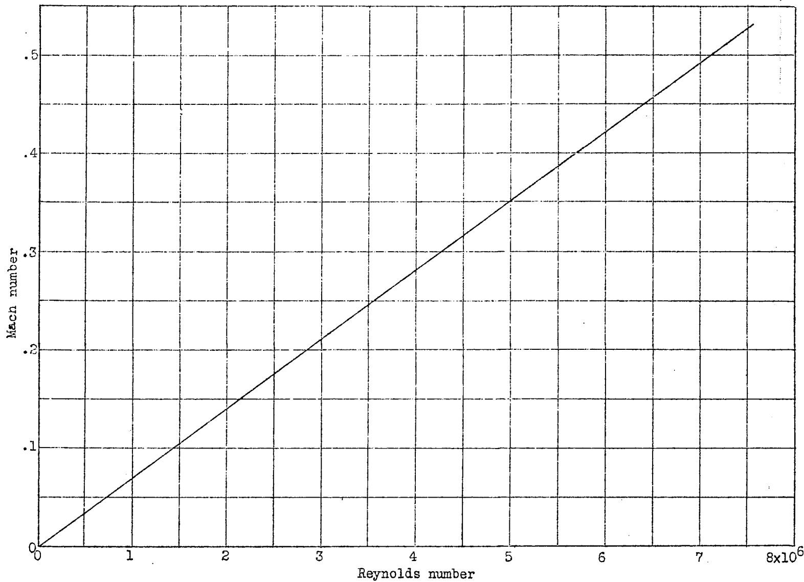
Figure 3.- Variation of test Mach number with Reynolds number, based on standard atmosphere, for a 2-foot chord airfoil in the 2.5-by 6-foot test section of the stability tunnel.
