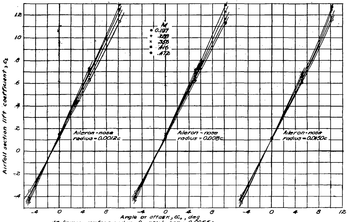
Figure 12- Variation of section lift coefficient with angle of attack, \delta_2 = 0 . Lower-surface radius = 0; vent gap = 0.0055c.
