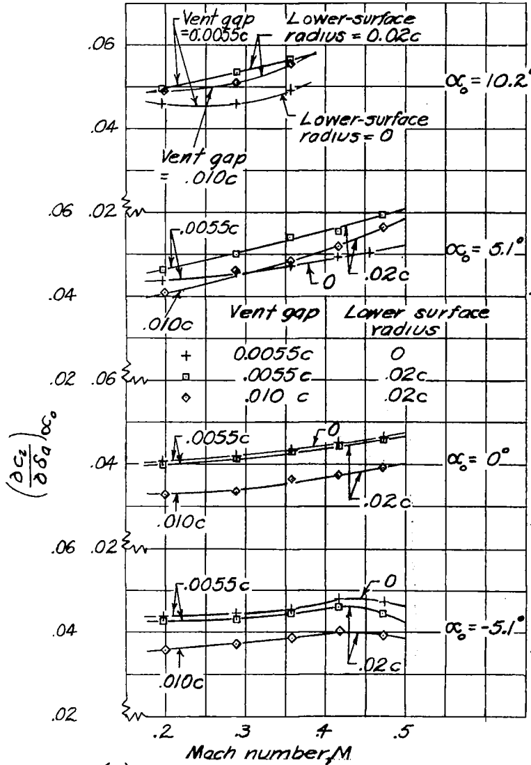
(b) Aileron-nose radius = 0.008c.
