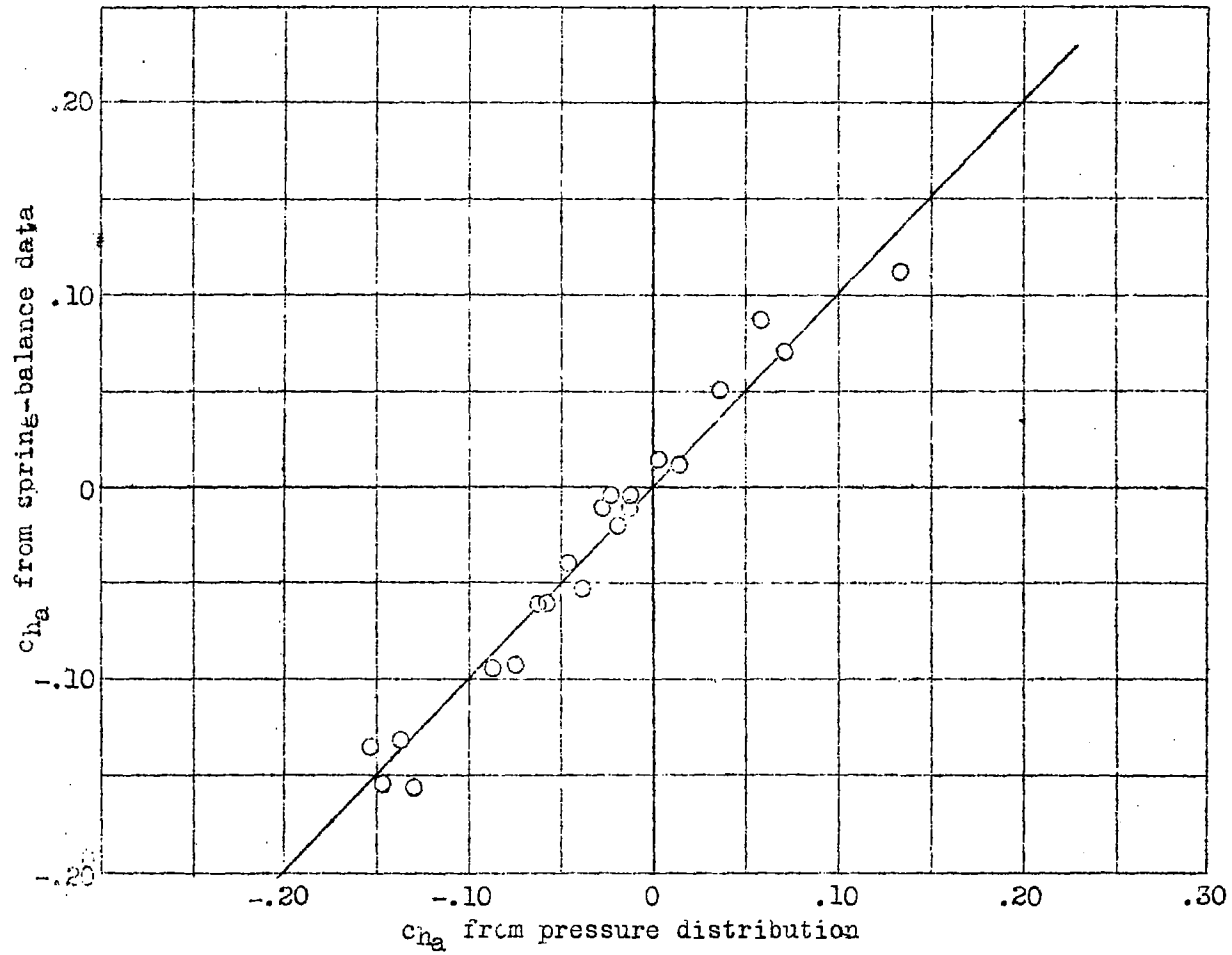
Figure 4.- Comparison of hinge-moment coefficients obtained from spring-balance data with those obtained from pressure distribution.
