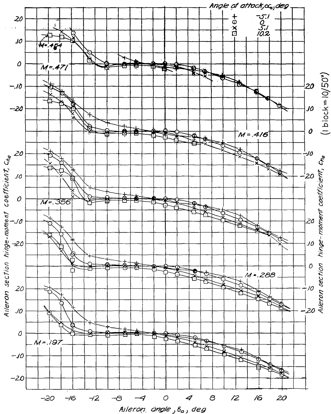
Figure 8. — Variation of aileron section hinge-moment coefficient with aileron angle Aileron-nose radius = 0.008c; lower-surface radius = 0.02c; vent gap = 0.0055c.
