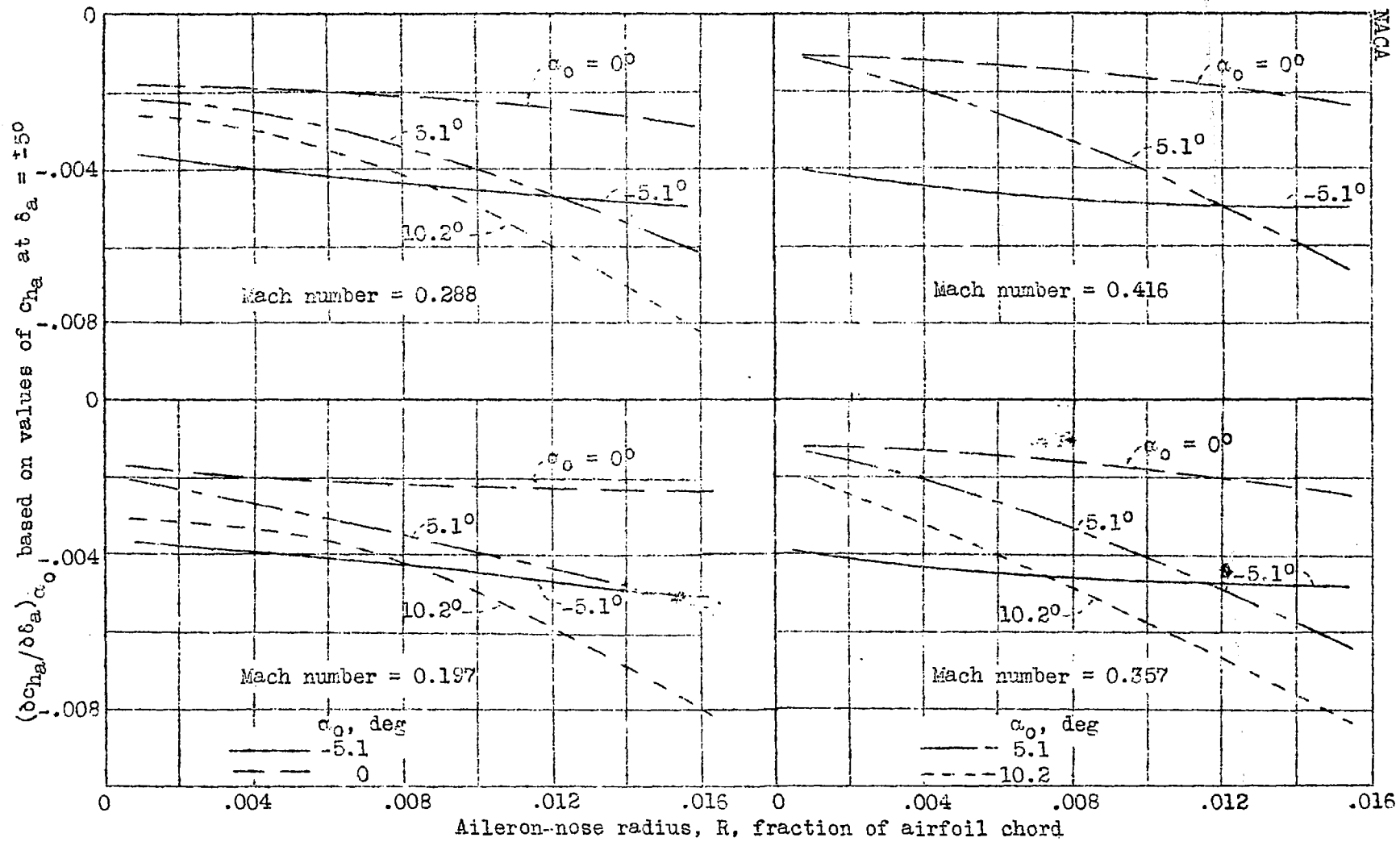
Figure 11.- Variation of (\partial c_{ha} / \partial \delta a)_{\alpha_0} with aileron-nose radius. Lower-surface radius = 0; vent gap = 0.0055c.
