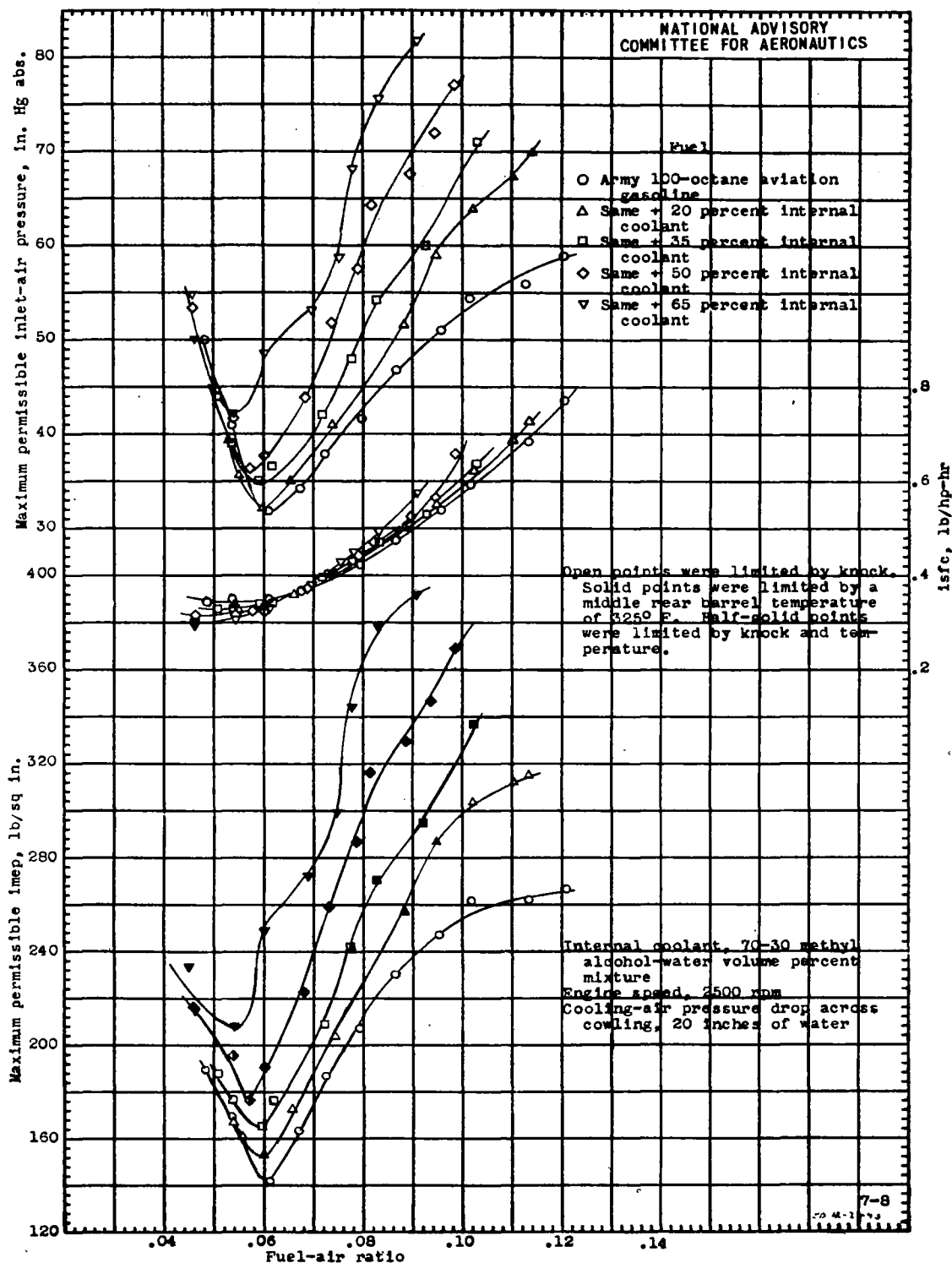
Figure 8. - Engine performance permitted with a mixture of methyl alcohol and water as an internal coolant at an engine speed of 2500 rpm and a cooling-air pressure drop across cooling of 20 inches of water. Wright C9GC cylinder; compression ratio, 7.0; spark advance, 20° B.T.C.; inlet-air temperature, 250° F; cooling-air upstream temperature, 125° F; fuel, Army 100-octane aviation gasoline.
