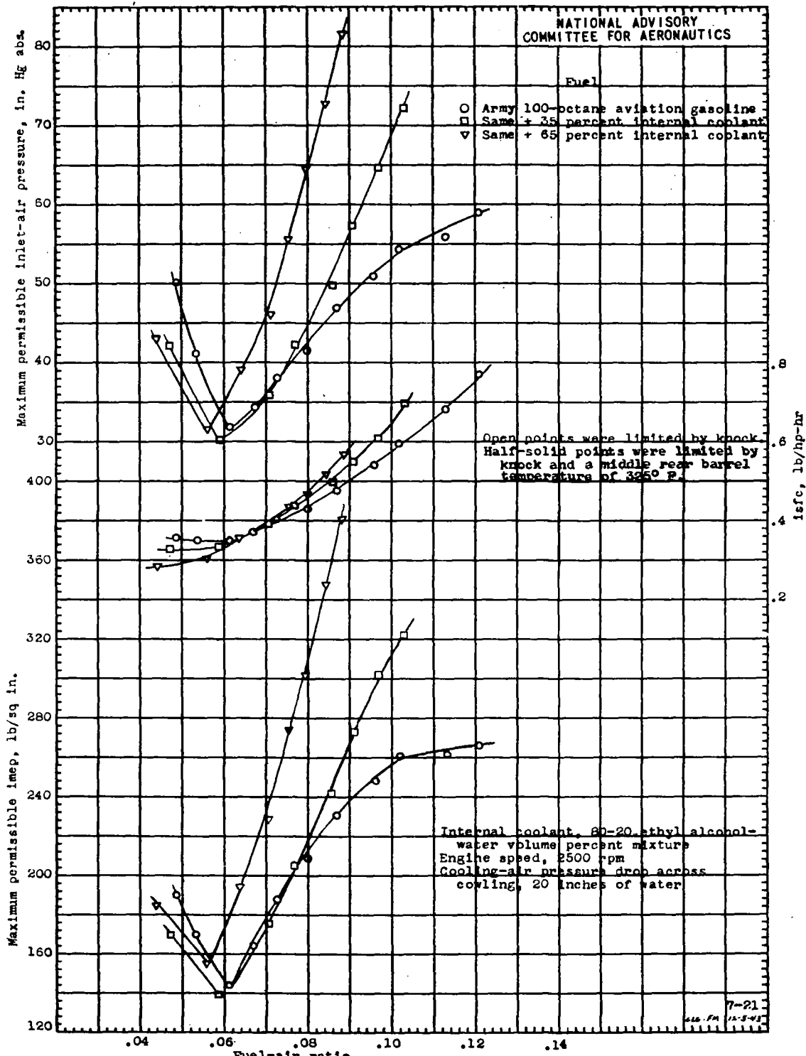
Figure 9. - Engine performance permitted with a mixture of ethyl alcohol and water as an internal coolant at an engine speed of 2500 rpm and a cooling-air pressure drop across cowling of 20 inches of water. Wright C90C cylinder; compression ratio, 7.0; spark advance, 20° B.T.C.; inlet-air temperature, 250° F; cooling-air upstream temperature, 125° F; fuel, Army 100-octane aviation gasoline.
