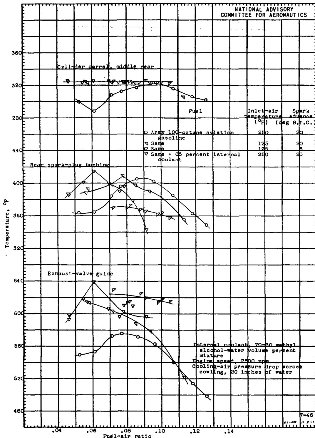
Figure 25. - Effect of spark advance, inlet-air temperature, and internal coolant on representative engine temperatures at maximum permissible inlet-air pressure at an engine speed of 2500 rpm and a cooling-air pressure drop across cowling of 20 inches of water. Wright C9GC cylinder; compression ratio, 7.0; cooling-air upstream temperature, 125° F; fuel, Army 100-octane aviation gasoline.
