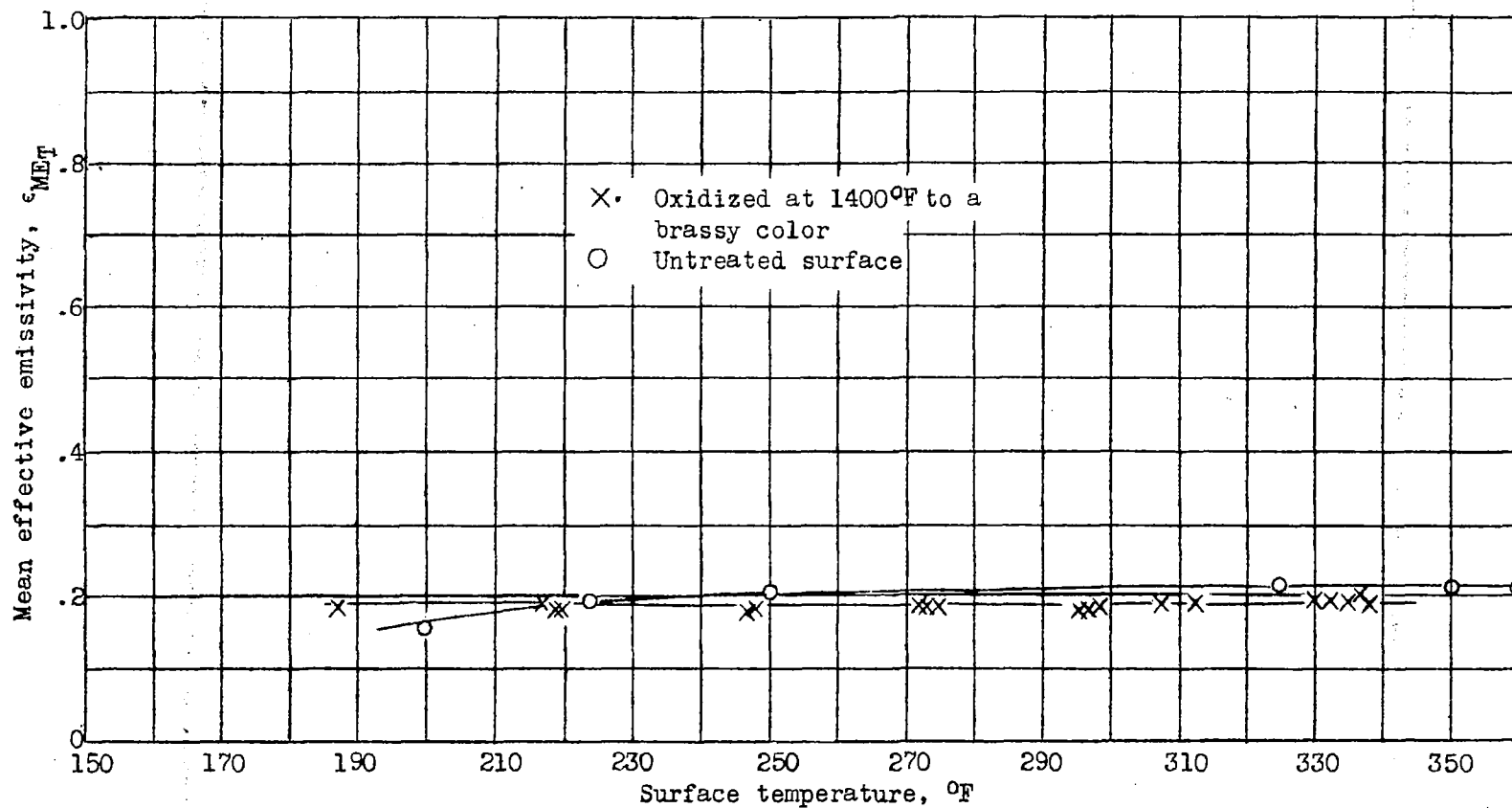
Figure 2.- Emissivity of Inconel as a function of temperature. (Measured in a direction perpendicular to the plane of the surface)..
