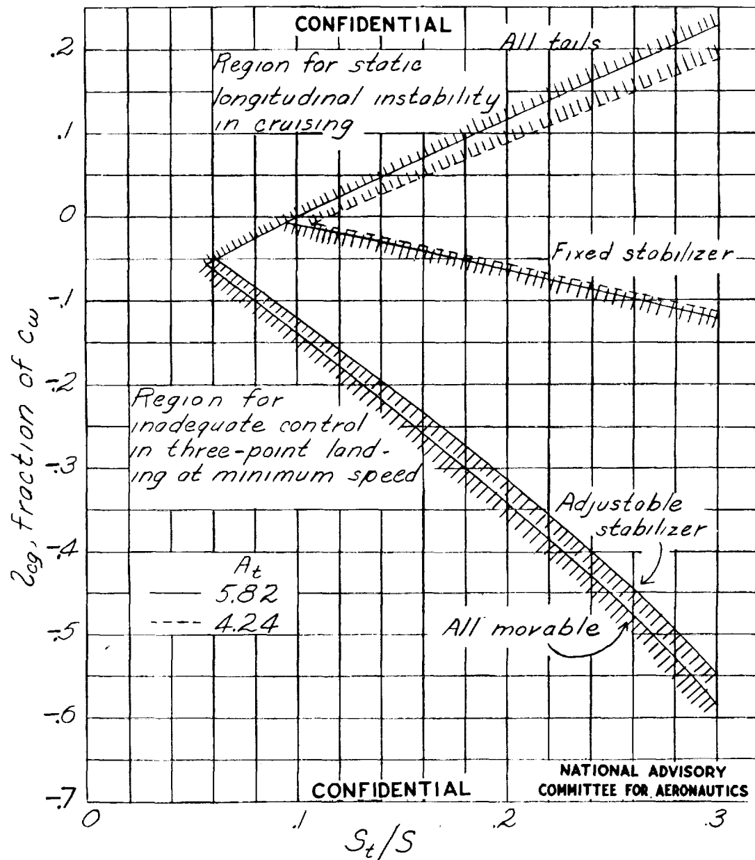
Figure 2.- Variation with horizontal-tail area of permissible center-of-gravity positions for fixed-stabilizer, adjustable-stabilizer, and all-movable horizontal tails.
