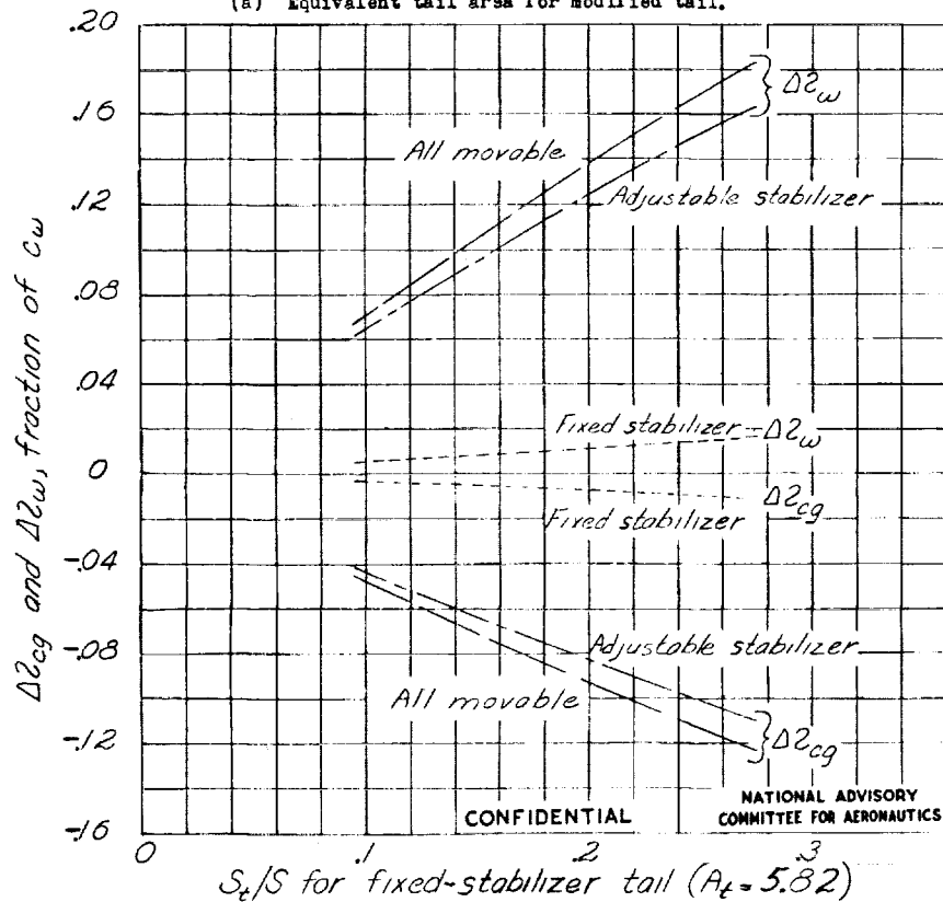
(b) Required movements of center-of-gravity or wing position.
