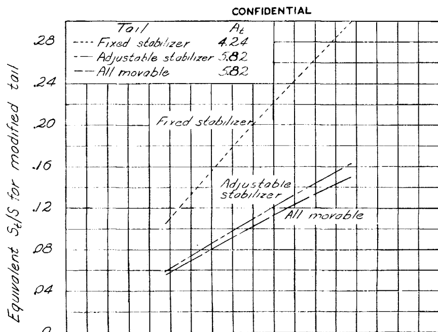
(a) Equivalent tail area for modified tail.
