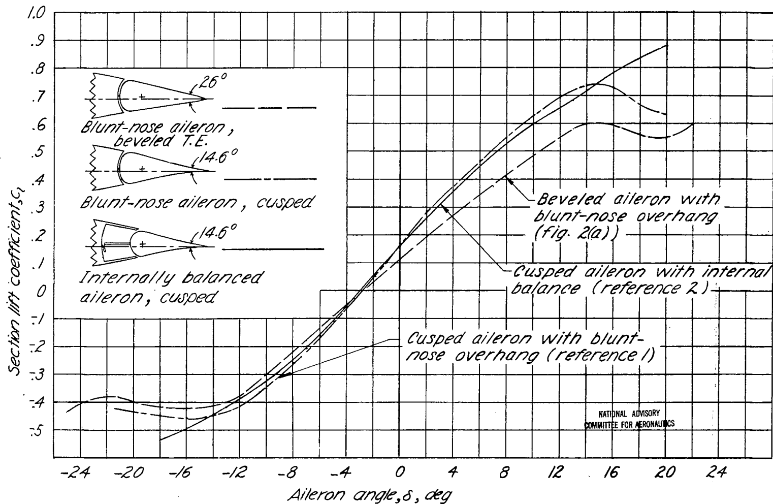
Figure 17. — Variation of section lift coefficient with aileron angle. \alpha_0 = 0^\circ . All ailerons sealed.
