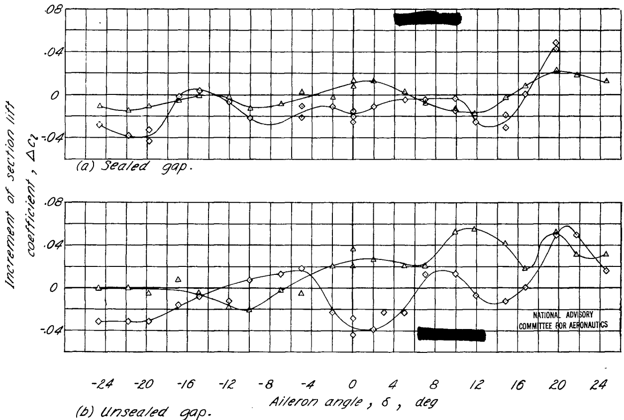
Figure 10. - Effect of rounding airfoil contour adjacent to aileron nose on section lift characteristics of aileron. \alpha_0 = 0^\circ
