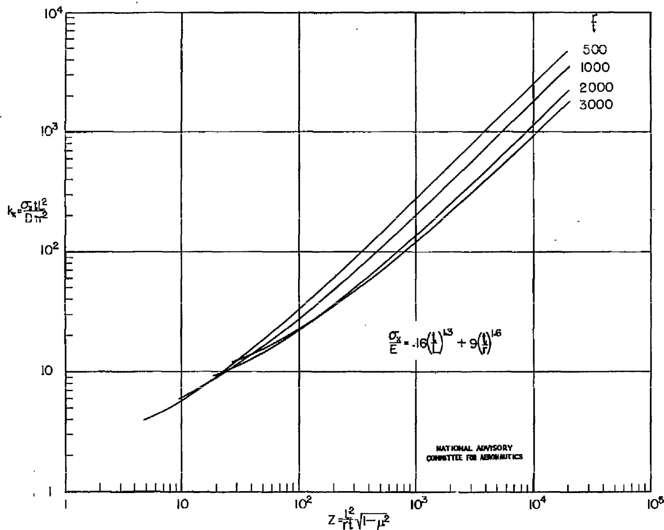
Figure 5.- Critical stress coefficients implied by the formula of Kanemitsu and Nojima (reference 9) for thin-walled cylinders.
