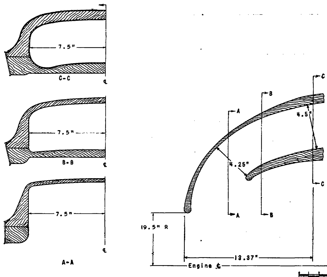
(b) Under-cowling scoop.
