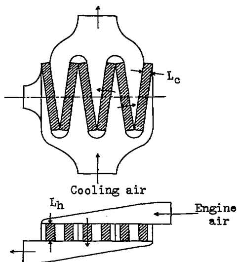
Figure 3.- Suggested type of intercooler.
