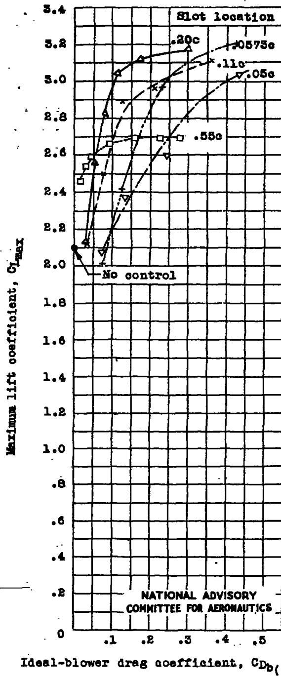
Figure 18.- Variation of maximum lift coefficient with ideal-blower drag coefficient on the NACA 2415 wing with Zap flap deflected 50° to the chord line.
