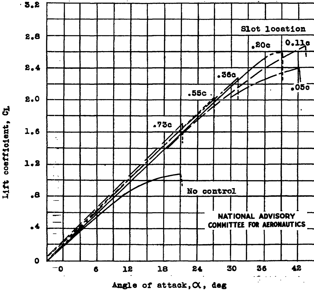
Figure 12,- Lift curves of the NACA 2415 plain wing for six slot locations with constant blower speed.
