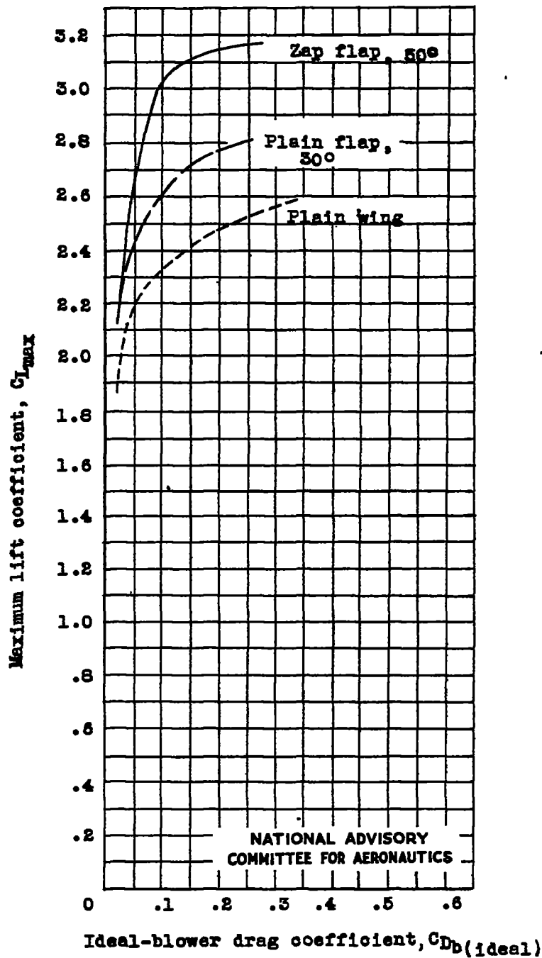
Figure 19.- Comparison of maximum lift coefficient obtained for the NACA 2415 plain wing, for the wing with a plain flap, and for the wing with a Zap flap.
