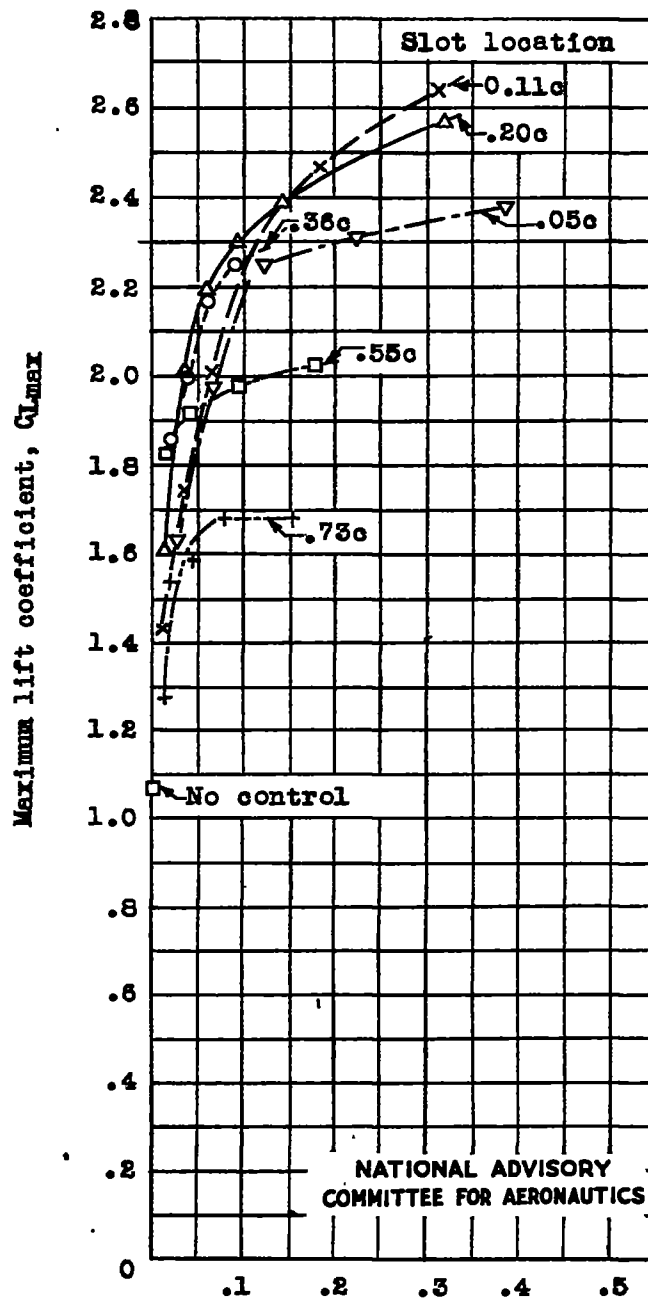
Ideal-blower drag coefficient, CD_b(ideal) Figure 13.- Variation of maximum lift coefficient of the NACA 2415 plain wing with ideal-blower drag coefficient and slot location.
