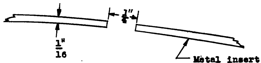
Typical normal-opening suction slot
