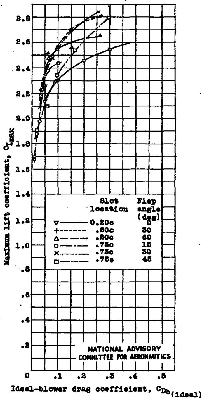
Figure 16.- Variation of maximum lift coefficient with ideal-blower drag coefficient. NACA 2415 wing with plain flap.
