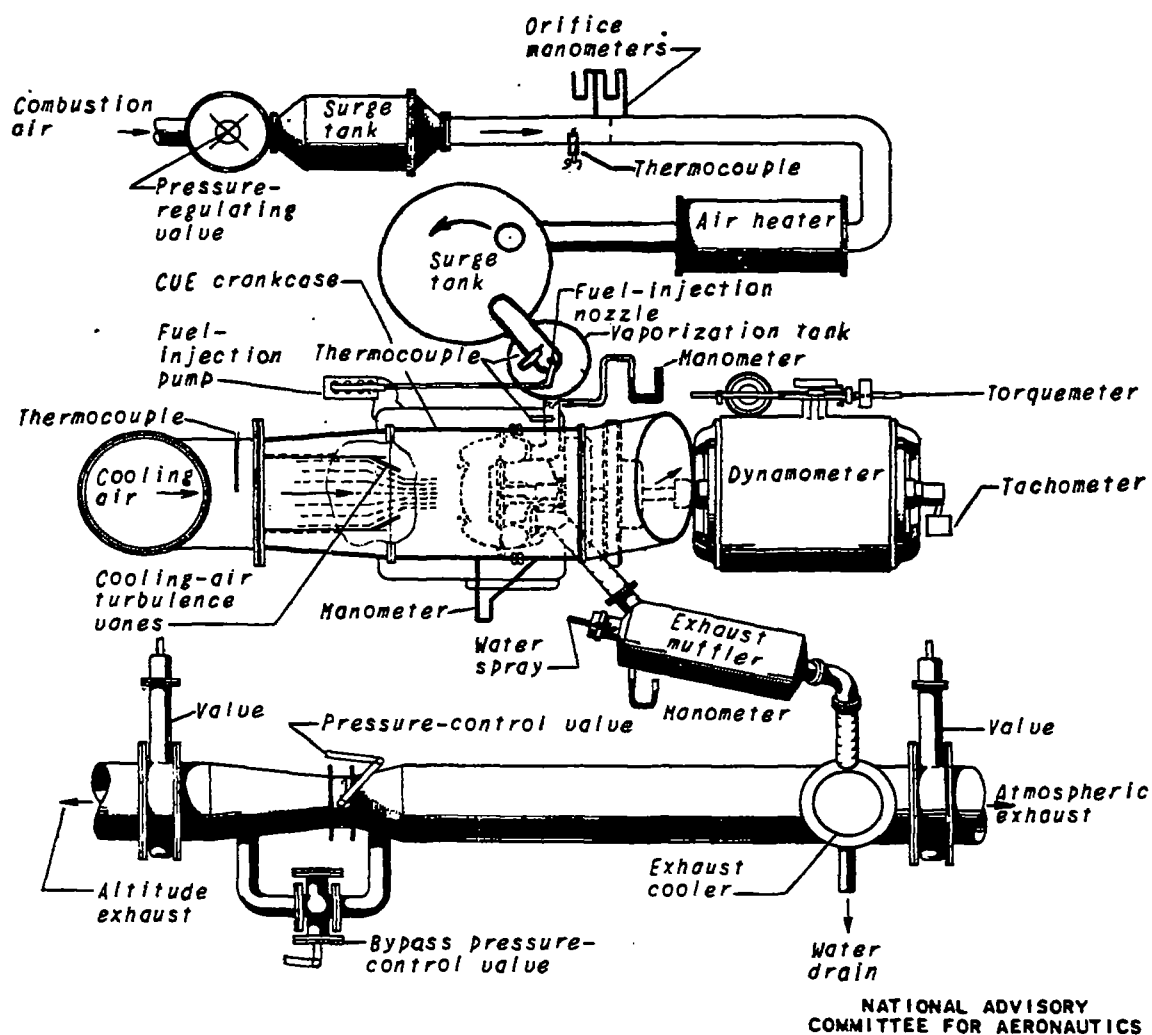
Figure 1. - Arrangement of apparatus for full-scale air-cooled single-cylinder test setup.
