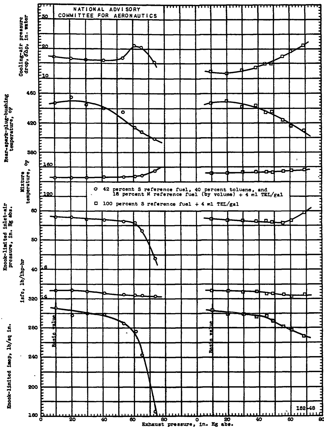
Figure 7. - Effect of exhaust pressure on knock-limited performance of two fuels. Full-scale air-cooled cylinder; engine speed, 2100 rpm; fuel-air ratio, 0.078; compression ratio, 6.9; inlet-air temperature, 200° F; spark advance, both plugs, 20° B.T.C.; cylinder temperature at exhaust end zone, 500° F.
