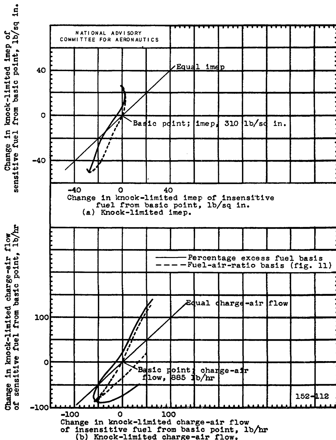
Figure 12. - Effect of comparing fuel-air-ratio knock-test data on percentage excess fuel basis rather than fuel-air-ratio basis.
