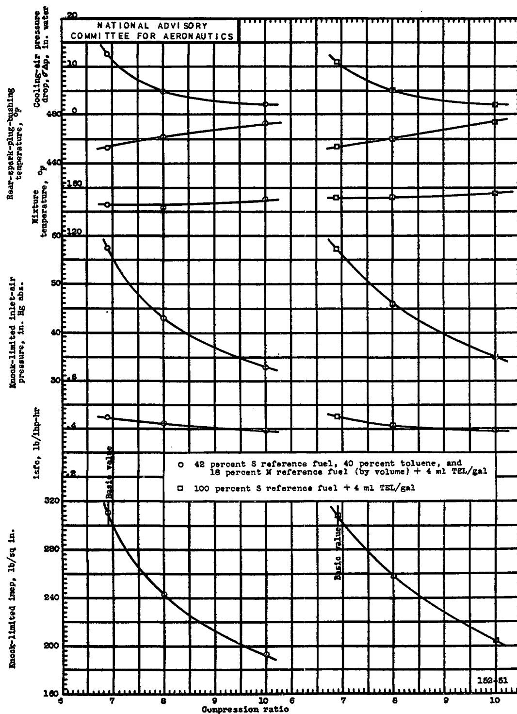
Figure 4. - Effect of compression ratio on knock-limited performance of two fuels. Full-scale air-cooled cylinder; engine speed, 2100 rpm; fuel-air ratio, 0.078; inlet-air temperature, 200^{\circ}\text{F} ; spark advance, both plugs, 20^{\circ} B.T.C.; exhaust pressure, 10 inches mercury absolute; cylinder temperature at exhaust end zone, 500^{\circ}\text{F} .
