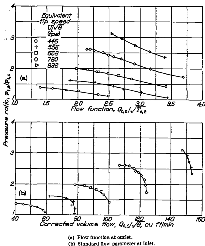
FIGURE 4.—Performance curves of typical axial-flow compressor.
