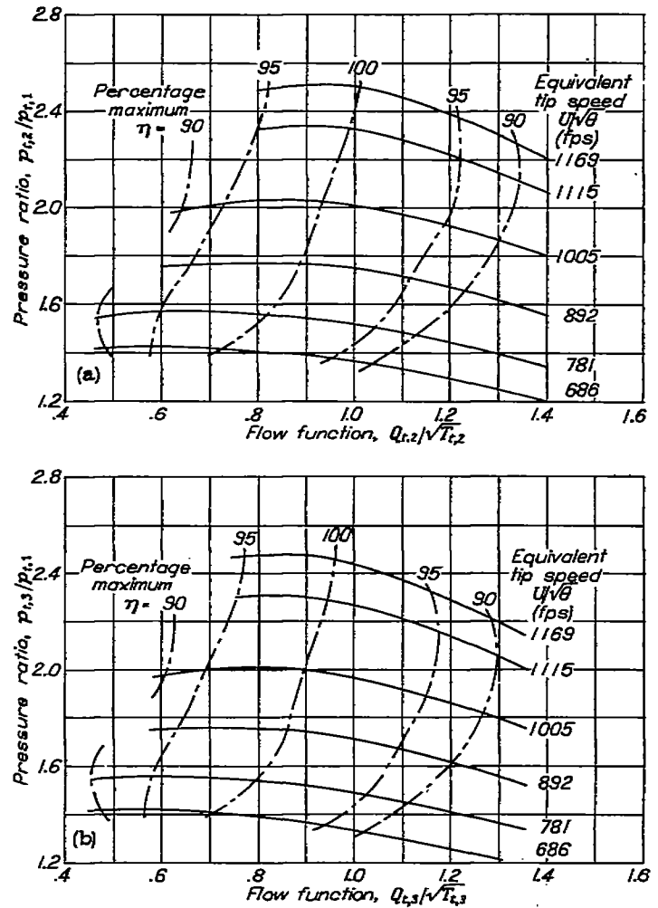
(a) Experimental performance. (b) Performance corrected for pressure and temperature changes through aftercooler; k_2 , 0.015; \eta_c , 0.45.
