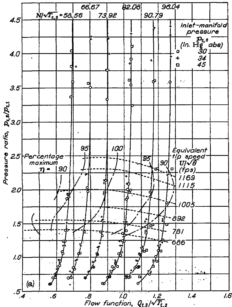
(a) Compressor performance for constant values of U/\sqrt{\theta} .
