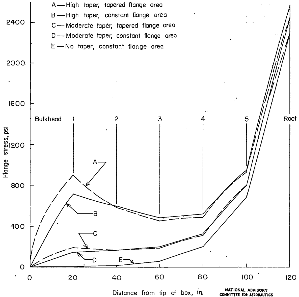
(a) Flange stresses.
