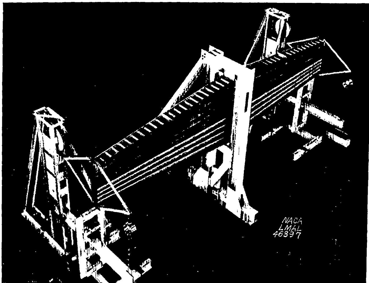
Figure 6.- Setup for torsion tests of tapered box beam.
