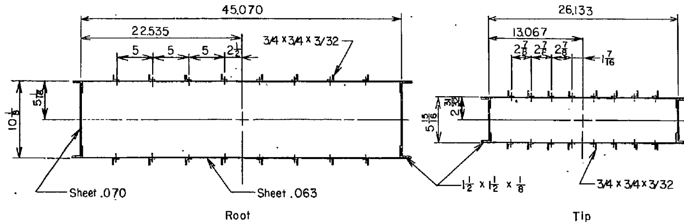
(a) Actual root and tip cross sections.
