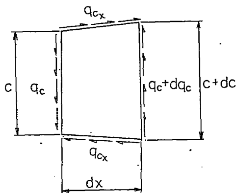
(b) Infinitesimal section of spar web.
