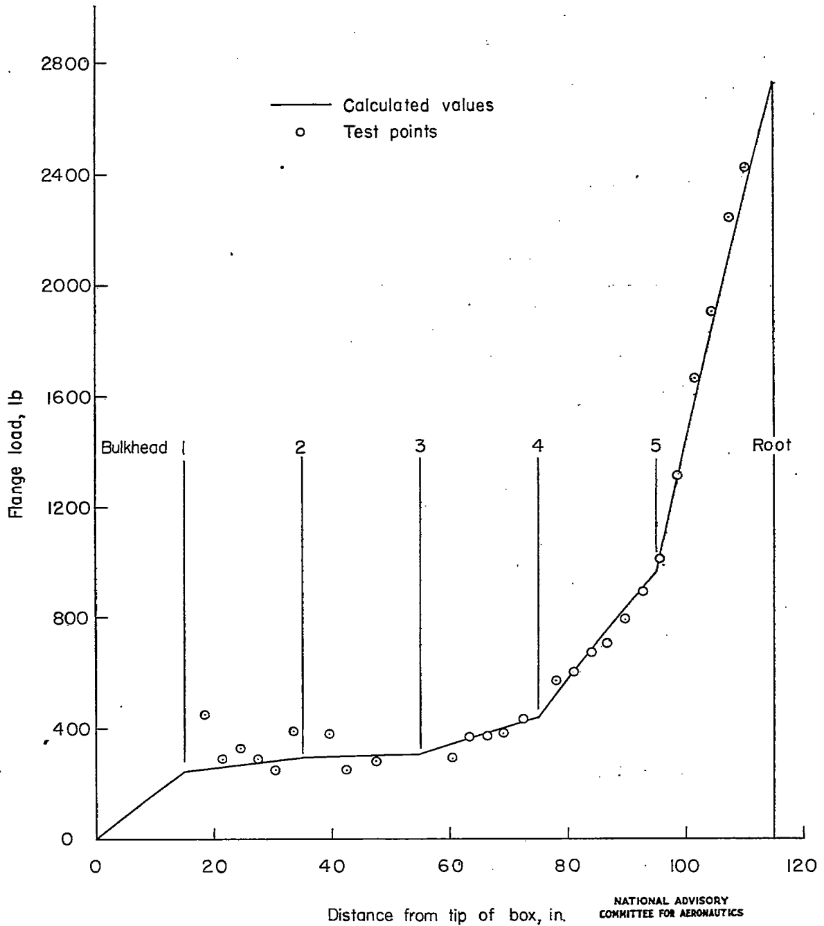
Figure 13.— Comparison of experimental and calculated flange loads for tip loading condition.
