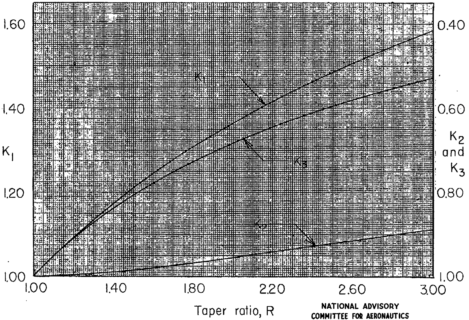
Figure 4.—Variation of taper constants with taper ratio.
