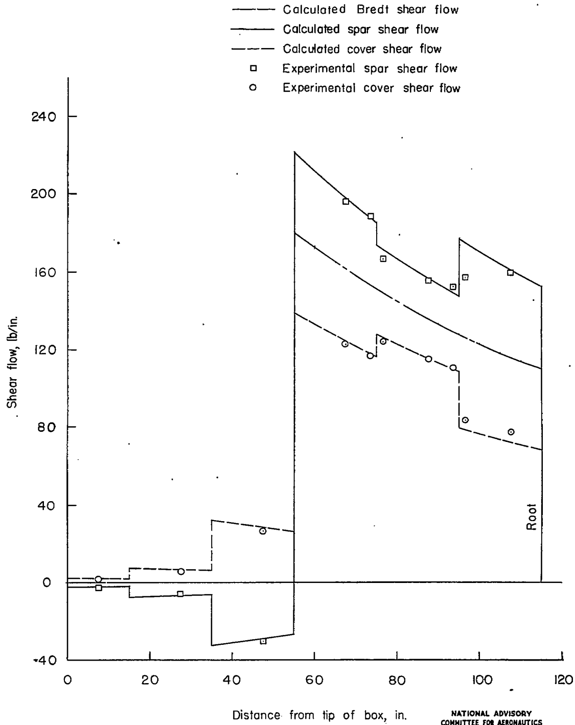
Figure 12.— Comparison of experimental and calculated shear flows for quarter-point loading condition. T=100,000 inch-pounds.
