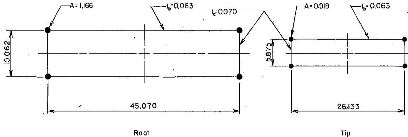
(b) Equivalent root and tip cross sections.
