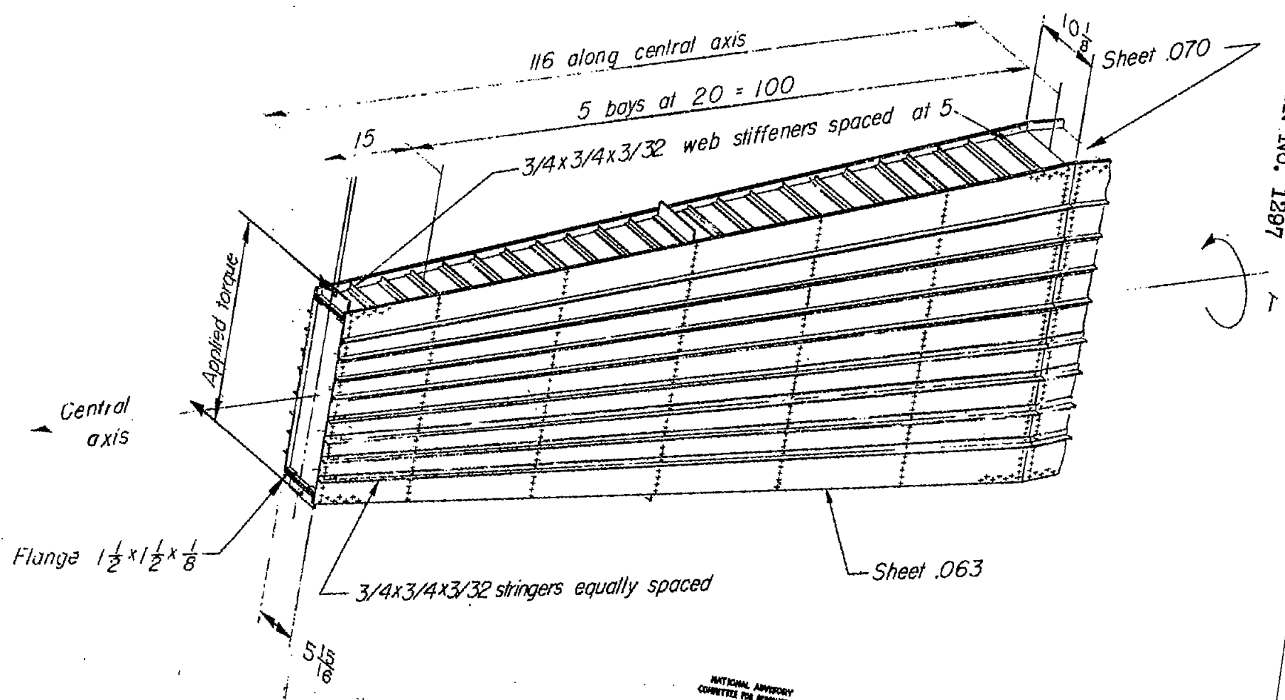
Figure 7.—Tapered box beam.
