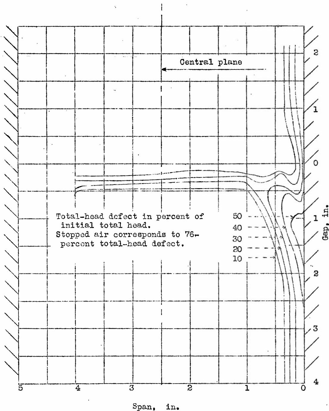
Figure 12.- Contours of constant total-head defect downstream of cascade. Cascade of NACA 65,2-810 sections; Stagger: 45^\circ ; \alpha_1 : 12^\circ ; Solidity: 1.
