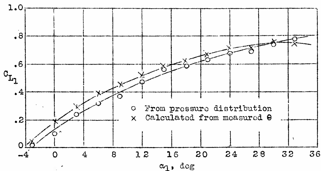
Figure 7.- Lift coefficients based on initial air conditions. Cascade of NACA 65,2-810 sections; Stagger: 45^\circ ; Solidity: 1.
