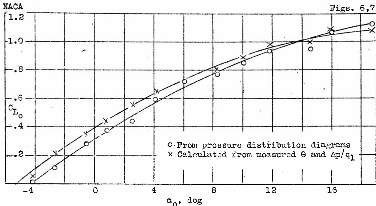
Figure 6.- Lift coefficients based on mean air conditions. Cascade of NACA 65,2-810 sections; Stagger: 45^\circ ; Solidity: 1.
