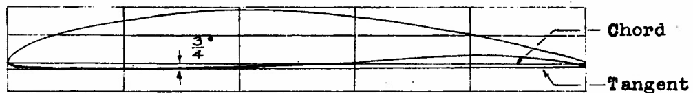
Blower-blade section NACA 65,2-810
