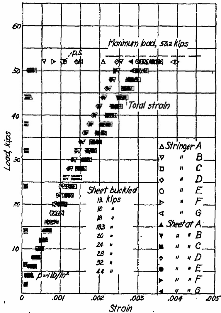
Figure 38.- Test of panel 27. Vacuum on sheet side, 1 psi; length, 19 inches; sheet thickness, 0.0282 in.
