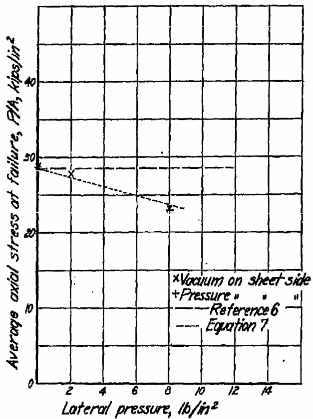
Figure 52.- Effect of lateral pressure on average axial stress at failure for panels 23 to 25 with 19 in. length and 0.051 in. sheet.
