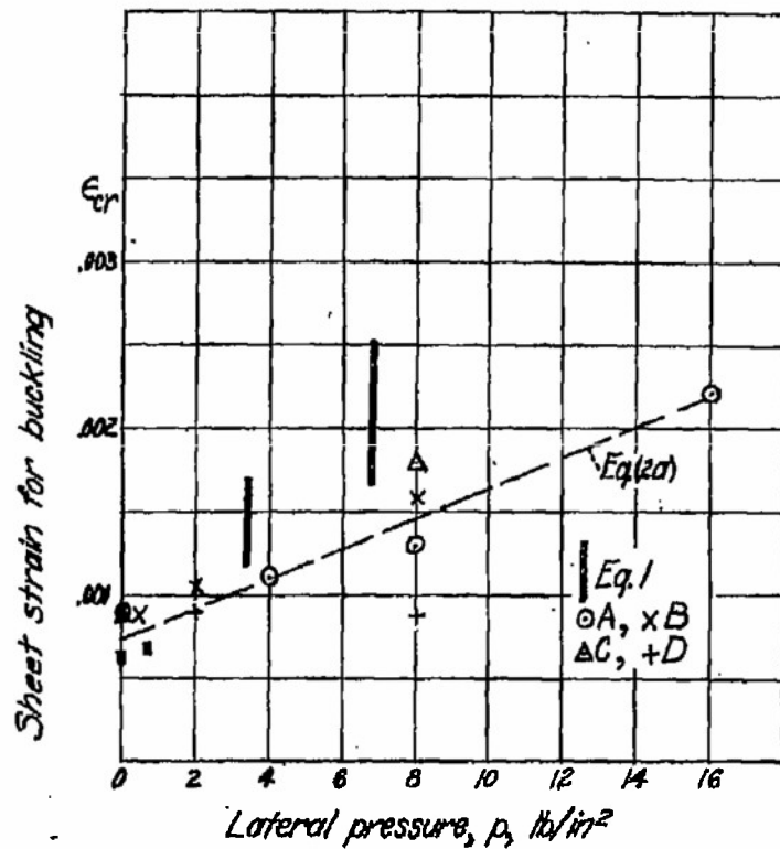
Figure 41.- Effect of lateral pressure on sheet strain at stringer edge for buckling of 0.051 inch panels. A and B, panels with pressure and vacuum on sheet side respectively for l = 12 in., w = 18-3/4 in.; C and D the same for l = 19 in., w = 18-3/4 in.
