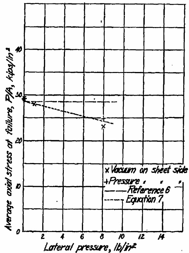
Figure 53.- Effect of lateral pressure on average axial stress at failure for panels 26 to 29 with 19 in. length; six sheet bays; 0.025 in. sheet.
