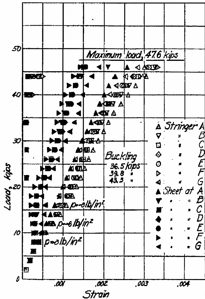
Figure 35.- Test of panel 26. Vacuum on sheet side, 8 psi; length, 19 inches; sheet thickness, 0.0259 in.
