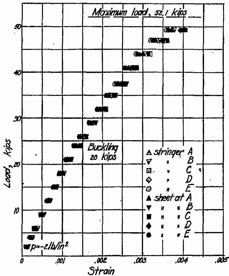
Figure 31.- Test of panel 13. Vacuum on sheet side, 2 psi; length, 12 inches; sheet thickness, 0.0515 in.
