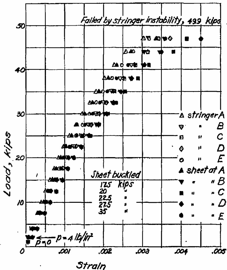
Figure 24.- Test of panel 15. Pressure on sheet side, 4 psi; length, 12 inches; sheet thickness, 0.0515 in.
