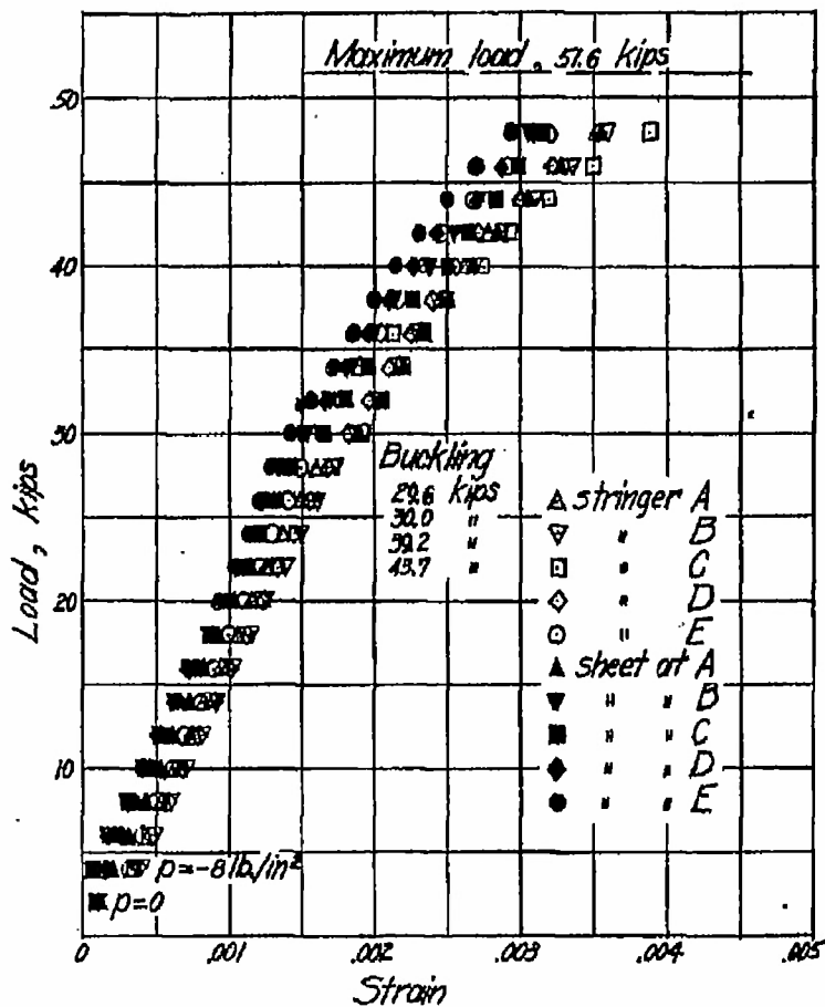
Figure 30.- Test of panel 11. Vacuum on sheet side, 8 psi; length, 12 inches; sheet thickness, 0.0513 in.
