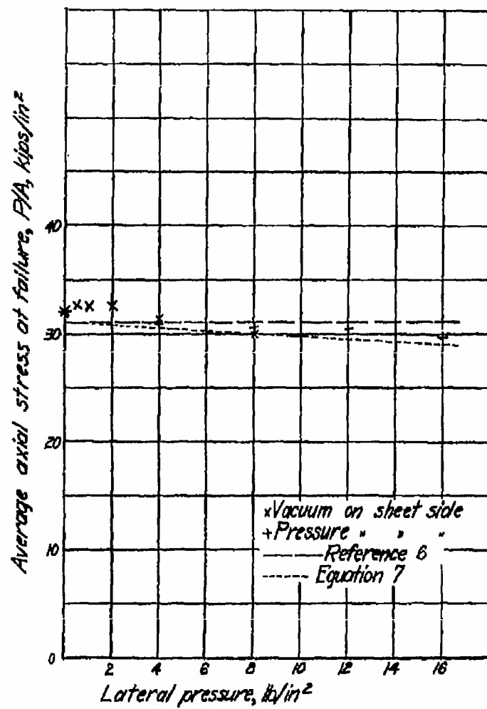
Figure 49.- Effect of lateral pressure on average axial stress at failure for panels 1 to 10 with 12 in. length and 0.025 in. sheet.
