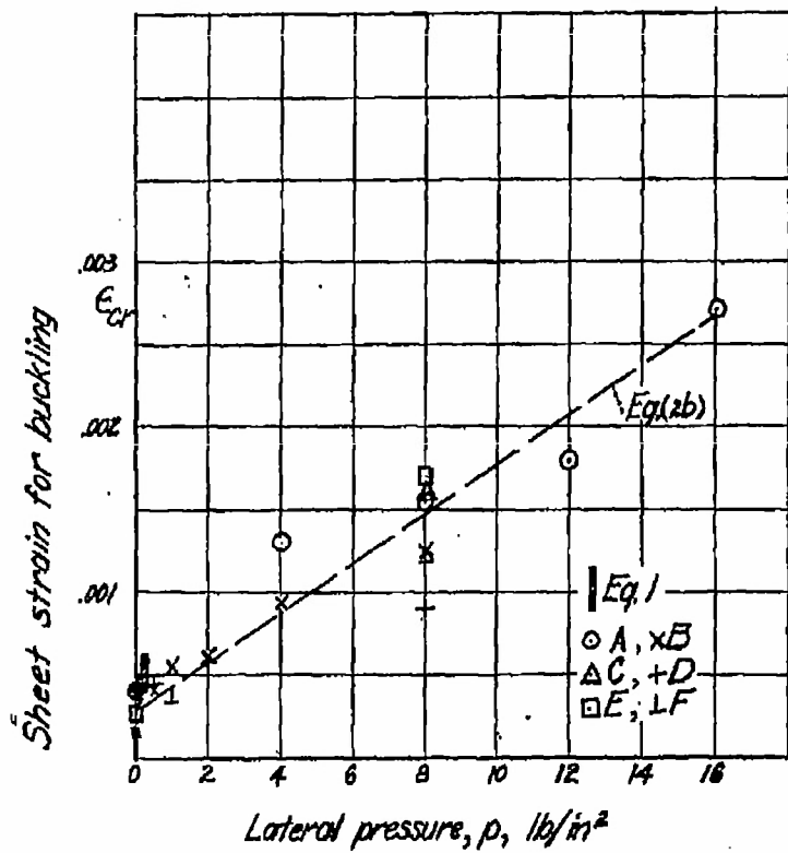
Figure 40.- Effect of lateral pressure on sheet strain at stringer edge for buckling of 0.035 inch panels. A and B, panels with pressure and vacuum on sheet side respectively for l = 18 in., w = 18-3/4 in.; C and D the same for l = 19 in., w = 18-3/4 in.; E and F the same for l = 19 in., w = 24-3/4 in.
