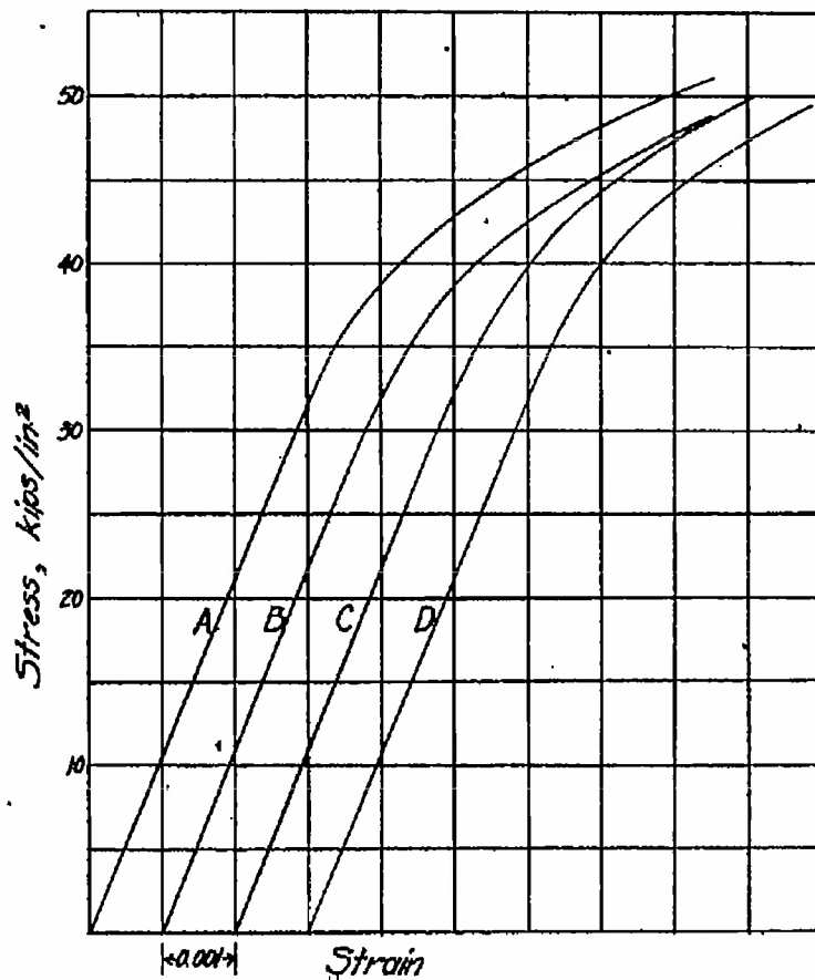
Figure 2.- Compressive stress-strain curves of sheet material: A, panels 1,3,4,7,8,18,19,20,21,27; B, panels 2,5,6,9,10,28,29,29; C, panels 11,12,14,15,16,17; D, panels 13,22,23,24,25.
