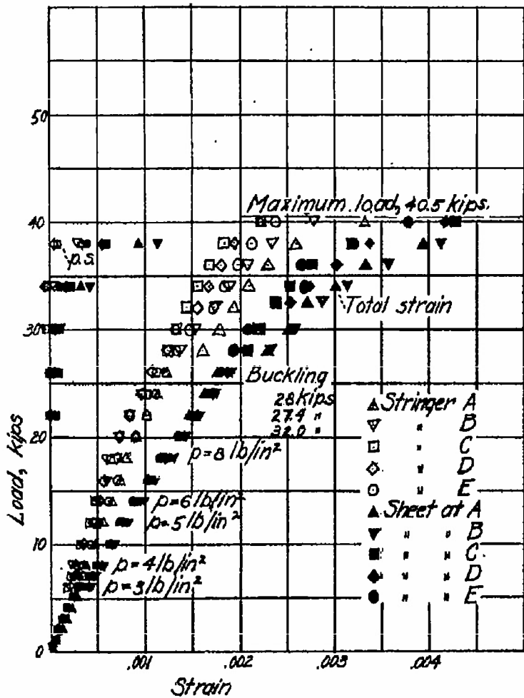
Figure 34.- Test of panel 25. Pressure on sheet side, 8 psi; length, 19 inches; sheet thickness, 0.0521 in.
