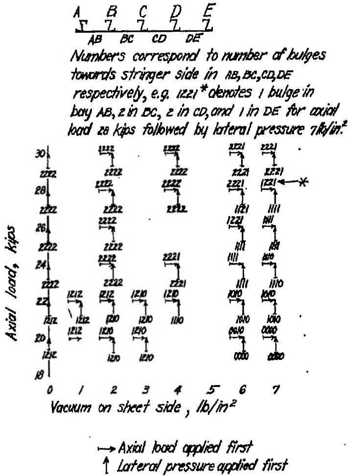
Figure 8.- Buckles pattern for panel 13 in the elastic range with vacuum on the sheet side from zero to 7 psi and axial load from 20 to 30 kips.
