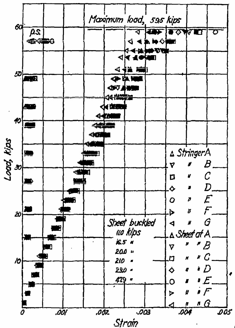
Figure 37.- Test of panel 28. No lateral pressure; length, 19 inches; sheet thickness, 0.0280 in.
