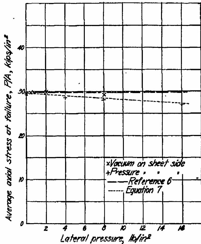
Figure 50.- Effect of lateral pressure on Average axial stress at failure for panels 11 to 17 with 12 in. length and 0.051 in. sheet.
