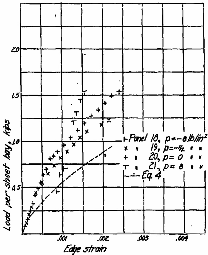
Figure 46.- Sheet load against edge strain, vacuum on sheet side, length, 19 in., sheet thickness, 0.035 in.
