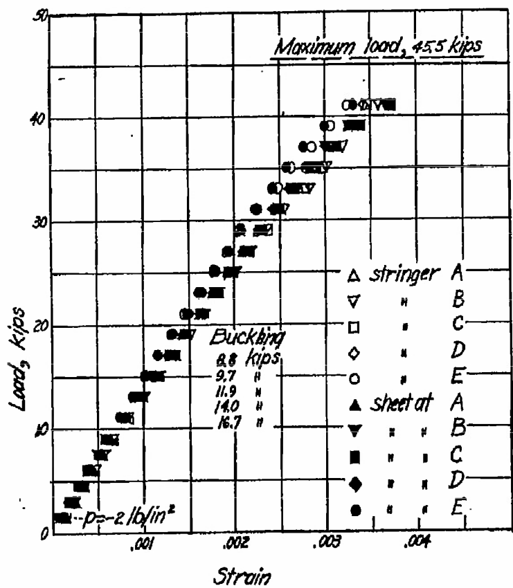
Figure 12.- Test of panel 3. Vacuum on sheet side, 2 psi; length, 12 inches; sheet thickness, 0.0261 in.
