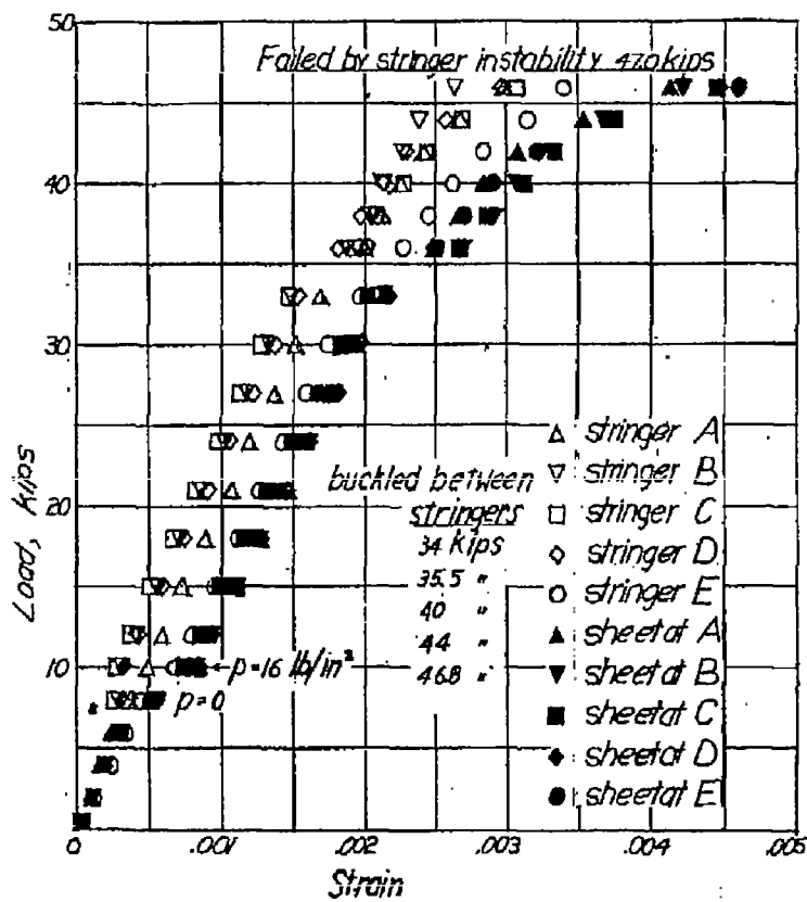
Figure 26.- Test of panel 17. Pressure on sheet side, 16 psi; length, 12 inches; sheet thickness, 0.0520 in.
