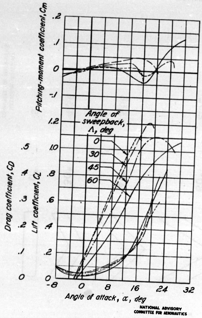
Figure 4.- Representative data from reference 2 showing the effect of sweepback on lift, drag, and pitching-moment coefficients.
