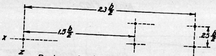
Positions of tail relative to wing M.A.C.
