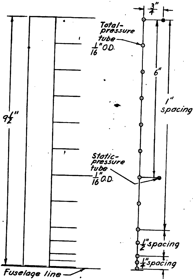
Figure 4.- Rakes used to determine boundary-layer profile.
