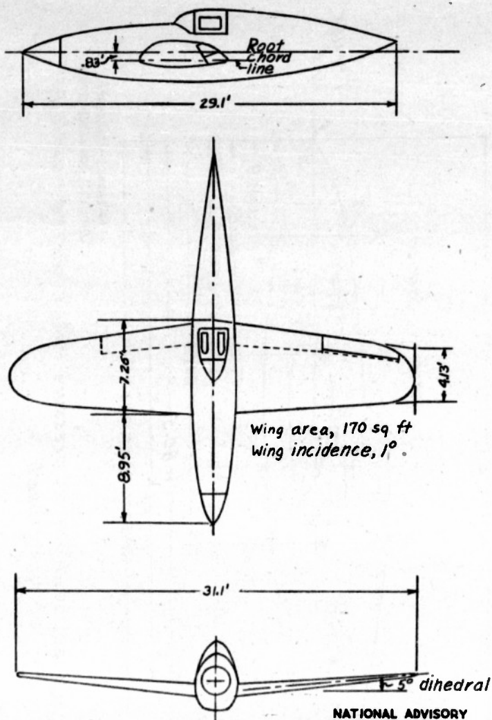
Figure 2.-General arrangement of model.
