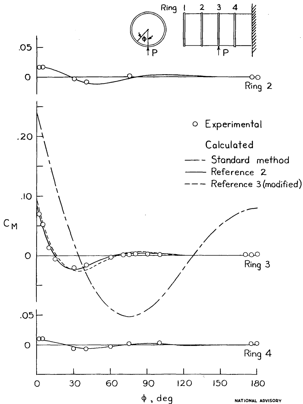
Figure 5. - Ring bending-moment coefficients in cylinder I for radial load at ring 3.
