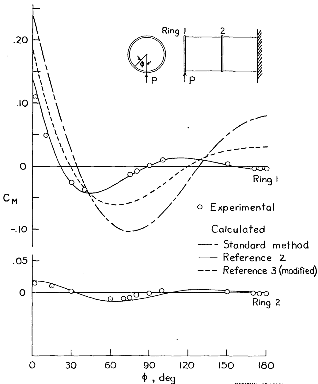
Figure 7.— Ring bending-moment coefficients in cylinder 1a for radial load at ring 1.
