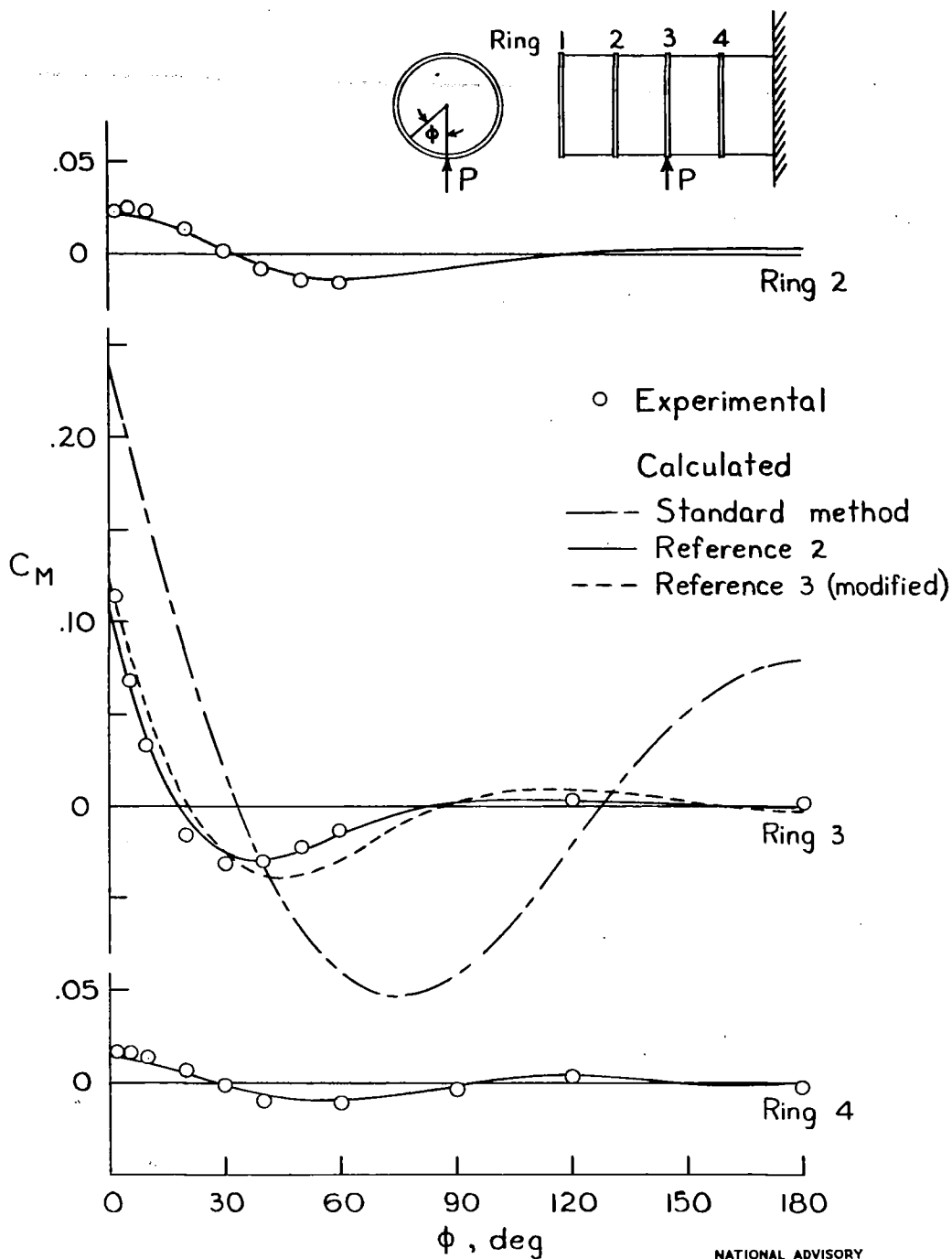
Figure 20. - Ring bending-moment coefficients in cylinder 4 for radial load at ring 3.
