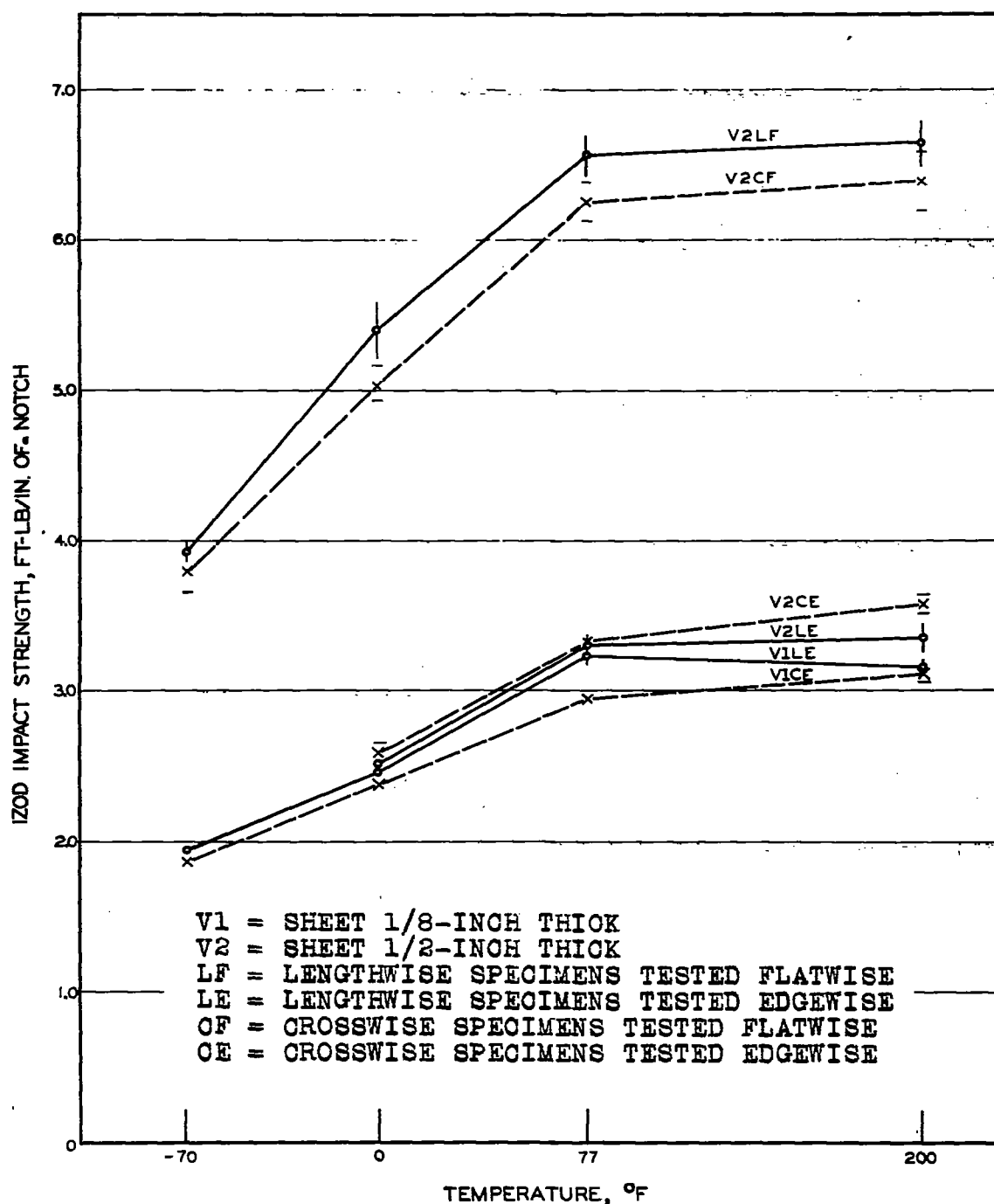
Figure 6.- Variation of IZOD impact strength with temperature for low-pressure grade C cotton-fabric phenolic laminate. Mean value \pm standard error is indicated by \circ or \bar{x} .
