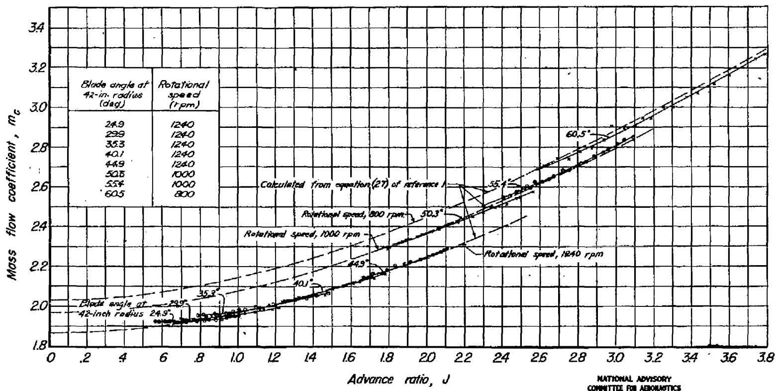
Figure 27.—Variation of the coefficient of mass flow of de-icing air with advance ratio.
