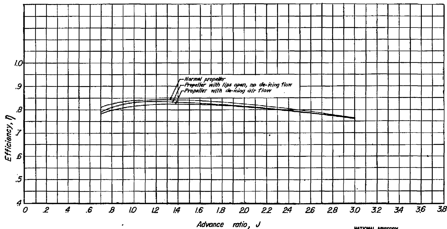
Figure 32.—A comparison of the envelope curves of propeller efficiency.
