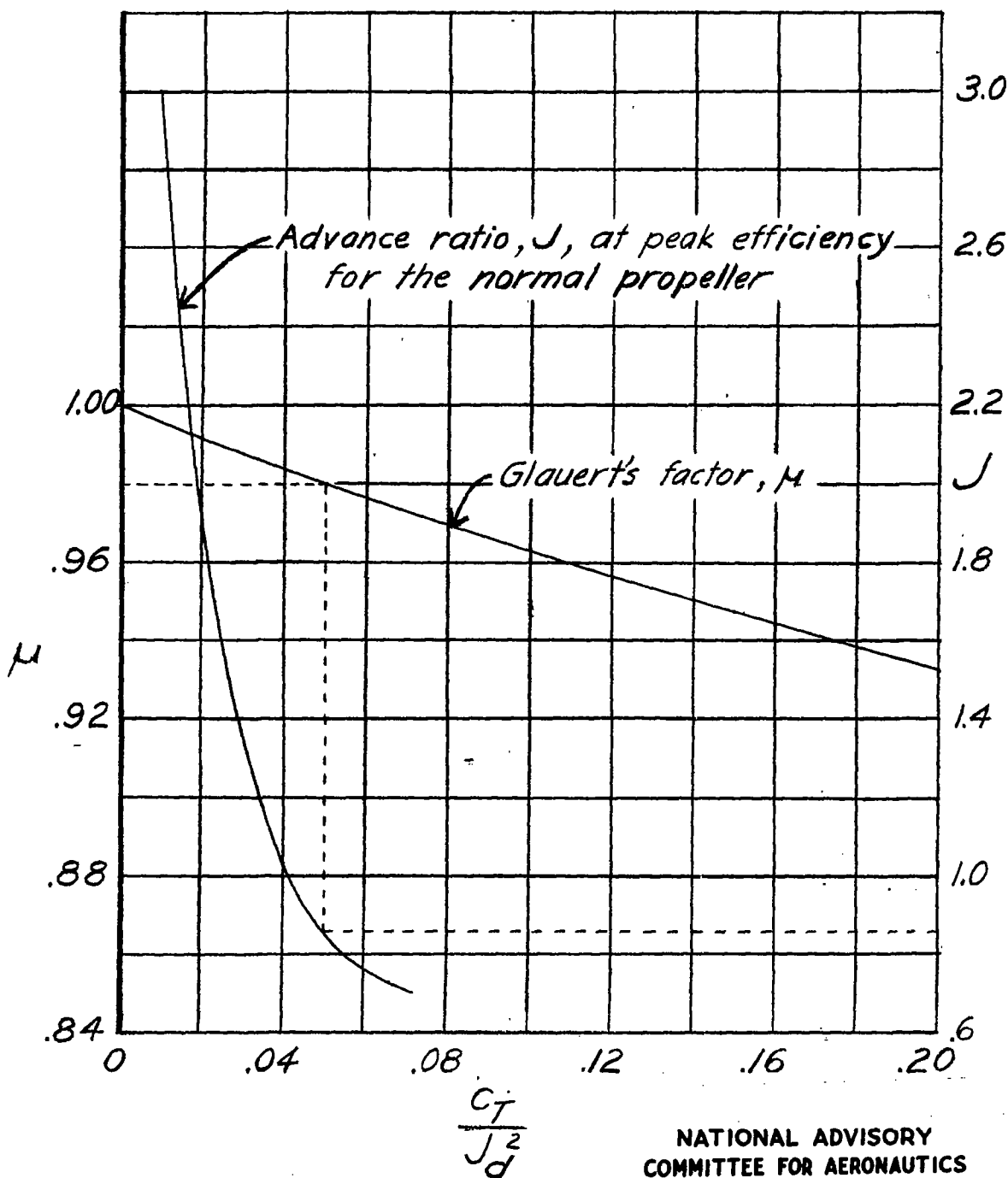
Figure 11.— Glauert's factor for correcting wind tunnel datum velocity to equivalent free airspeed for a 12.208-foot-diameter propeller in a closed 16-foot circular test jet.
