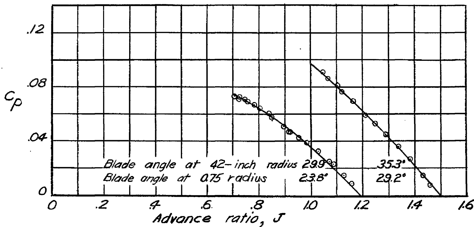
Figure 19.—Variation of power coefficient with advance ratio. Tips open; no de-icing flow; rotational speed, 1450 rpm.
