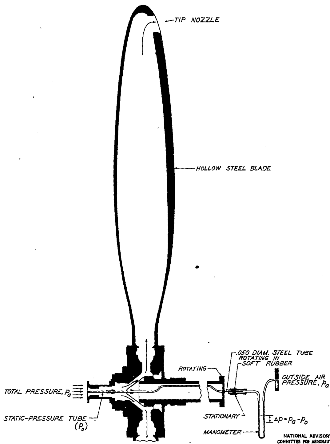
FIGURE 10.—PATH OF INTERNAL FLOW THROUGH THE PROPELLER AND THE INTERNAL-MASS-FLOW METER.
