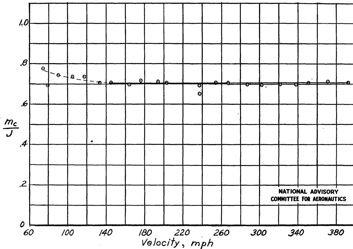
Figure 30.- Coefficient of mass flow of de-icing air for infinite advance ratio (rotational speed very low).
