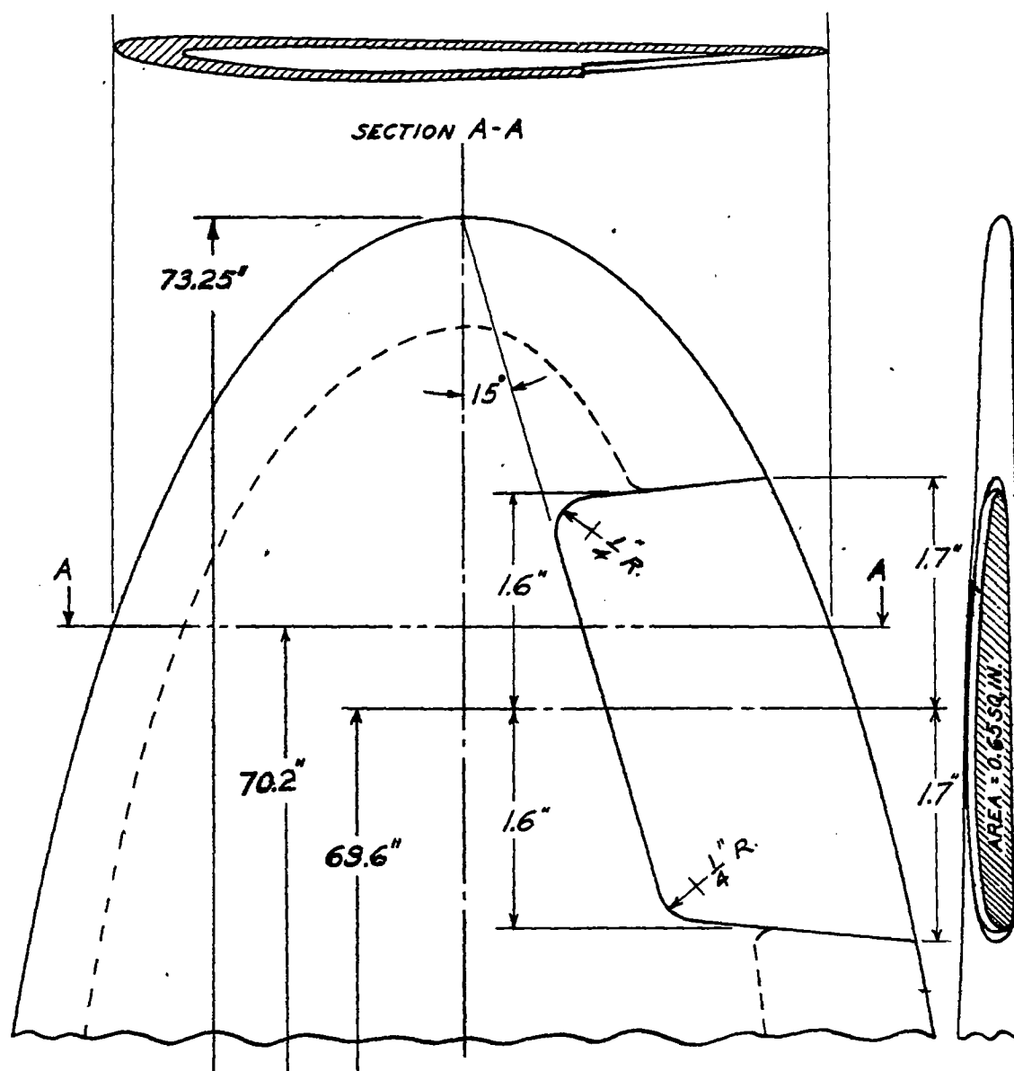
FIGURE 8.- APPROXIMATE DIMENSIONS OF THE TIP OPENING IN THE CURTISS 714-1C2-12 PROPELLER.
