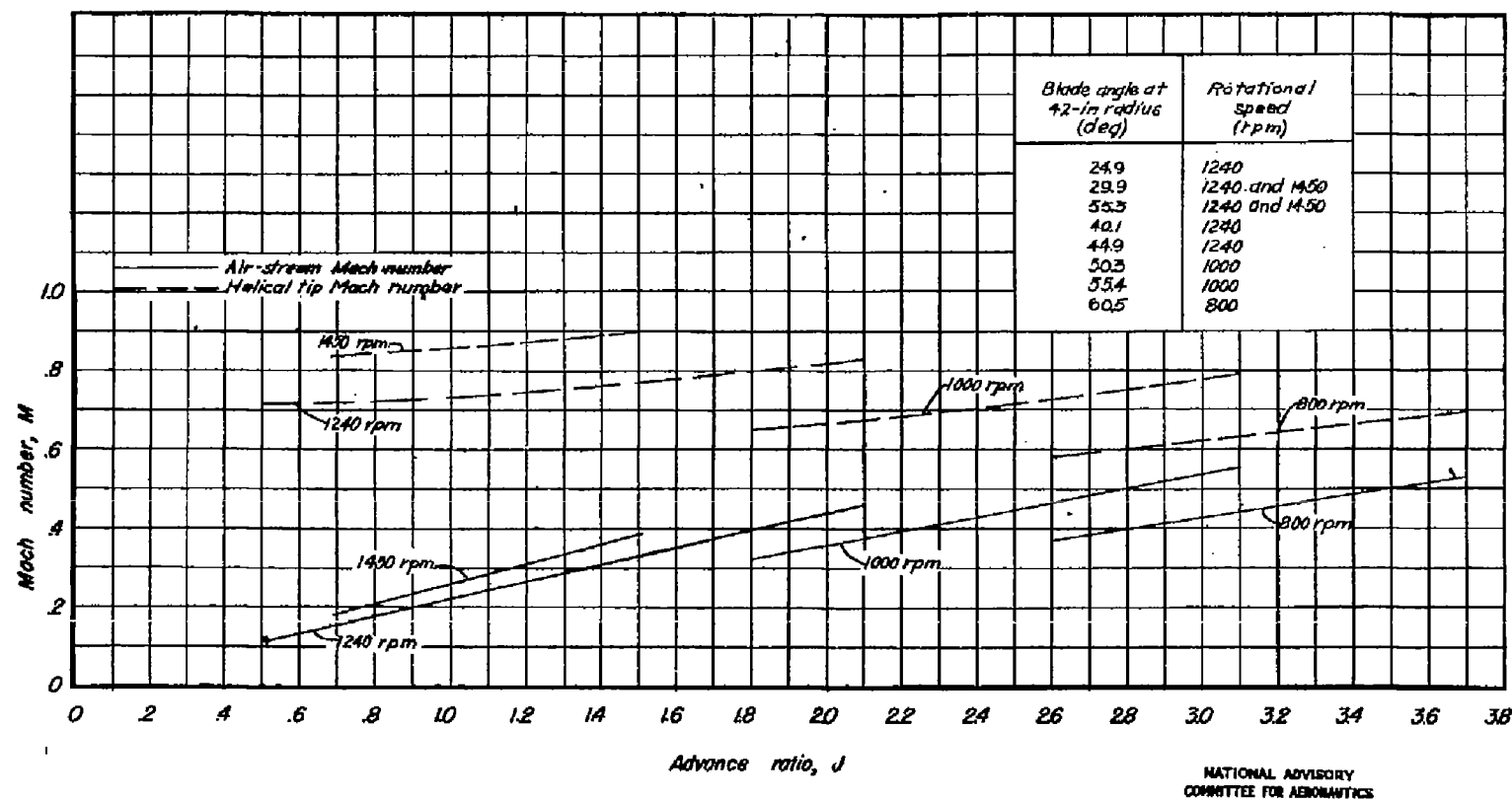
Figure 31.—Variation of air-stream Mach number and helical tip Mach number with advance ratio.
