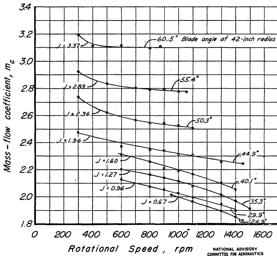
Figure 29.—Variation of the coefficient of mass flow of de-icing air with rotational speed.
