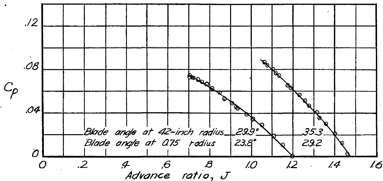
Figure 25.—Variation of the power coefficient with advance ratio. Propeller with de-icing air flow; rotational speed, 1450 rpm.
