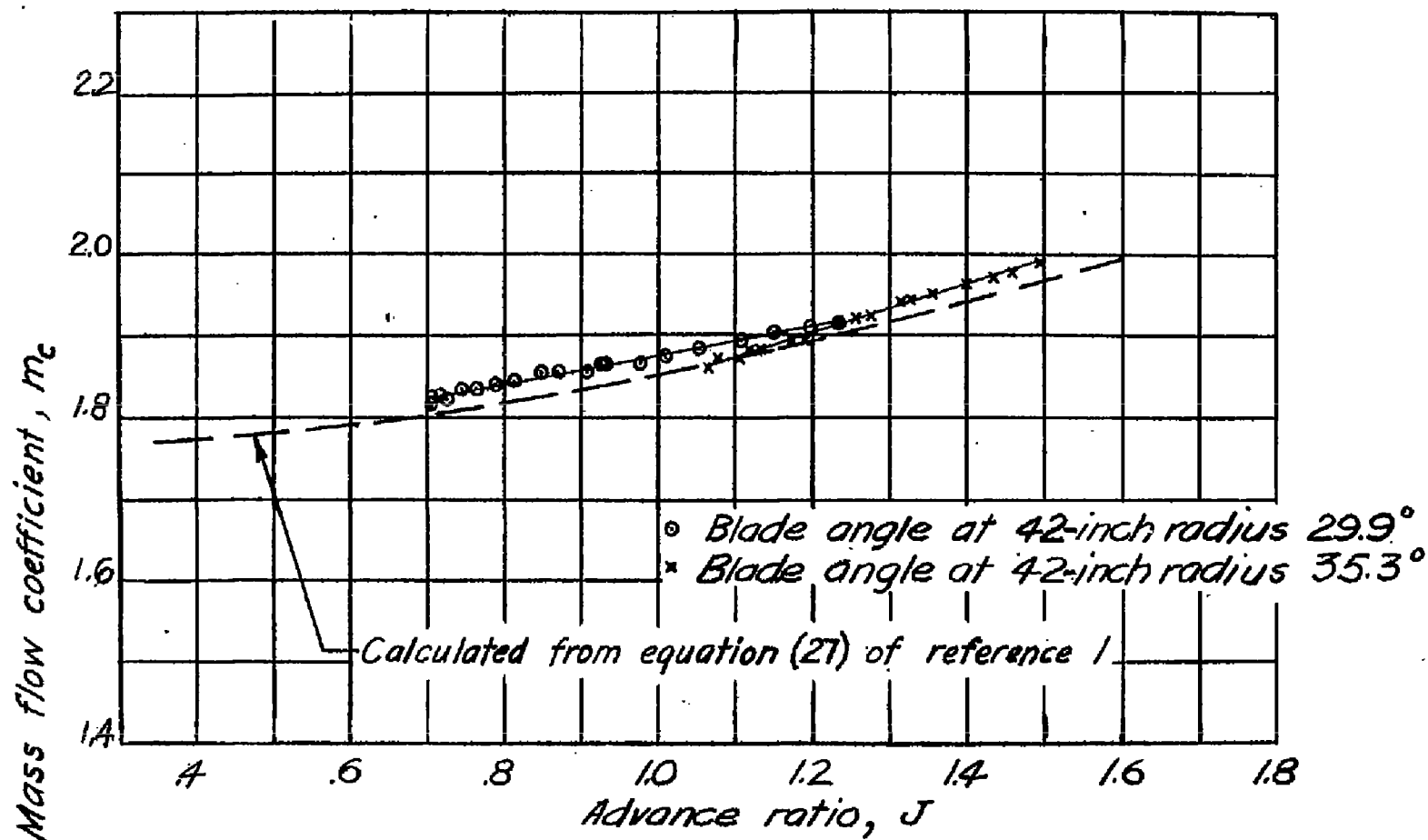
Figure 28.— Variation of the coefficient of mass flow of de-icing air with advance ratio. Rotational speed, 1450 rpm.
