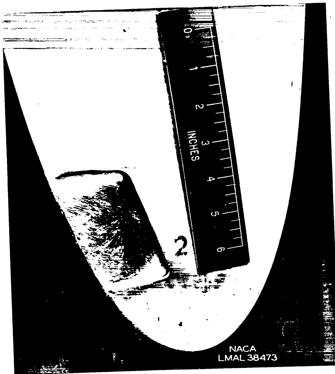
Figure 6.- Tip opening in blade 2.
