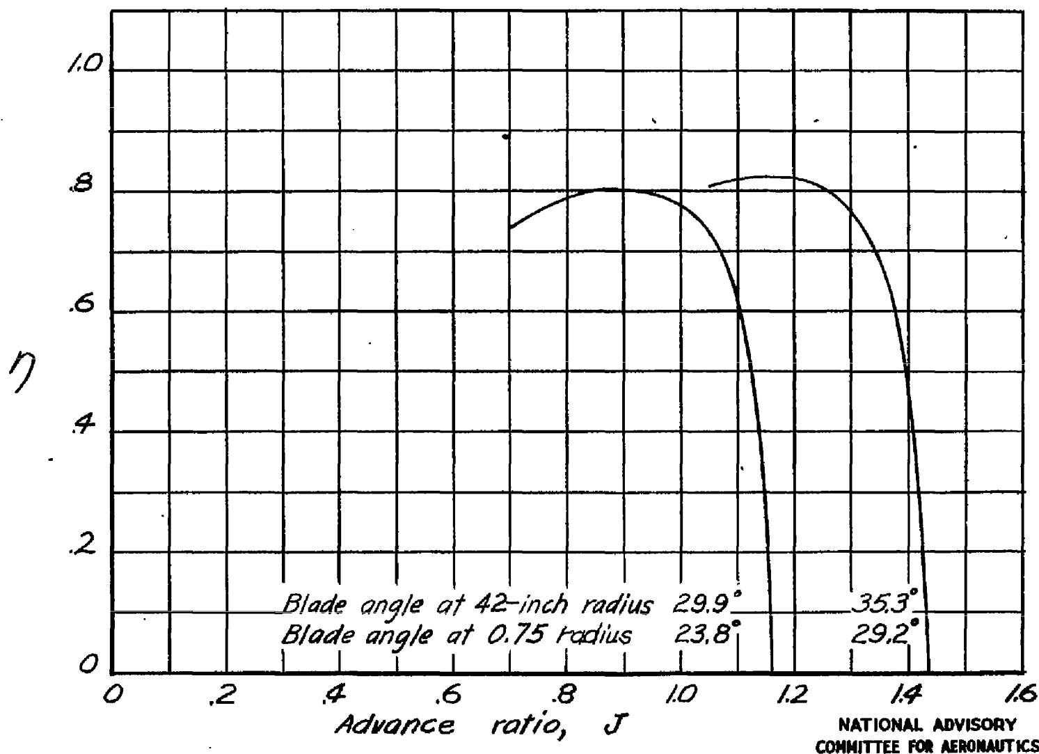
Figure 26.-Variation of propeller efficiency with advance ratio. Propeller with de-icing air flow; rotational speed, 1450 rpm.
