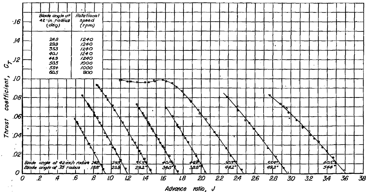
Figure 12.—Variation of thrust coefficient with advance ratio. Normal propeller.
