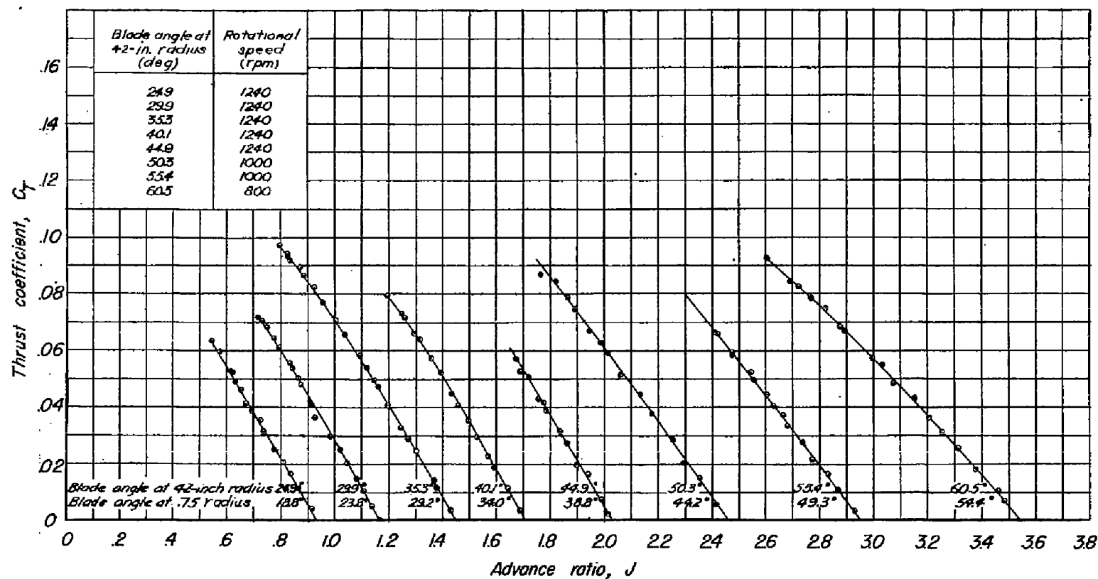
Figure 15.—Variation of thrust coefficient with advance ratio. Tips open, no de-icing flow.
