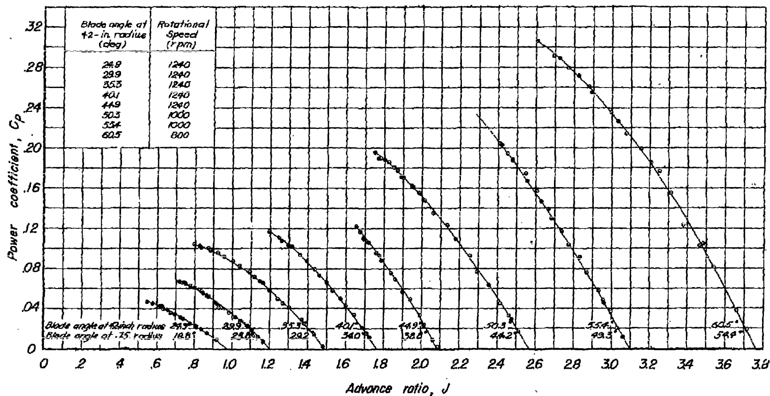
Figure 16.—Variation of power coefficient with advance ratio. Tips open, no de-icing flow.
