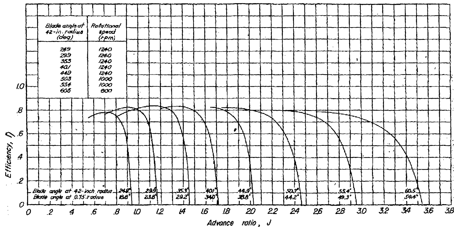
Figure 17.—Variation of propeller efficiency with advance ratio, Tips open; no de-icing flow.
