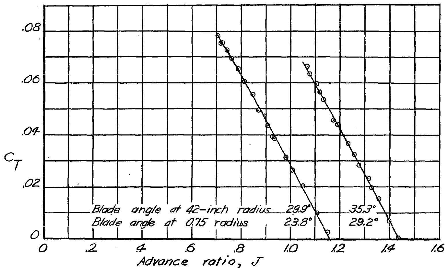
Figure 24.—Variation of thrust coefficient with advance ratio. Propeller with de-icing air flow; rotational speed, 1450 rpm.
