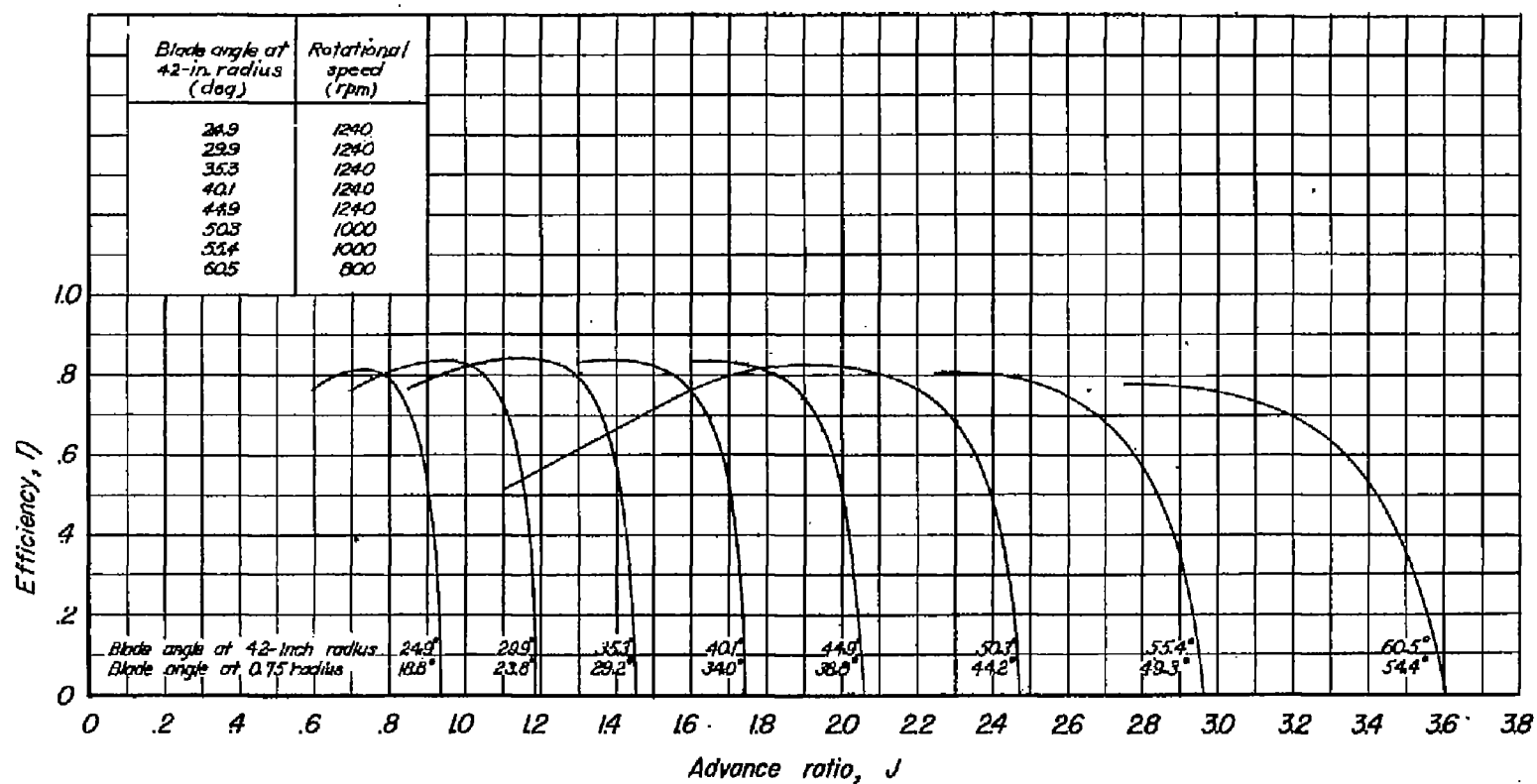
Figure 14.—Variation of propeller efficiency with advance ratio. Normal propeller.
