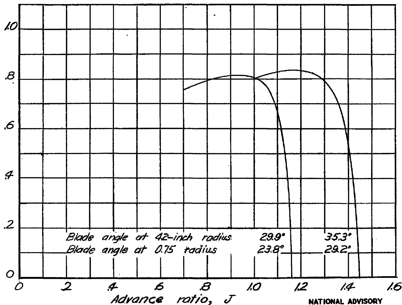
Figure 20.- Variation of propeller efficiency with advance ratio, Tips open; no de-icing flow; rotational speed, 1450 rpm.
