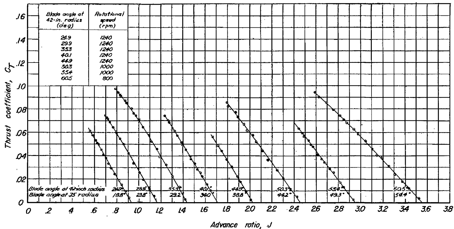
Figure 21.—Variation of thrust coefficient with advance ratio. Propeller with de-icing air flow
