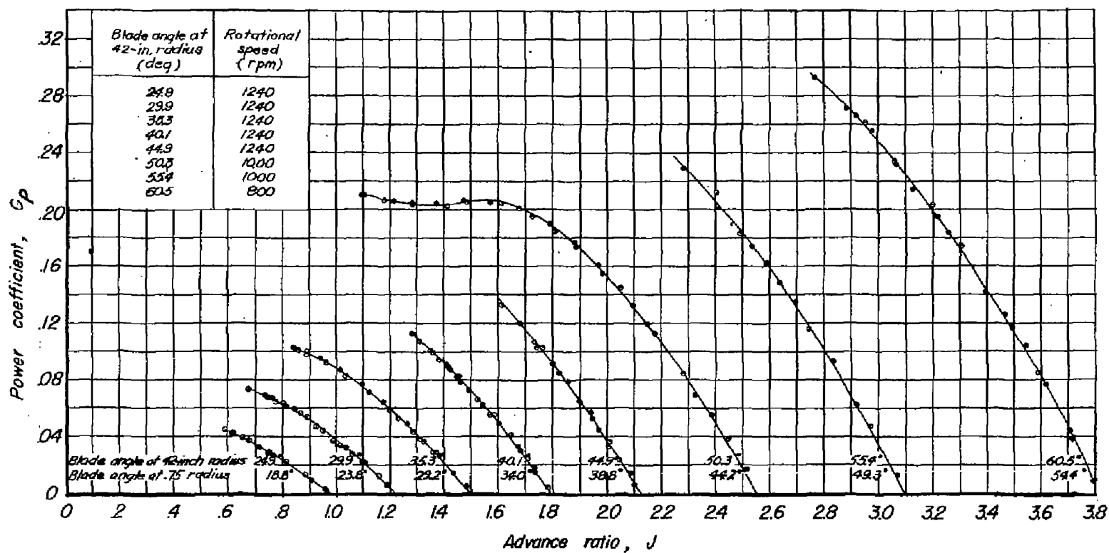
Figure 13.—Variation of power coefficient with advance ratio, Normal propeller.
