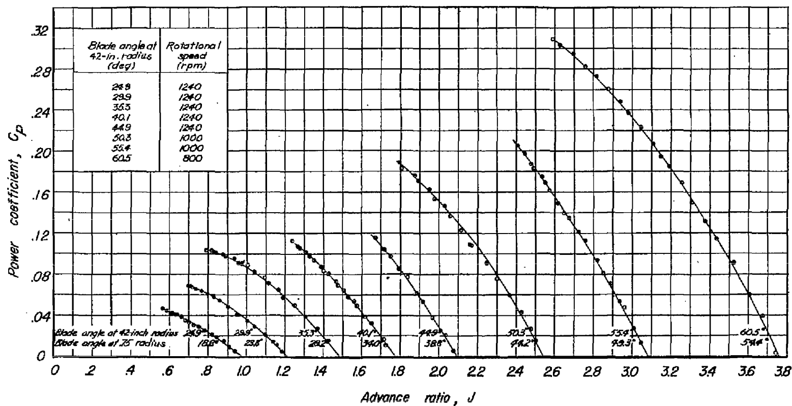
Figure 22.—Variation of power coefficient with advance ratio. Propeller with de-icing air flow.
