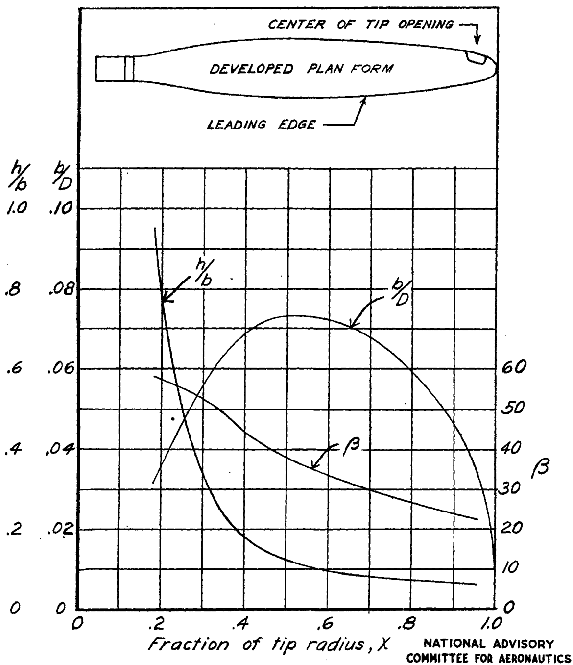
Figure 4.- Blade form curves for Curtiss 714-1C2-12 propeller.
