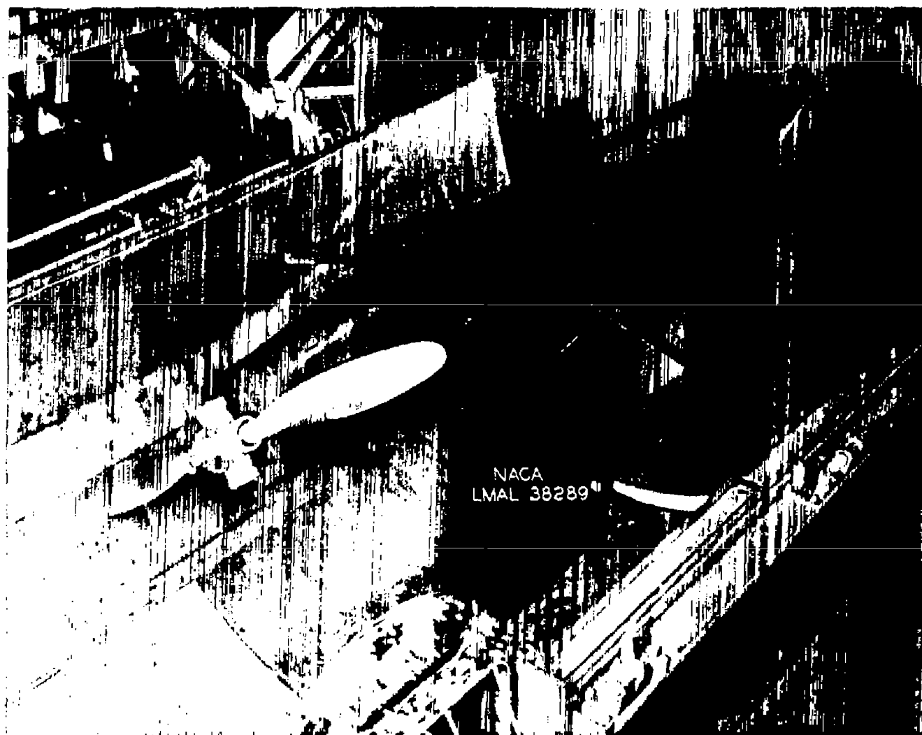
Figure 2.- Propeller dynamometer mounted in test section. Normal propeller, tunnel open.
