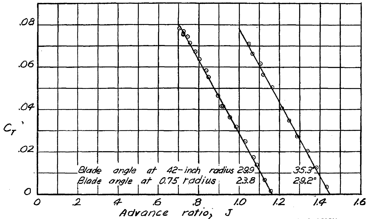
Figure 18.—Variation of thrust coefficient with advance ratio. Tips open; no de-icing flow; rotational speed, 1450 rpm.
