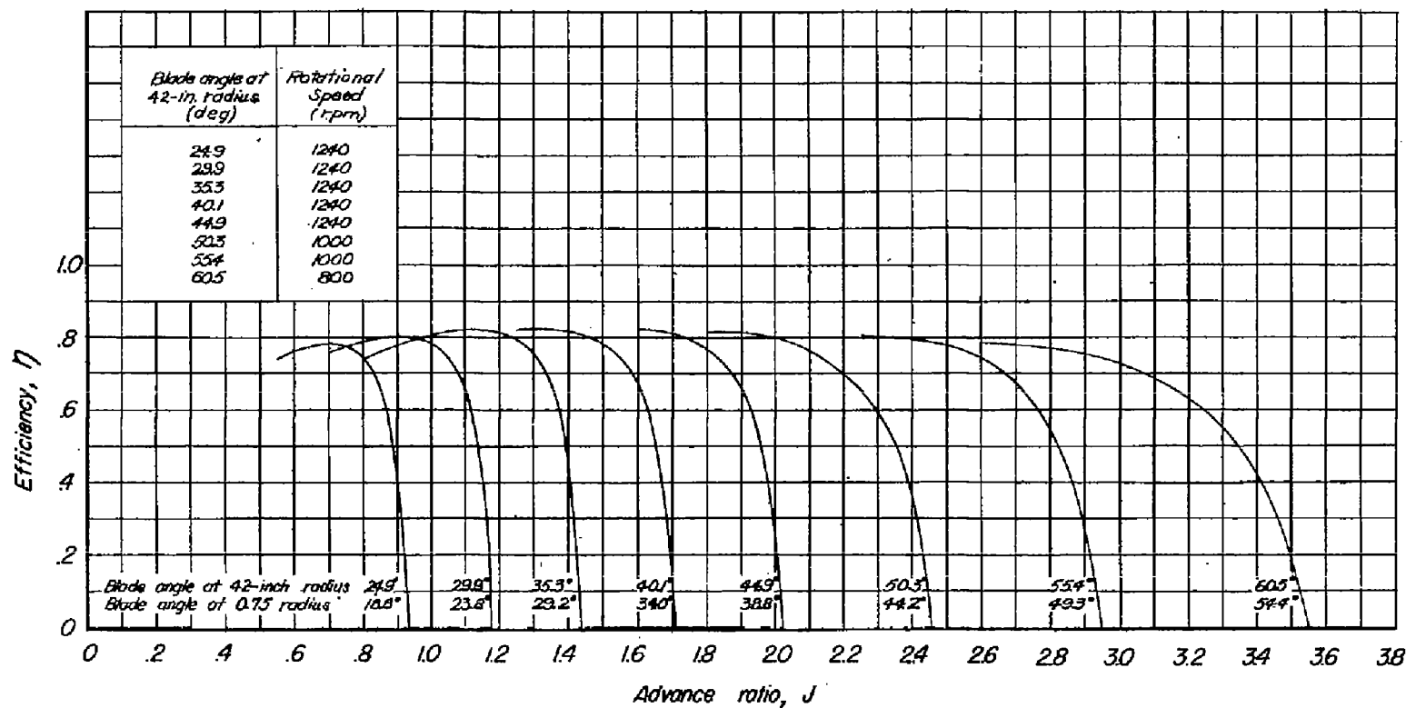
Figure 23.—Variation of propeller efficiency with advance ratio, Propeller with de-icing air flow.
